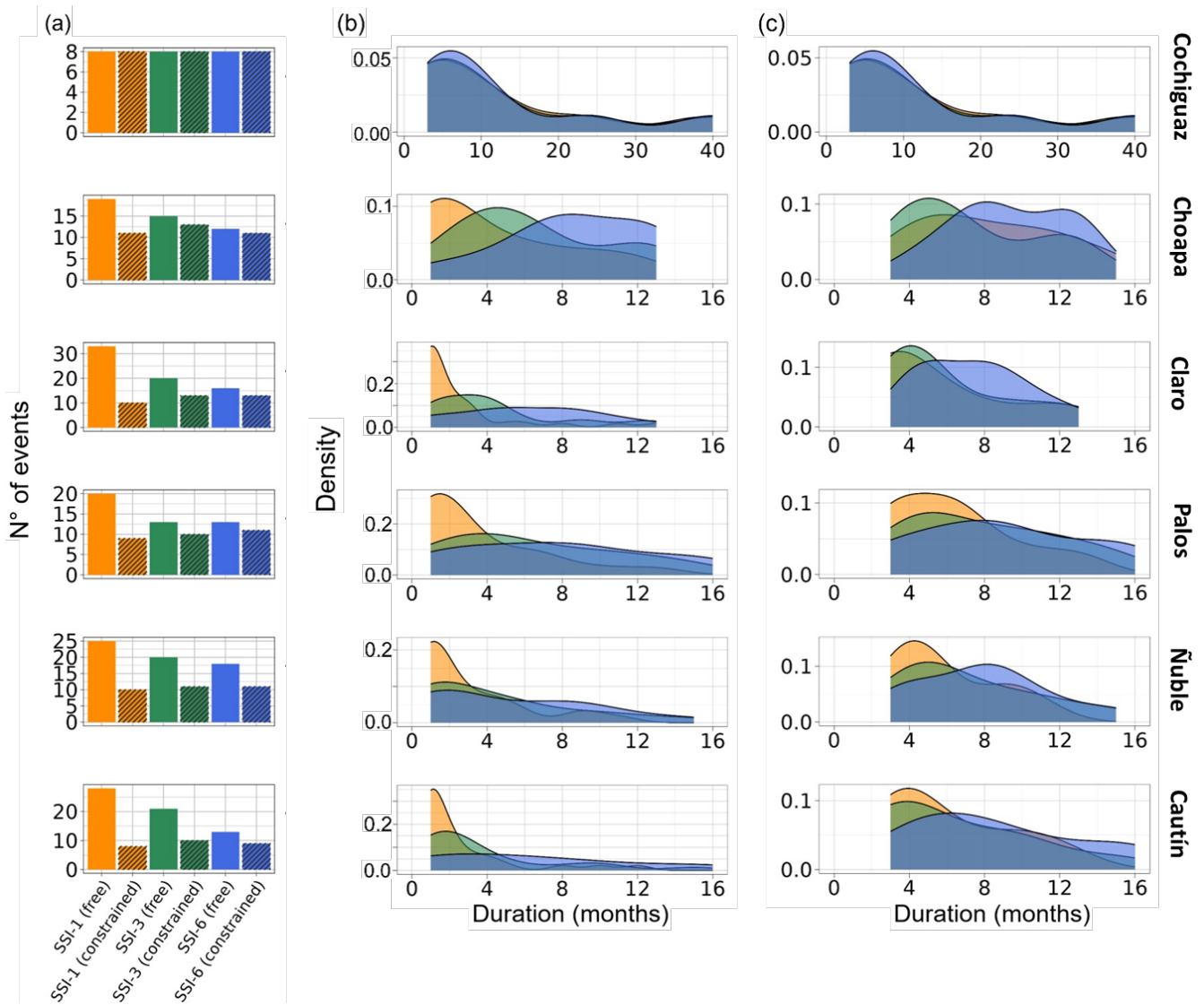
865 Figure 5. Effects of the choice of temporal scale (1, 3, and 6 months) in SSI calculations and duration restrictions on (a) the frequency and (b,c) duration of hydrological droughts detected between the water years 1983/84-2019/20. Probability distributions of drought durations are displayed for the cases (b) no restrictions regarding the duration of droughts – i.e., it is possible to detect one-month events (“free”) –, and (c) minimum drought duration of three months (i.e., “constrained”) for event detection – i.e., SSI-n < -1 during at least three consecutive months. 870
