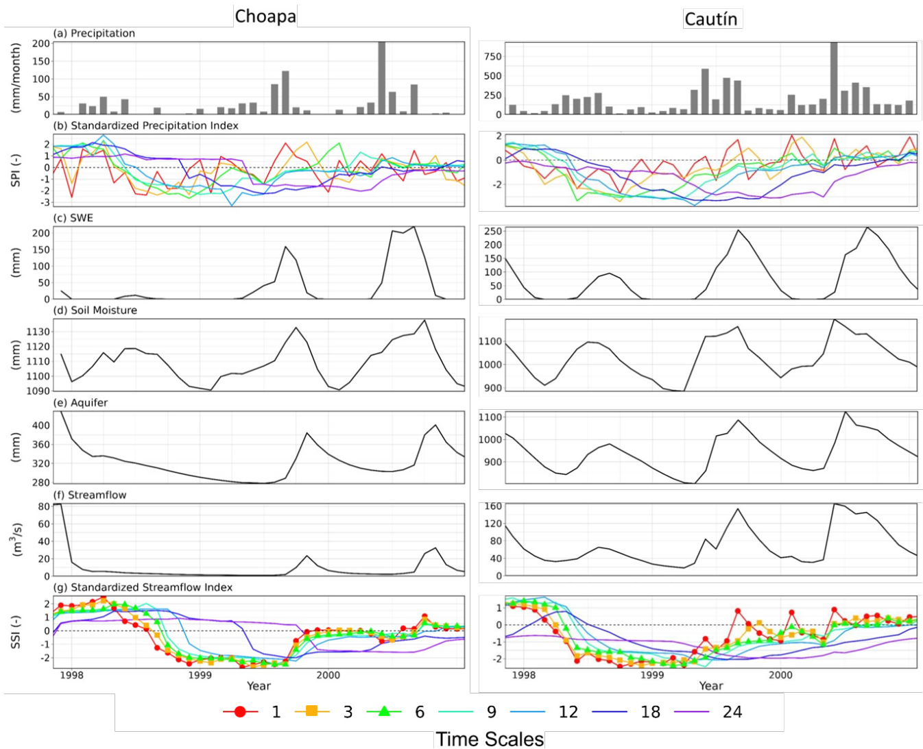
Figure 4. Monthly time series of (a) precipitation, (b) SPI-n, (c) SWE, (d) total soil moisture, (e) aquifer storage, (f) streamflow, and (g) SSI-n for the Choapa (snowmelt-driven, left) and Cautín (rainfall-driven, right) River basins. Monthly precipitation and SPI are obtained from the CR2MET meteorological product, whereas the remaining variables are obtained from SUMMA model simulations during January/1998-December/2000. SPI-n and SSI-n are displayed for time scales n = 1, 3, 6, 9, 12, 18, and 24 months. Time scales of 1, 3 and 6 months for the SSI are highlighted with circles, squares and triangles, respectively, due to their widespread use.
