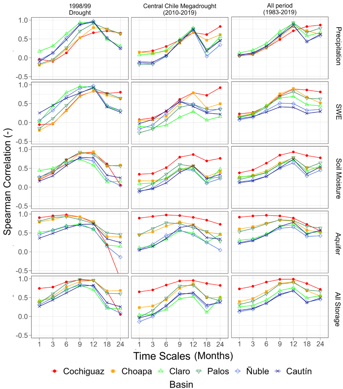
Figure 7. Spearman rank correlation coefficients between SSI-6 and temporally aggregated/averaged catchment-scale hydrological variables (rows) for three different periods: the October/1998-September/1999 drought event, (b) the central Chile megadrought (April/2010-March/2019), and (c) the entire analysis period (April/1983 - March/2020).
