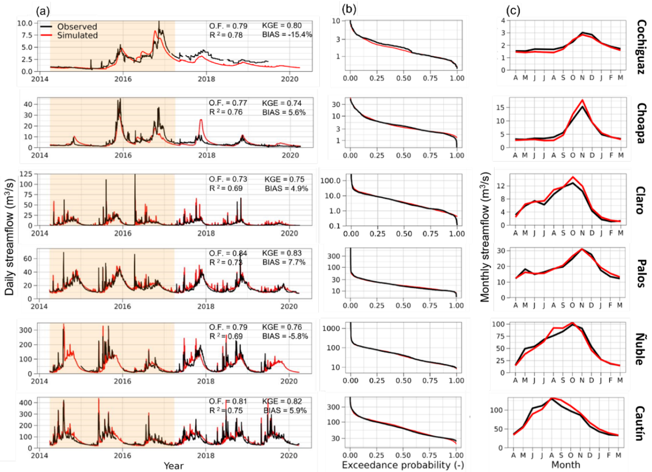
850 Figure 3. Comparison between simulated and observed streamflow for all basins in terms of (a) daily time series (April/2014 to March/2020), (b) daily flow duration curves (vertical logarithmic scale), and (c) mean monthly runoff. In (a) the shaded area represents part of the calibration (yellow) and evaluation (white) periods, and OF, R^2 , KGE and BIAS indicate the values for the objective function (Eq 3.1), coefficient of determination, Kling-Gupta Efficiency and percent bias over the evaluation period, respectively. The results in (b) and (c) correspond to the evaluation periods (April/2006 – March/2010 and April/2017 – March/2020) combined.
