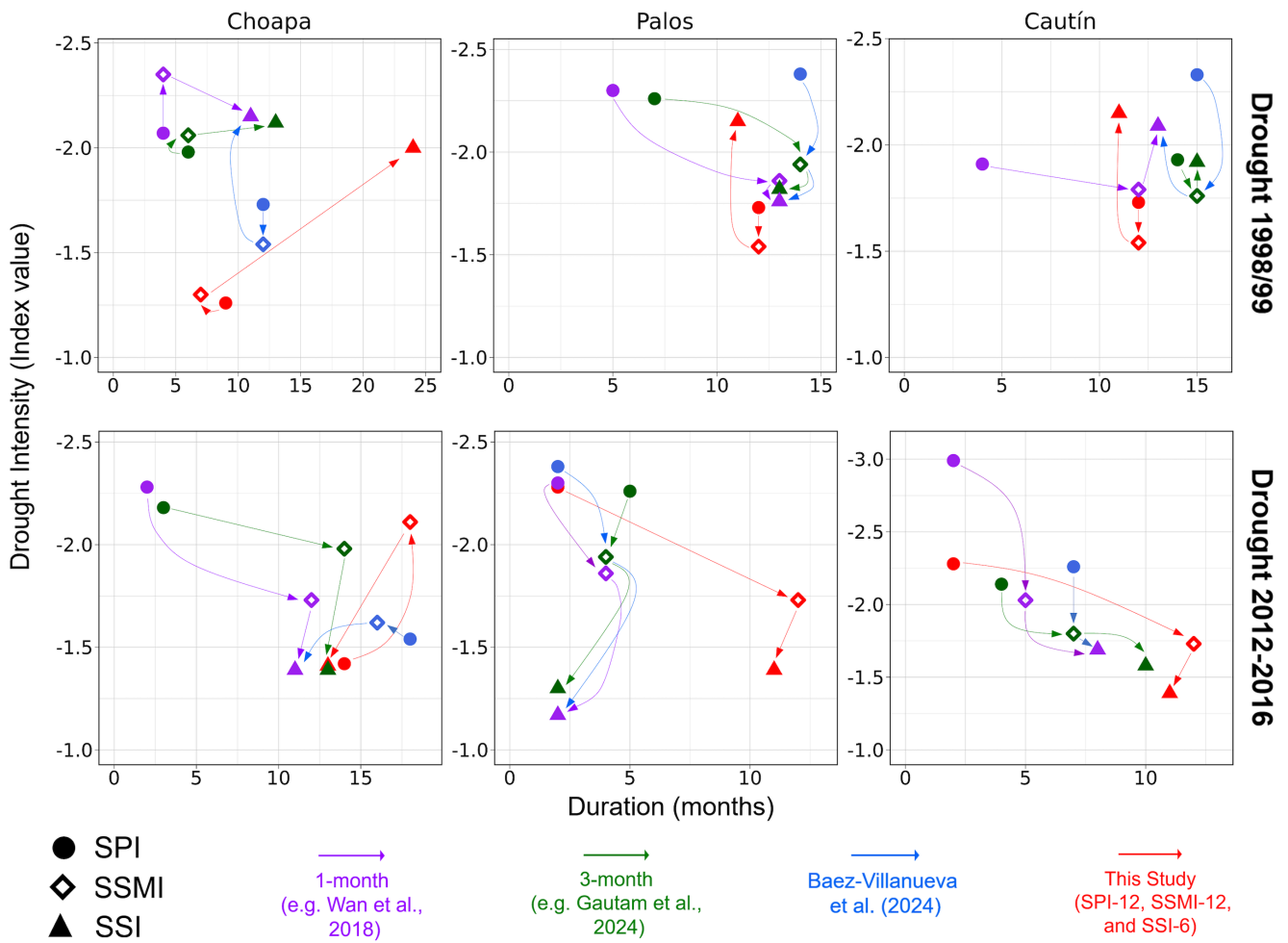
885 Figure 8. Propagation from meteorological (circles) to soil moisture (diamonds) and hydrological (triangles) droughts 886 for two selected drought events (1998/99 and 2012/-2016, displayed in different rows) and three basins with different 887 hydrological regimes: (a) Choapa (snowmelt-driven, left), (b) Palos (mixed regime, center) and Cautín (rainfall-driven, 888 right). The x-axis shows the duration in months, and the y-axis displays the intensity. The colors indicate trajectories 889 obtained with the temporal scales recommended by different studies.
