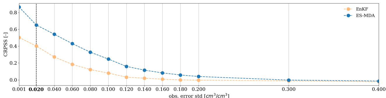
Figure 9. CRPSS sensitivity to standard deviation of observation error for the surface cell with EnKF and ES-MDA. The CRPSS is computed as an average over the whole time series and over the whole catchment. The bold label and vertical dashed line denote the nominal value of observation error used in this case study.
