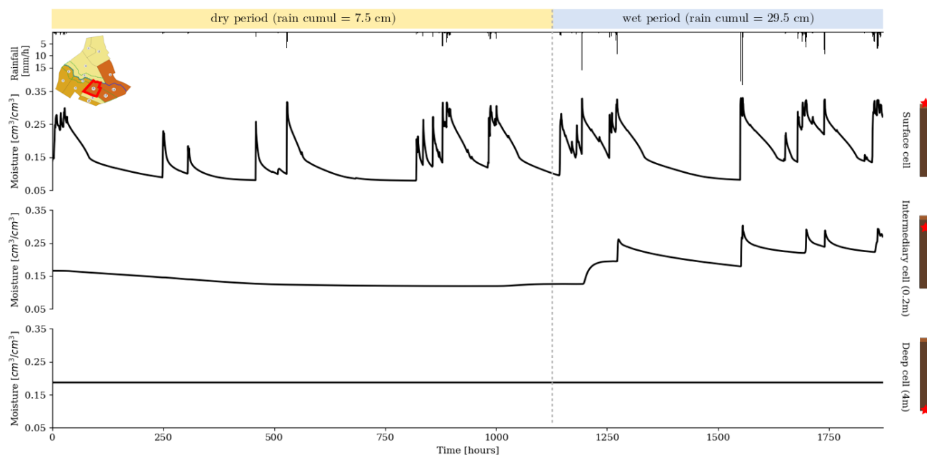
Figure 4. Soil moisture time series for the nominal simulation on plot 10 at surface (top), 0.2m depth (middle) and 4m depth (bottom). Rain forcings are shown in the top black histogram while the position of plot 10 in the catchment is denoted by a red line on the top-left pictogram. The soil composition of plot 10 is reminded in the soil columns depicted on the right with red stars showing the corresponding depths.
