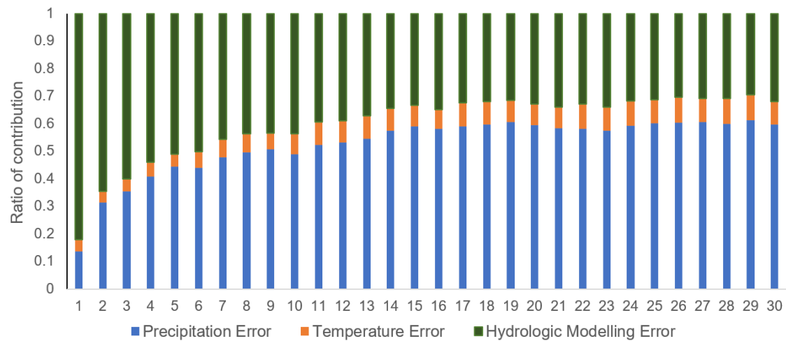
Figure 11. Contribution of precipitation forecast errors, temperature forecast errors, and hydrologic modelling errors to their combined error.
