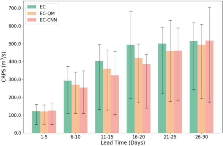
Figure 10. The CRPS of streamflow forecasts driven by the EC, EC-QM, and EC-CNN ensemble forecasts at different lead times during the test period. Error bar represents the 25 th -75 th percentile interval.
