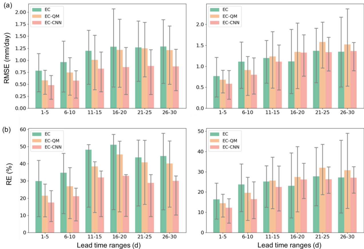
325 Figure 4. (a) RMSE and (b) RE of all rain events (left) and heavy rain events (right) for the ensemble means of EC, EC-QM and EC-CNN 5-day precipitation forecasts at lead times of 1-5 days, 6-10 days, 11-15 days, 16-20 days, 21-25 days, 26-30 days. Error bar represents the 25 th -75 th percentile interval.
