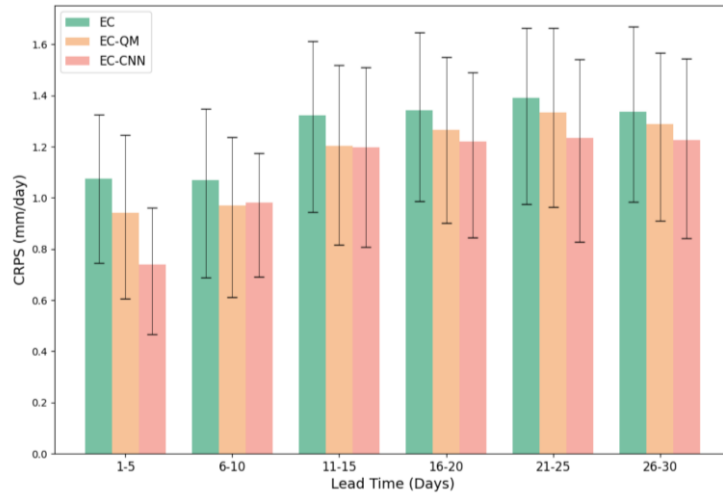
385 Figure 7. The CRPS of areal-averaged precipitation for the EC, EC-QM, and EC-CNN ensemble forecasts at different lead times during the test period. Error bar represents the 25 th -75 th percentile interval.
