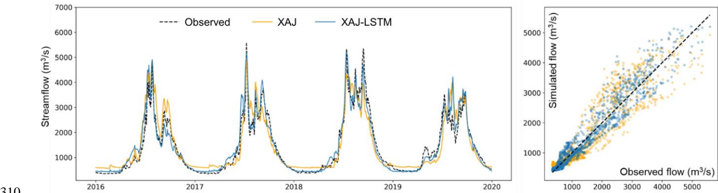
Figure 3. Streamflow validation of the XAJ model and the XAJ-LSTM hydrologic model.
