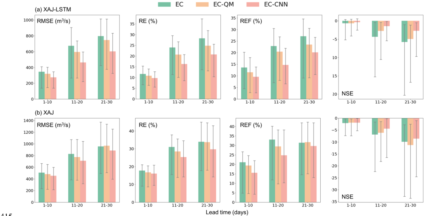
Figure 8. The RMSE, RE, REF, and NSE for the (a) XAJ-LSTM and (b) XAJ streamflow forecasts driven by the ensemble means of EC, EC-QM, and EC-CNN forecasts for lead times of 1-10 days, 11-20 days, and 21-30 days. Error bar represents the 25 th -75 th percentile interval.
