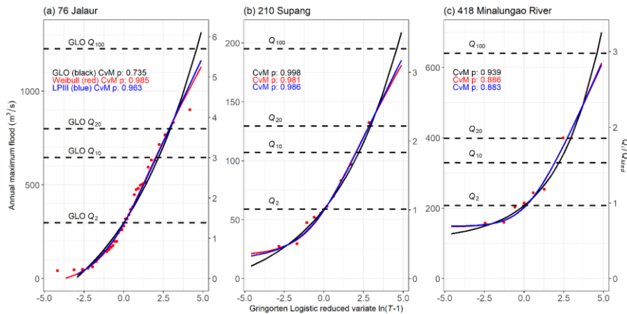
Figure 2: Selected annual maximum flood data and curve fits. Red points are data. Fitted curves are Generalised Logistic Distribution GLO (black), Weibull (red) and Log-Pearson III (blue). Cramér-von-Mises p-values shown. Left axes are flood magnitude ( \text{m}^3\text{s}^{-1} ) and right axes scale this by the median annual flood at each site. Values of 2,10,20 and 100 year recurrence interval floods are indicated, calculated using the GLO method. (A) Site 76, Jalaur (Lat: 11.1195; Long: 122.5386; Area 210 \text{km}^2 ; BRS_C data set; 37 years of data; best-fit curve: Weibull); (B) Site 210, Supang (Lat: 17.0073; Long: 120.9086; Area 56 \text{km}^2 ; Cagayan data set; 10 years; GLO); (C) Minalungao (or Sumacbao) River (Lat: 15.3430; Long: 121.0794; Area 309 \text{km}^2 ; SWS data set; 7 years; GLO).
