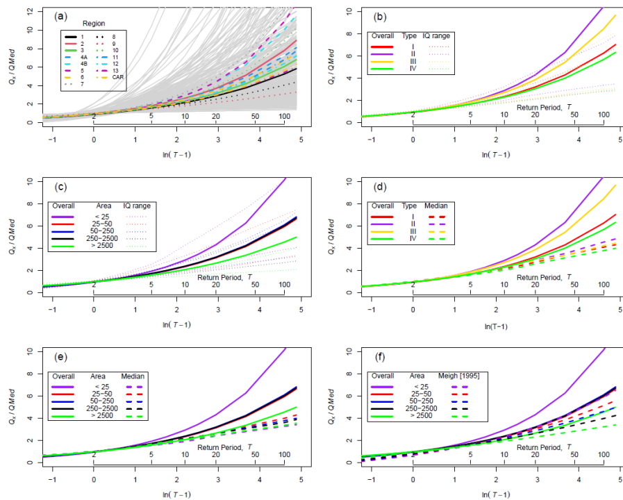
Figure 4 Dimensionless growth curves. (a) individual curves (GLO, Weibull or Log-Pearson Type III according to which produced the highest p-value in the Cramér-von Mises test) for 466 sites, overlain by pooled GLO curves for each region. (b) GLO curves fitted to data pooled from all sites in each climate type; IQ range lines are the inter-quartile (25 th and 75 th percentiles) of the curves for individual sites within each climate zone. (c) GLO curves fitted to all data within bins of catchment area, with inter-quartile ranges from individual sites shown. (d) Comparison of GLO curves fitted to all data from within each climate zone and the median value from curves fitted to individual sites within that zone. (e) Comparison of GLO curves fitted to all data for sites within each catchment area bin and the median value from individual sites within that area bin. (f) Overall GLO curves for each catchment area bin, and adjusted equivalent curves from Meigh (1995). Adjustment was necessary as Meigh (1995) used the mean annual flood as the index flood, rather than the median. See text for details.
