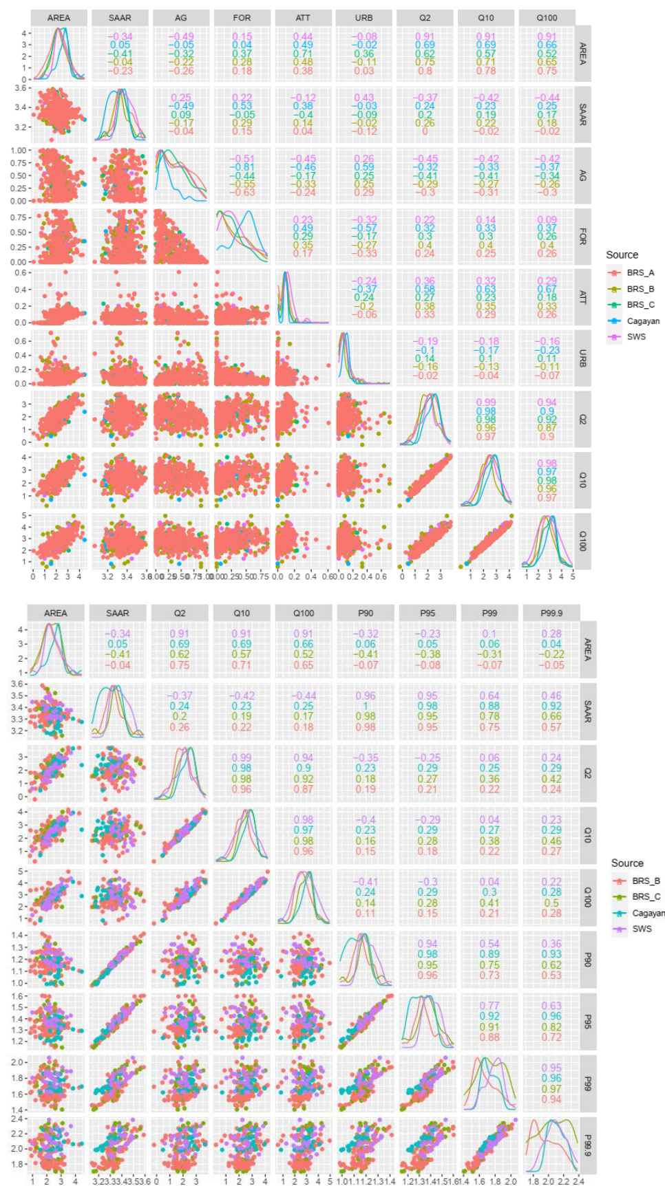
Figure S7. Cross-correlations between all variables used in the analysis. Note that several variables have been transformed prior to plotting, either Log10 (AREA, DPLBAR, SAAR, Q_{MED} , Q_2 , Q_{10} , Q_{100} ) or square root (ATT, RFSD, URB). See Table 4 for details. Points are colour coded by data source. Plots on the diagonal are probability
