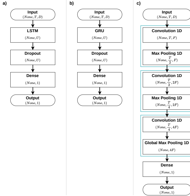
Figure 3. Schematic diagrams of the architectures of the three utilized utilised models: (a) Long Short-Term Memory (LSTM), (b) Gated Recurrent Unit (GRU), and (c) Convolutional Neural Network (CNN).
