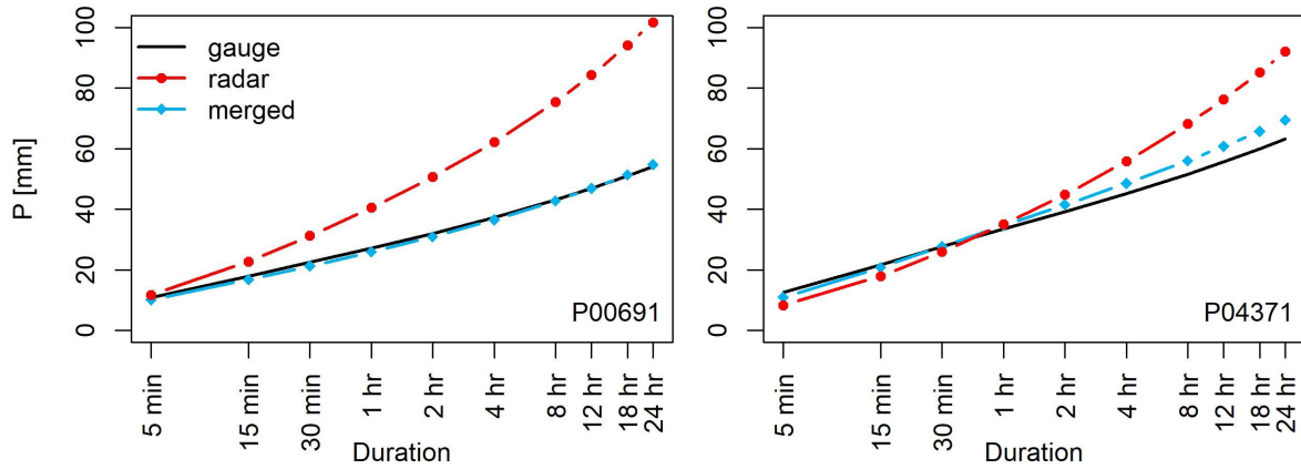
Figure 2. Example DDF curves of two validation stations P00691 and P04371, T = 20 yr. Curves from three sources are displayed: Ground rain gauges (black), radar data (red) and the product of conditional merging (blue)
