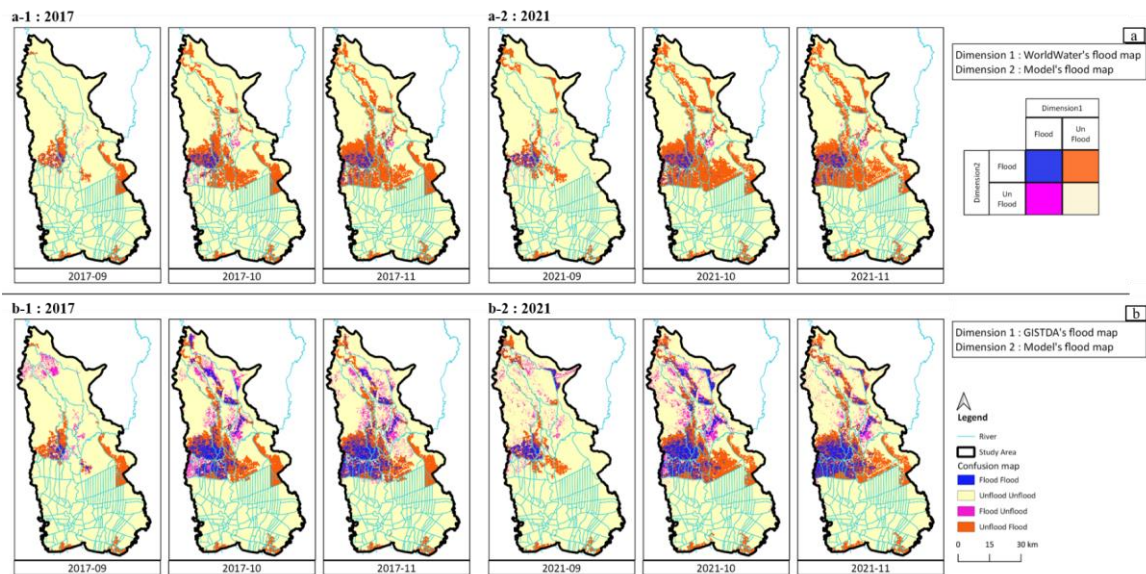
Figure 10: the contingency table of dimension 1 and dimension 2 flood maps on the spatial map: (a) Comparison between WorldWater and Model based on the merged LDD-JICA DEM, (a-1) in 2017 and (a-2) in 2021; (B) Comparison between GISTDA and Model based on the merged LDD-JICA DEM, (b-1) in 2017 and (b-2) in 2021.
