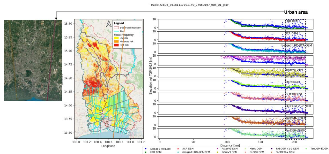
Figure A 12: The track-wise comparison of 10 DEM products with ICESat-2 ATL08 benchmark. © OpenStreetMap contributors 2015. Distributed under the Open Data Commons Open Database License (ODbL) v1.0. © Google Earth.
