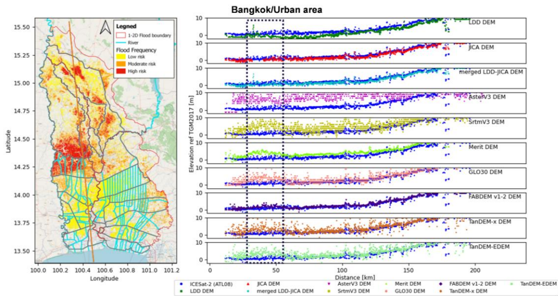
Figure 8: The track-wise comparison of 10 DEM products with ICESat-2 ATL08 benchmark. © OpenStreetMap contributors 2015. Distributed under the Open Data Commons Open Database License (ODbL) v1.0.
