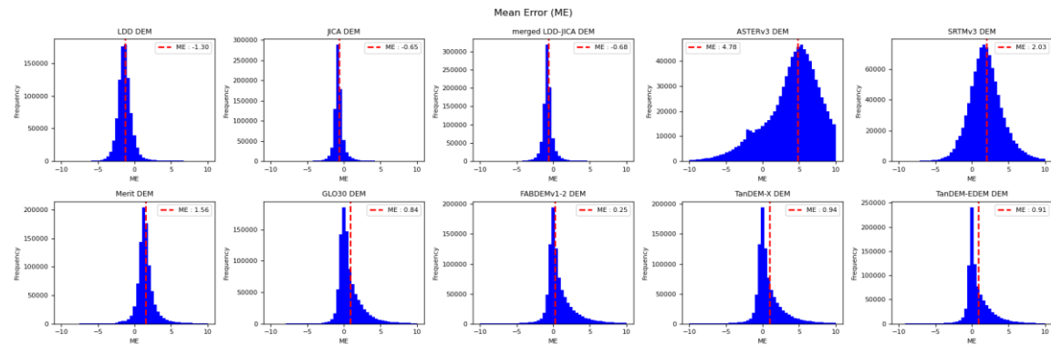
Figure 6: histogram distribution of the mean error (ME), comparing 10 DEM products against the ICESat-2 ATL08 benchmark.
