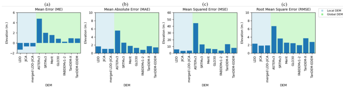
Figure 5: a bar chart of statistical metrics, comparing 10 DEM products against the ICESat-2 ATL08 benchmark, including (a) mean error (ME), (b) mean absolute error (MAE), (c) mean squared error (MSE), and (d) root mean square error (RMSE). The resulting averages are computed across the datasets in study area.
