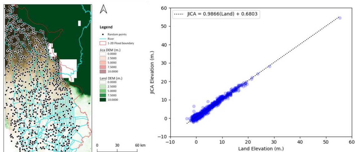
Figure A-4: the merged LDD-JICA-DEM's processing
