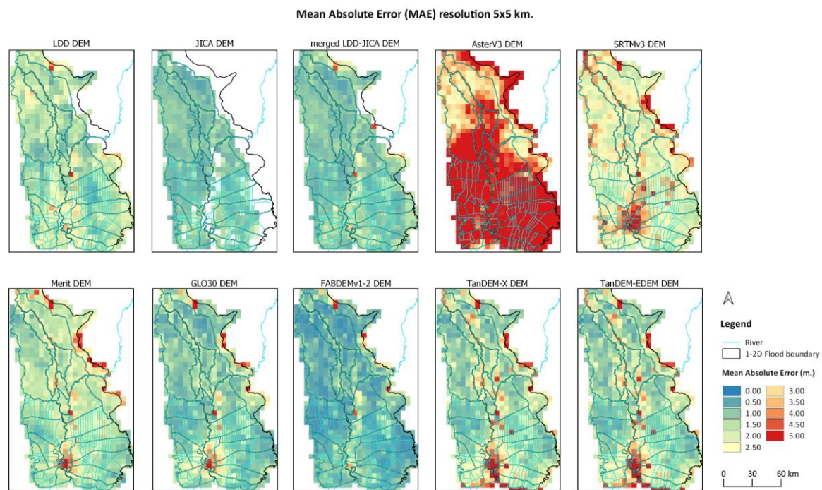
Figure A 10: The mean error (MAE) spatial grid comparison of 10 DEM products against the ICESat-2 ATL08 benchmark, with a resolution of 5x5 km.
