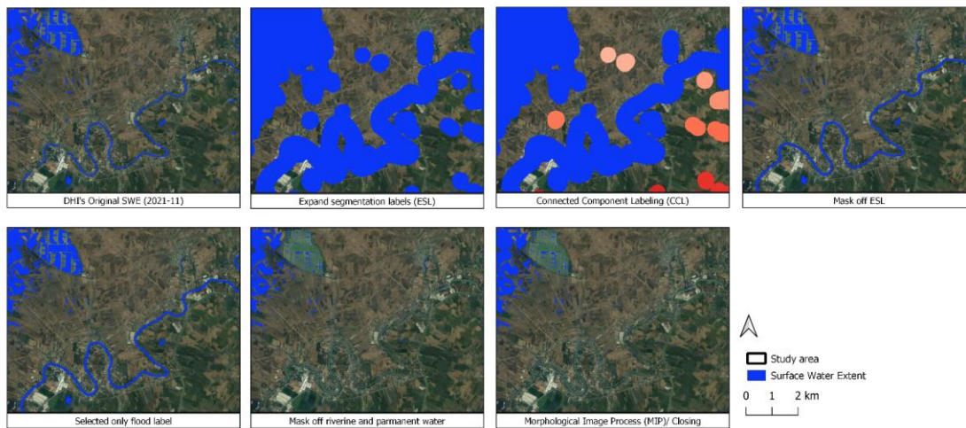
845 Figure A 5: Riverine flood classification processing. © Google Earth
