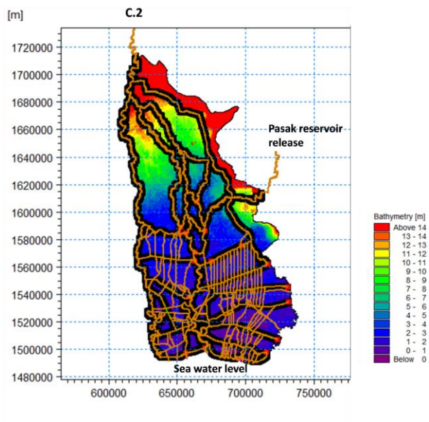
Figure A 1: 1D-2D Flood model
