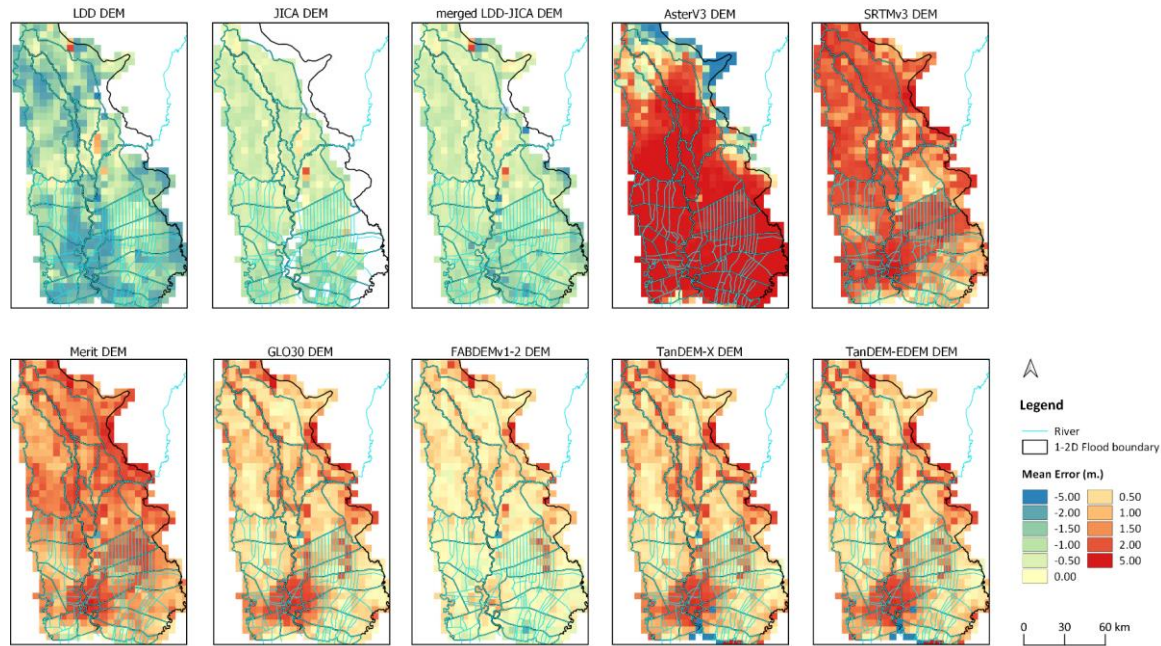
Figure A 9: The mean error (ME) spatial grid comparison of 10 DEM products against the ICESat-2 ATL08 benchmark, with a resolution of 5x5 km.
