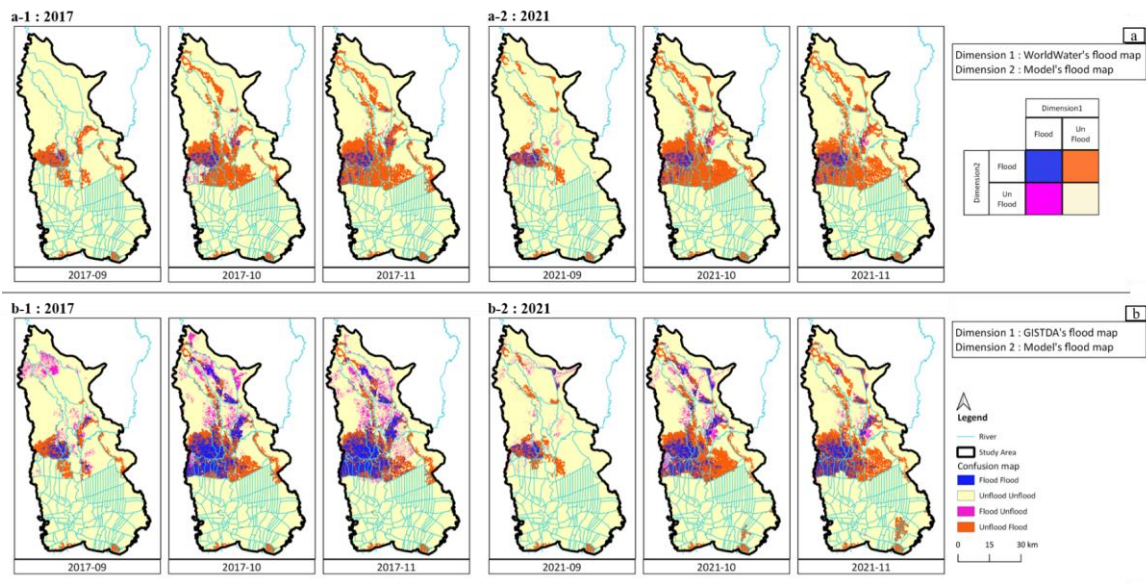
Figure 11: the contingency table of dimension 1 and dimension 2 flood maps on the spatial map: (a) Comparison between WorldWater and Model based on FABDEMv1-2 DEM, (a-1) in 2017 and (a-2) in 2021; (b) Comparison between GISTDA and Model based on FABDEMv1-2 DEM, (b-1) in 2017 and (b-2) in 2021.
