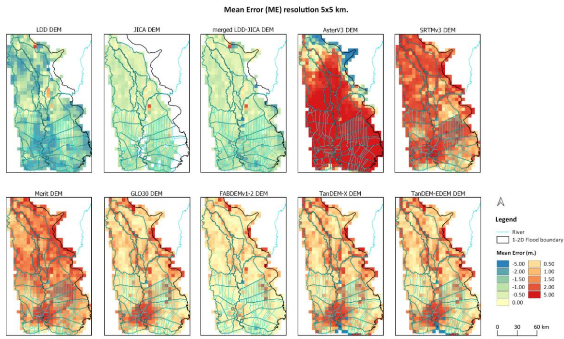
Figure 7: the mean error (ME) spatial grid comparison of 10 DEM products against the ICESat-2 ATL08 benchmark, with a resolution of 5x5 km.
