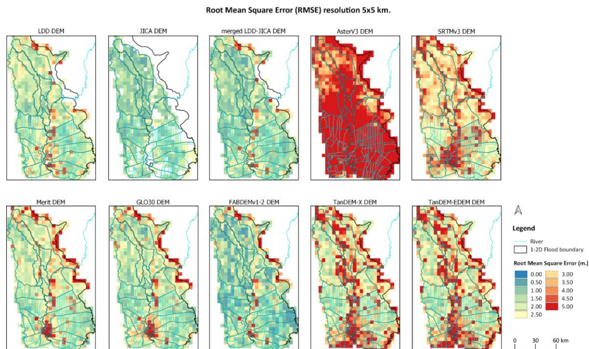
860 Figure A 11: The mean error (RMSE) spatial grid comparison of 10 DEM products against the ICESat-2 ATL08 benchmark, with a resolution of 5x5 km.
