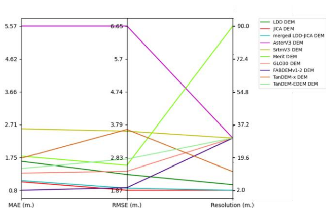
Figure 9: The parallel plot of 10 DEMs evaluation with the ICESat-2 ATL08 benchmark.
