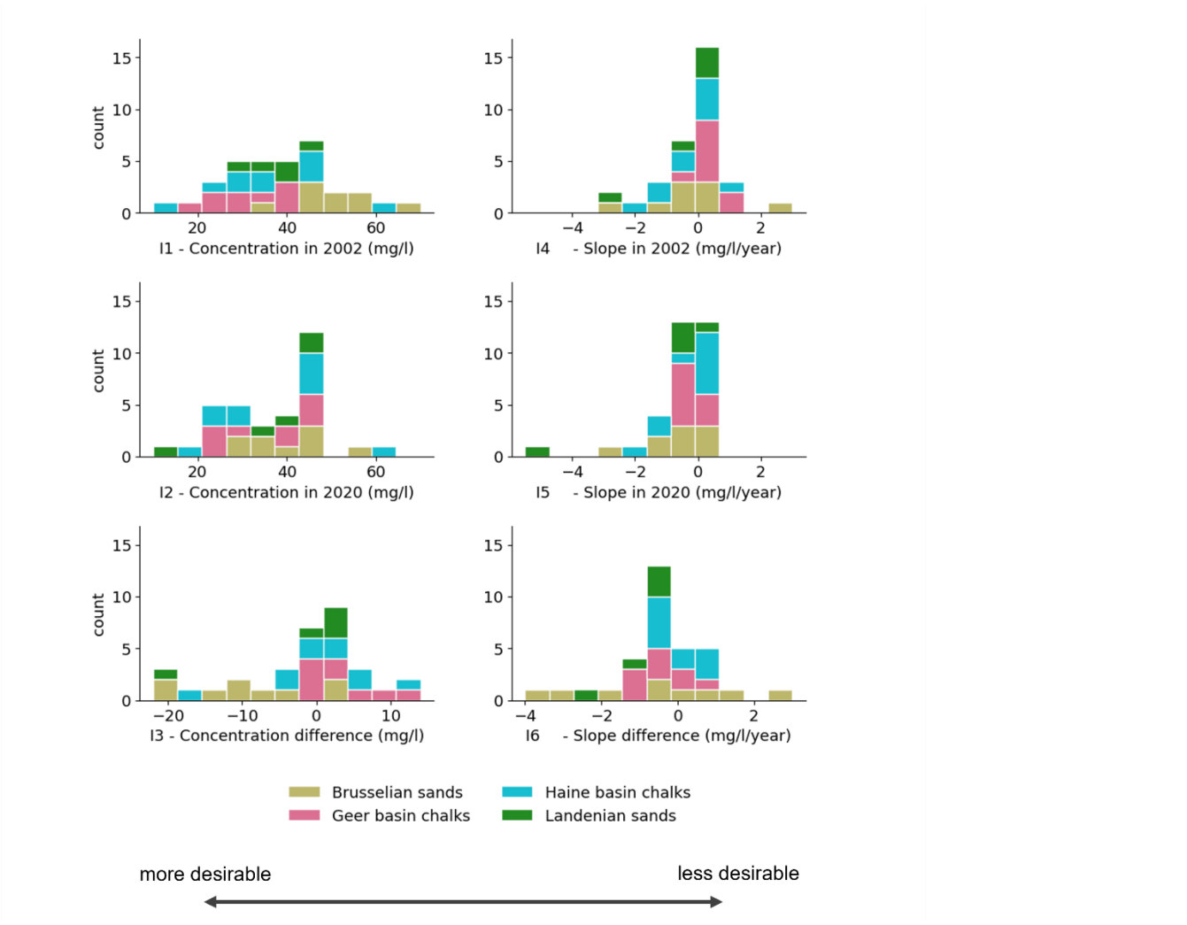
Figure 4. Histograms of the six pollution indicators. The black arrow at the bottom indicates that, for each indicator, lower values are more desirable than higher values, as this entail lower nitrate concentrations, decreasing trends and a decrease in concentration from 2002 to 2020.
