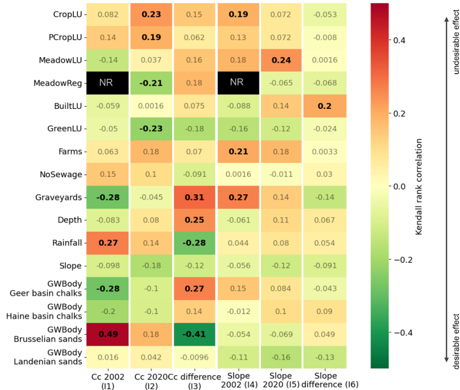
Figure 5 Heatmap of the Kendall rank correlation coefficients between the explanatory variables and the six pollution indicators. Coefficients in bold indicate a significant relationship (p-value<0.1) NR: not relevant. The black arrow on the right indicates that low correlation is more desirable than high correlation, as low correlation entails that high values of the explanatory variables are correlated to low values for the six pollution indicators and vice versa.
