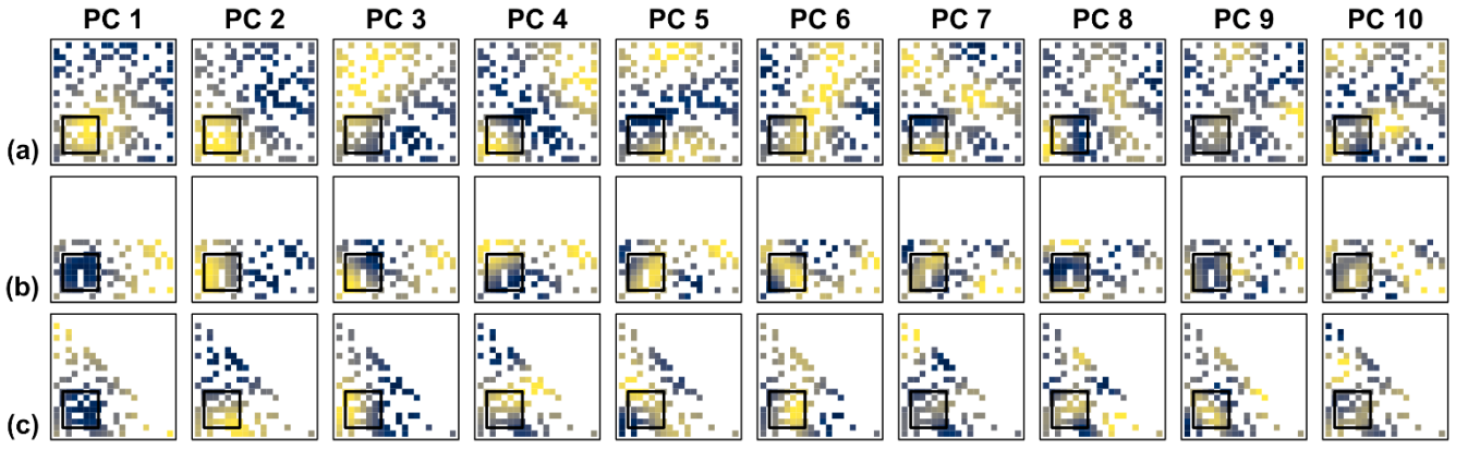
490 Figure 11 DD reference patterns as in Figure 8 but for a random selection of only 40 % from the cells within the three geometric domain boundaries of Figure 6. The sampling probability within the small square in the lower left was three times higher than in the rest of the domain (spatially heterogeneous case).
