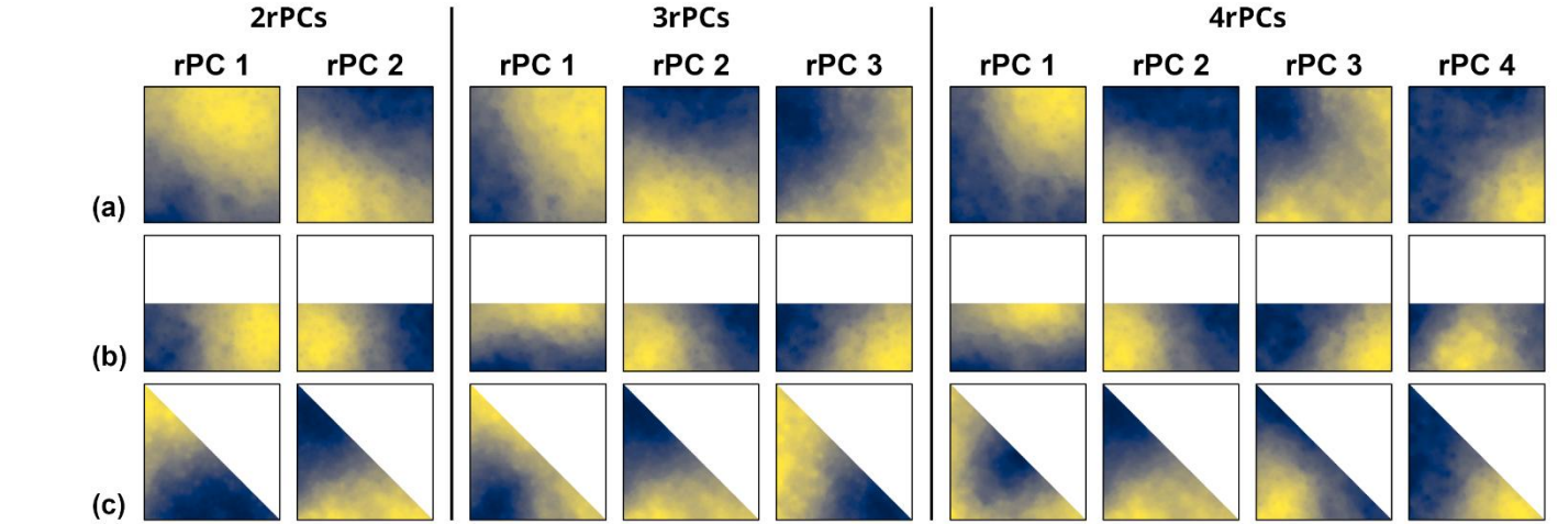
Figure 17 Leading varimax rotated spatial PC patterns from the PCAs of the precipitation data with the square, rectangular and triangular domain (Figure 16). The rotation was performed with the first two PCs (2rPCs), the first three PCs (3rPCs) or the first four PCs (4rPCs).
