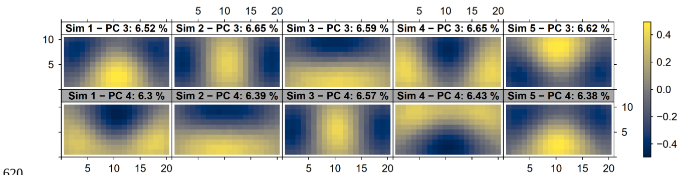
620 Figure 15 Spatial patterns of the degenerated PCs 3 and 4 from five distinct data sets, each simulated with rectangular domain ( 20 \times 10 cells), isotropic exponentially decaying spatial autocorrelation of correlation length 10 cells and time series length 10 000. Identical properties were used to simulate the ensembles from Figure 7b, Figure 8b and Figure 9b. The spatial patterns that belong to the same data set are plotted above each other with PC 3 on the top (white panel titles) and PC 4 on the bottom (grey panel titles). The index of the simulated data set and the fraction of assigned variance is given in the panel titles. 625
