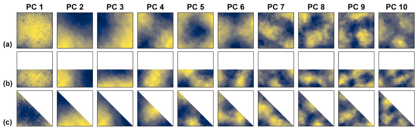
655 Figure 16 Overview of the leading ten spatial PC patterns from the PCAs of the precipitation data with the square, rectangular and triangular domain. The location of the square domain is marked in Figure 3. The two other domains are fit in the square domain.
