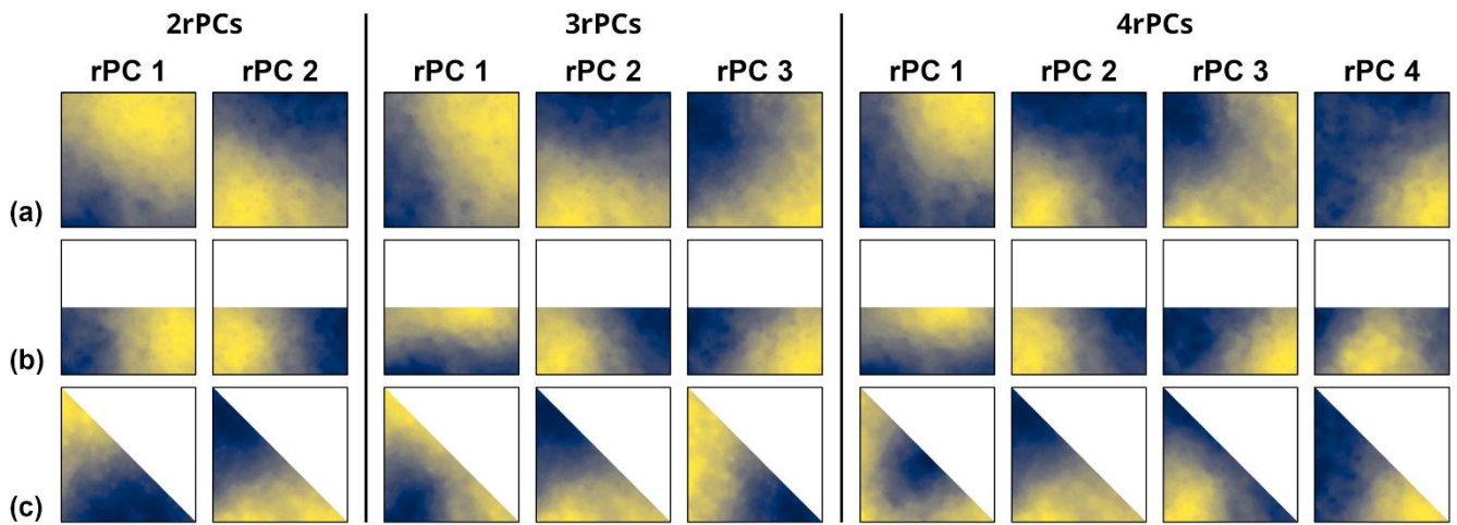
Figure 17 Leading varimax rotated spatial PC patterns from the PCAs of the precipitation data with the square, rectangular and triangular domain (Figure 16). The rotation was performed with the first two PCs (2rPCs), the first three PCs (3rPCs) or the first four PCs (4rPCs).
