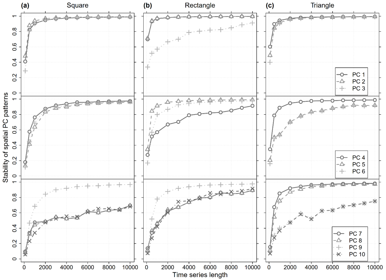
Figure S31 Stability of the spatial PC patterns as in Figure 7Figure-4 but for the patterns of the heterogeneous subsampling variant (Figure 11Figure-9).
