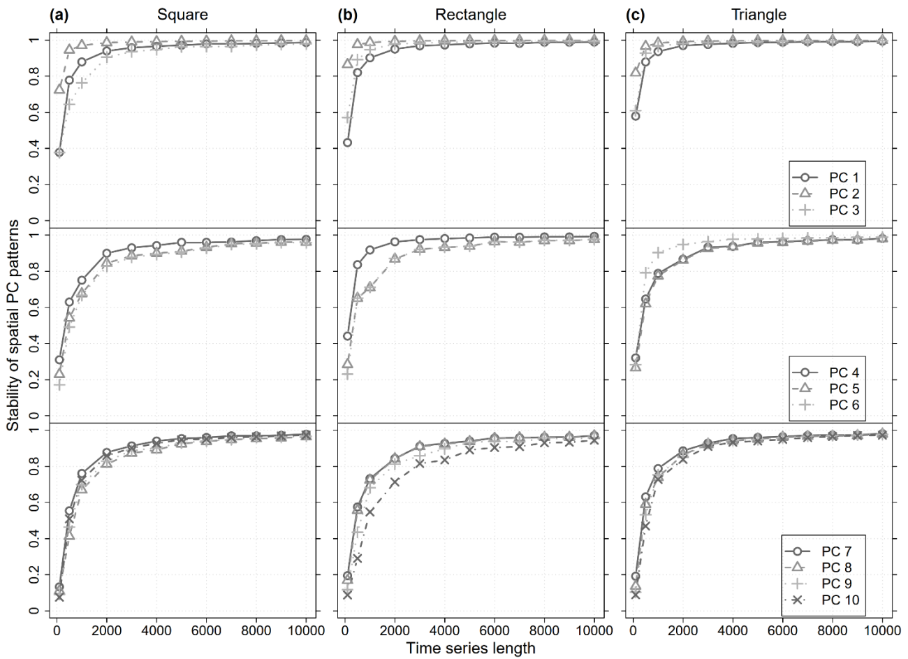
Figure S106 Stability of the spatial PC patterns from the anisotropic example in Figure S9 for the domain shapes (a) square, (b) rectangle and (c) triangle, all for different time series length of the simulated data. For each time series length 100 data sets were simulated with identical parametrisation. Each simulated data set was analysed separately with PCA. Symbols depict the mean R^2 of the correlation between the spatial patterns of all PCs with identical rank derived from the respective ensemble of all 100 simulated data sets. The legends in (c) apply also to (a) and (b) of the respective row.
