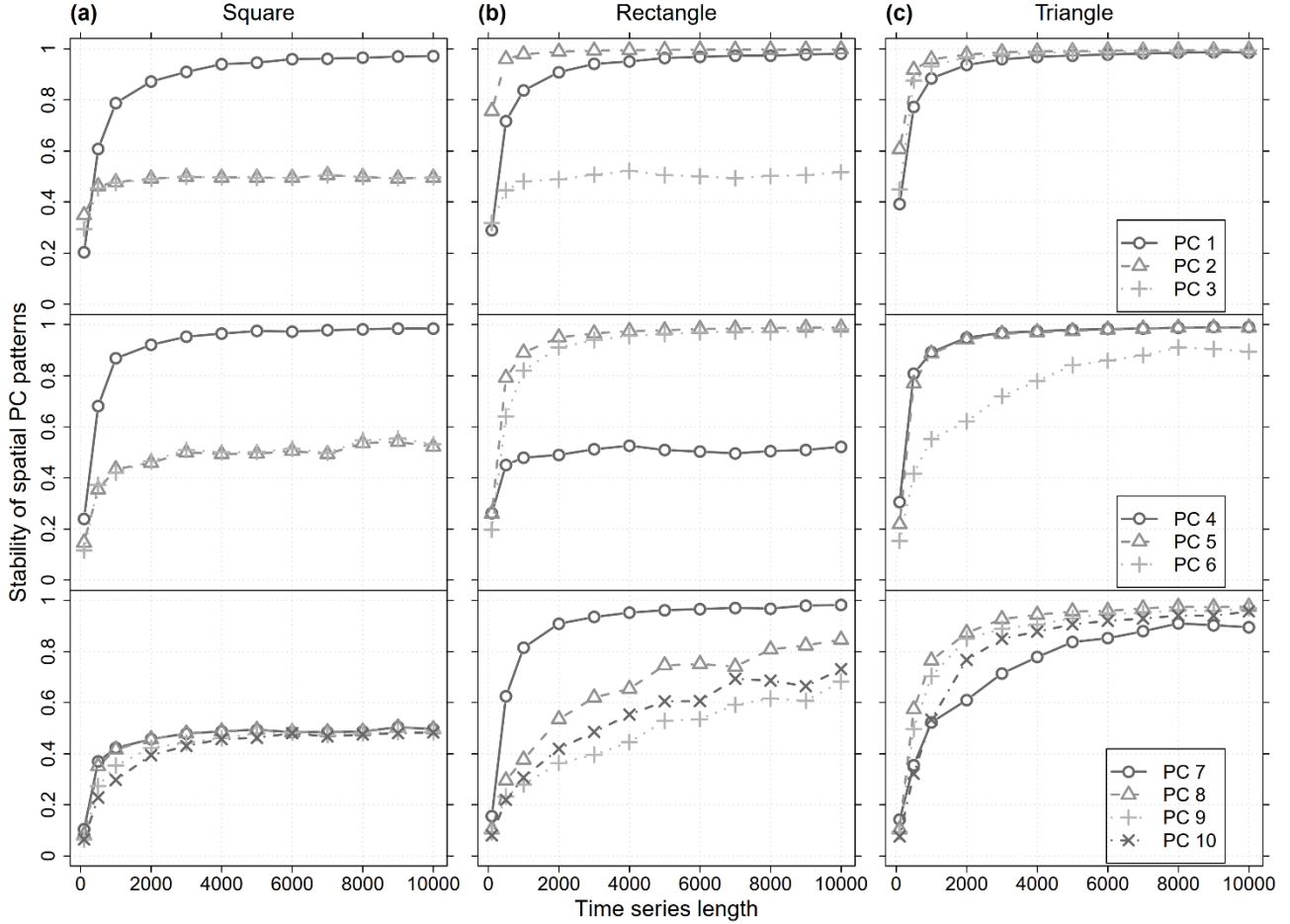
Figure 74 Stability of the spatial patterns from the leading ten PCs in relation to the time series length of the simulated data within the (a) square, (b) rectangular and (c) triangular domain boundaries of Figure 63Figure-3 . All cells within the boundaries were used. For each domain the results from 12 data set ensembles are shown. Each ensemble consists of 100 data sets simulated with
