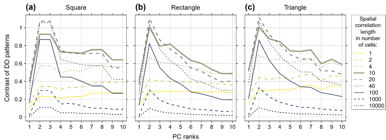
Figure 14 As in Figure 13 Figure-11 but for the contrasts of the DD patterns.
