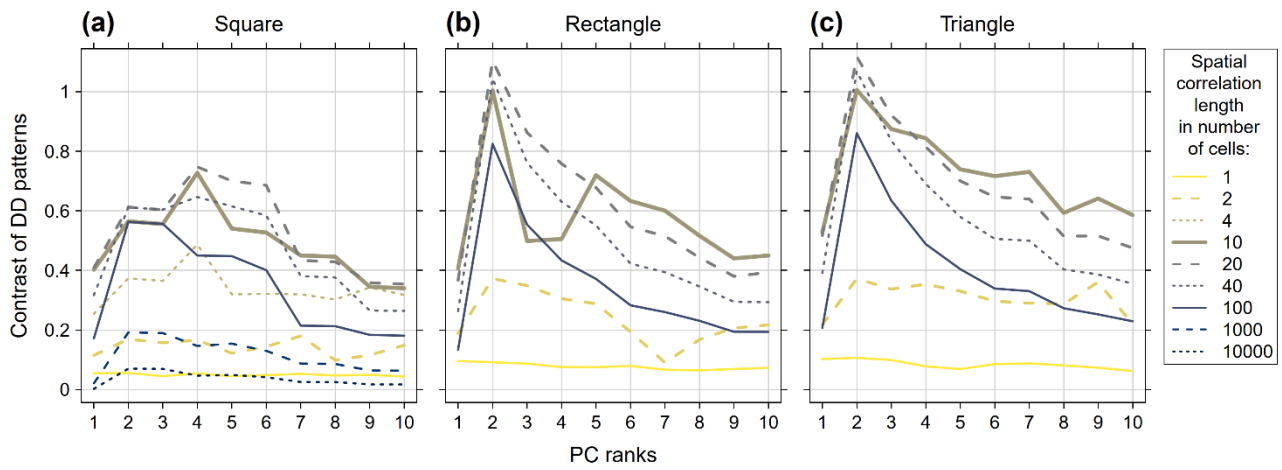
Figure S53 Contrast of the ten leading DD patterns PCs modelled with the stochastic DD reference method using an isotropic exponential covariance model, nine different spatial correlation lengths and the domain boundaries (a) square, (b) rectangle and (c) triangle from Figure 6 Figure 3 . All cells within the boundaries were used. For each correlation length, the DD reference patterns were estimated from ensembles with 100 simulated data sets, each with time series length 10 000.
