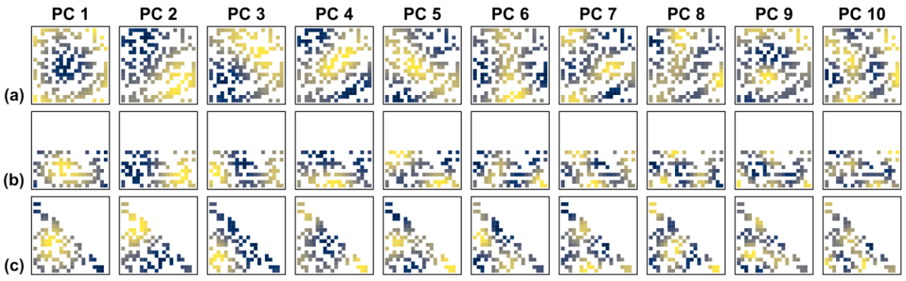
550 Figure 108 DD reference patterns as in Figure 8Figure-5 but for a random selection of only 40 % from the cells within the three geometric domain boundaries of Figure 6Figure-3. The sampling probability was homogeneous across the domain (spatially homogeneous case).
