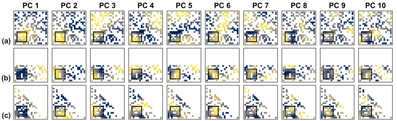
555 Figure 119 DD reference patterns as in Figure 8Figure-5 but for a random selection of only 40 % from the cells within the three geometric domain boundaries of Figure 6Figure-3. The sampling probability within the small square in the lower left was three times higher than in the rest of the domain (spatially heterogeneous case).
