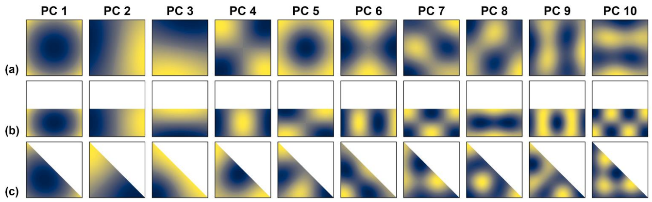
Figure S7 Overview of the ten leading DD reference patterns for the spatial PC patterns of the precipitation data sets from Figure 16. The patterns were estimated with the analytic method with an isotropic spherical covariance model and a spatial correlation length of 770 km. For comparison: The mean range of the spherical sample variograms from all 360 monthly 200 km \times 200 km square precipitation raster (Figure 3) was 824 km. The sample variograms were estimated with the R package "gstat" using the default settings and the cut off length set to the side length of the square.
