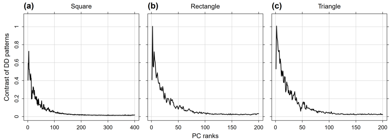
Figure S42 Contrast of all DD patterns modelled with the analytic DD reference method using an isotropic exponential covariance model, spatial correlation length of 10 cells and the domain boundaries (a) square, (b) rectangle and (c) triangle from Figure 6Figure-3. All cells within the boundaries were used. Note that the number of PCs depends on the number of analysed series, which equals here the number of cells in the domains.
