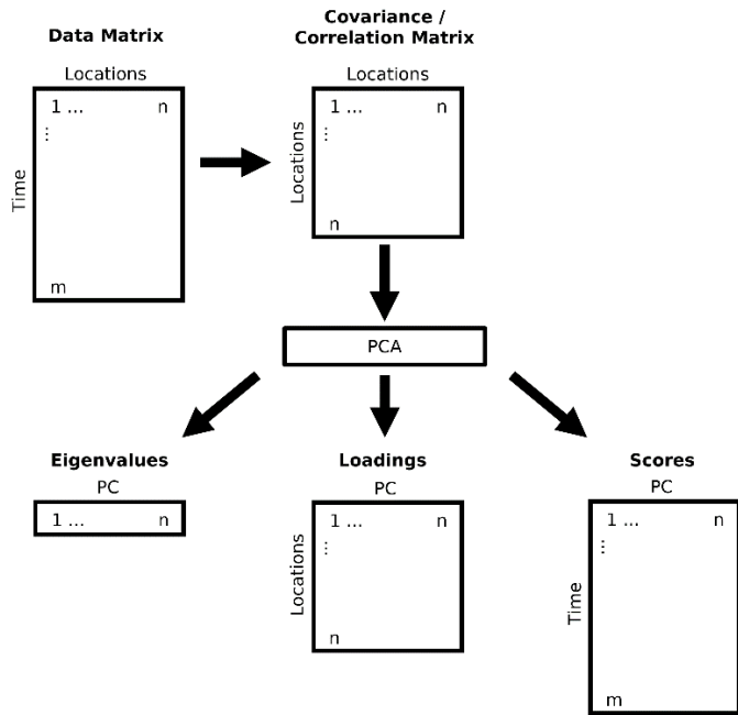
Figure S1 S-mode PCA, adapted after Fig. 9 in Richman (1986). n: number of locations, m: number of time steps. The eigenvalues define the explained variance, the loadings the unscaled spatial PC patterns and the scores the temporal PC patterns.
