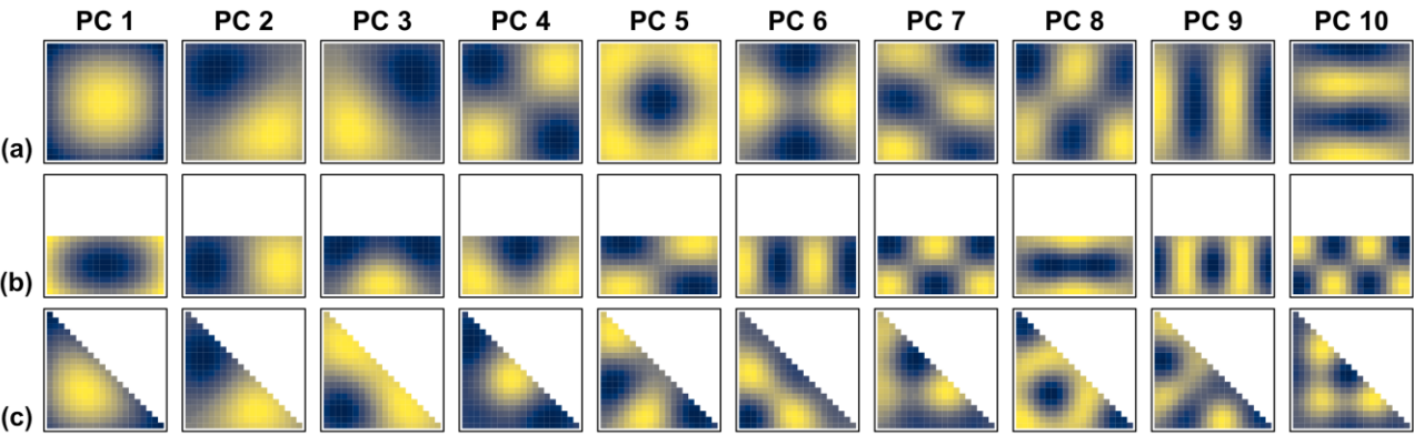
485 Figure 95 Overview of the leading ten mean spatial PC patterns (DD reference patterns), estimated with the stochastic method from the data set ensembles with time series length 10 000 shown in Figure 7Figure-4 . Instead of the +/- schemes used by Buell (1975) (Figure 1) we use colour gradients to picture the spatial patterns.
