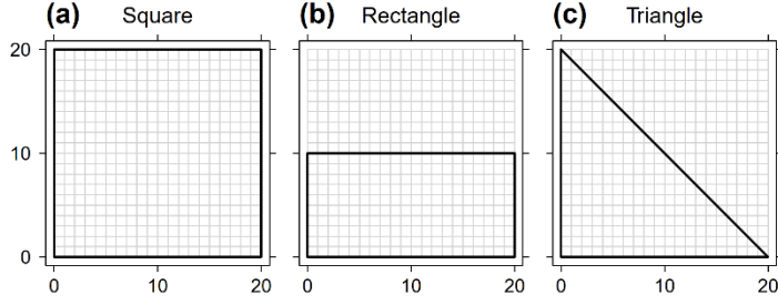
Figure 63 (a) Square, (b) rectangular and (c) triangular domain boundaries on the 20 \times 20 grid. The grid cells represent locations from a data set.
