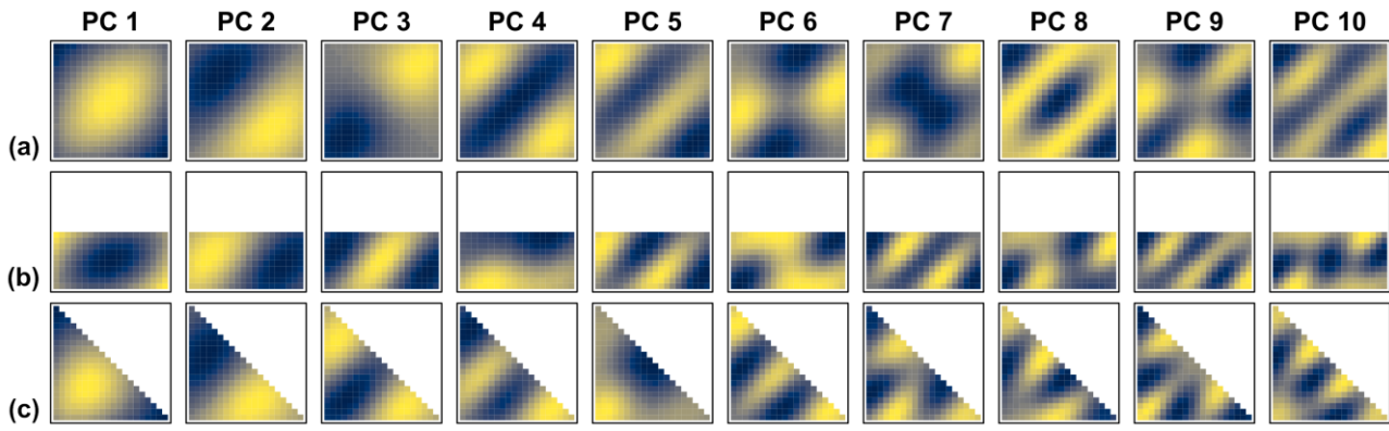
Figure S95 Anisotropic example: Overview of the ten leading DD reference patterns for anisotropic spatial correlation with a direction (angle) of 45^\circ clockwise from North and an anisotropy ratio of 2 with the longer spatial correlation length being 10 cells, and the domain boundaries (a) square, (b) rectangle and (c) triangle from Figure 6. All cells within the boundaries were used. The patterns were estimated with the stochastic method from ensembles with 100 data sets, each with time series length 10 000.
