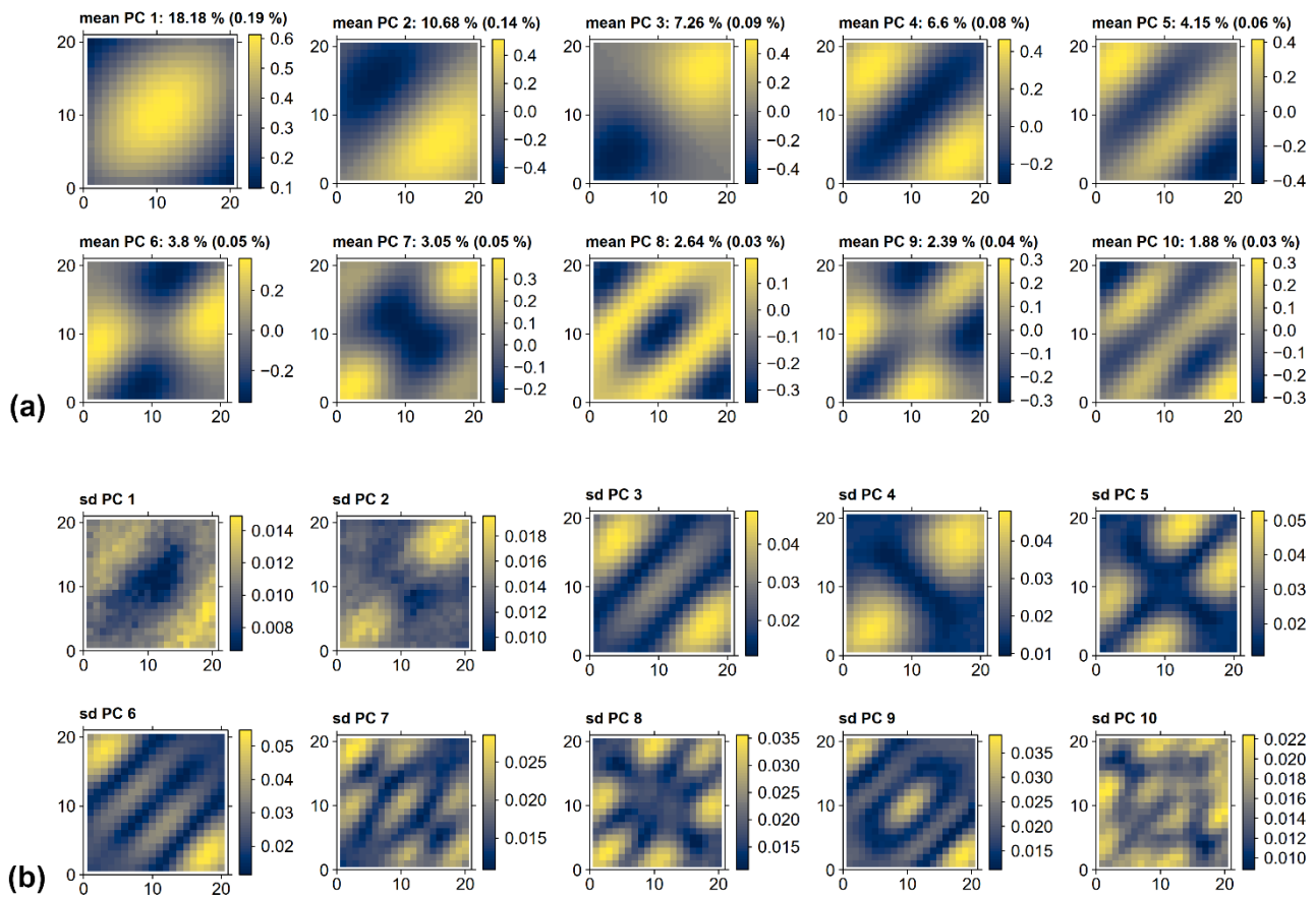
Figure S117 Detail plot of mean (a) and standard deviation (b) of the spatial patterns from the leading ten PCs of the data set ensemble with the square domain shown in Figure S9Figure S5a . The mean (and standard deviation) of the fractions of variance assigned to the respective PCs from the 100 PCAs of the ensemble is given in the panel titles of (a).
