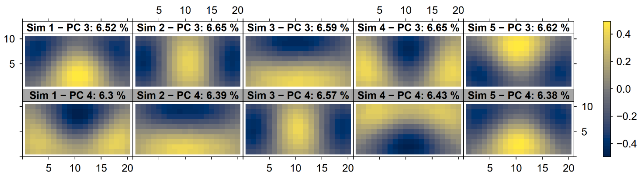
Figure 1513 Spatial patterns of the degenerated PCs 3 and 4 from five distinct data sets, each simulated with rectangular domain ( 20 \times 10 cells), isotropic exponentially decaying spatial autocorrelation of correlation length 10 cells and time series length 10 000. Identical properties were used to simulate the ensembles from Figure 7Figure 4b, Figure 8Figure 5b and Figure 9Figure 6b. The spatial patterns that belong to the same data set are plotted above each other with PC 3 on the top (white panel titles) and PC 4 on the bottom (grey panel titles). The index of the simulated data set and the fraction of assigned variance is given in the panel titles.
