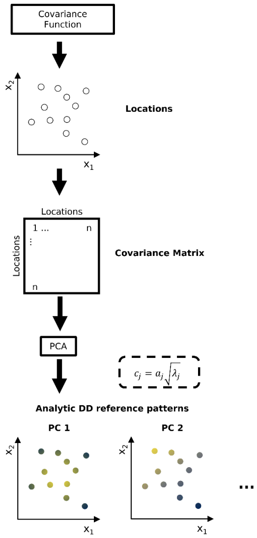
Figure 5 Analytic DD reference method.
