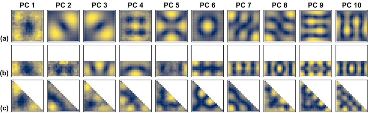
490 Figure 96 As in Figure 8Figure-5 but for the standard deviation patterns (uncertainty estimation of the stochastic DD reference patterns). From blue to yellow the colour gradients depict increasing uncertainty.
