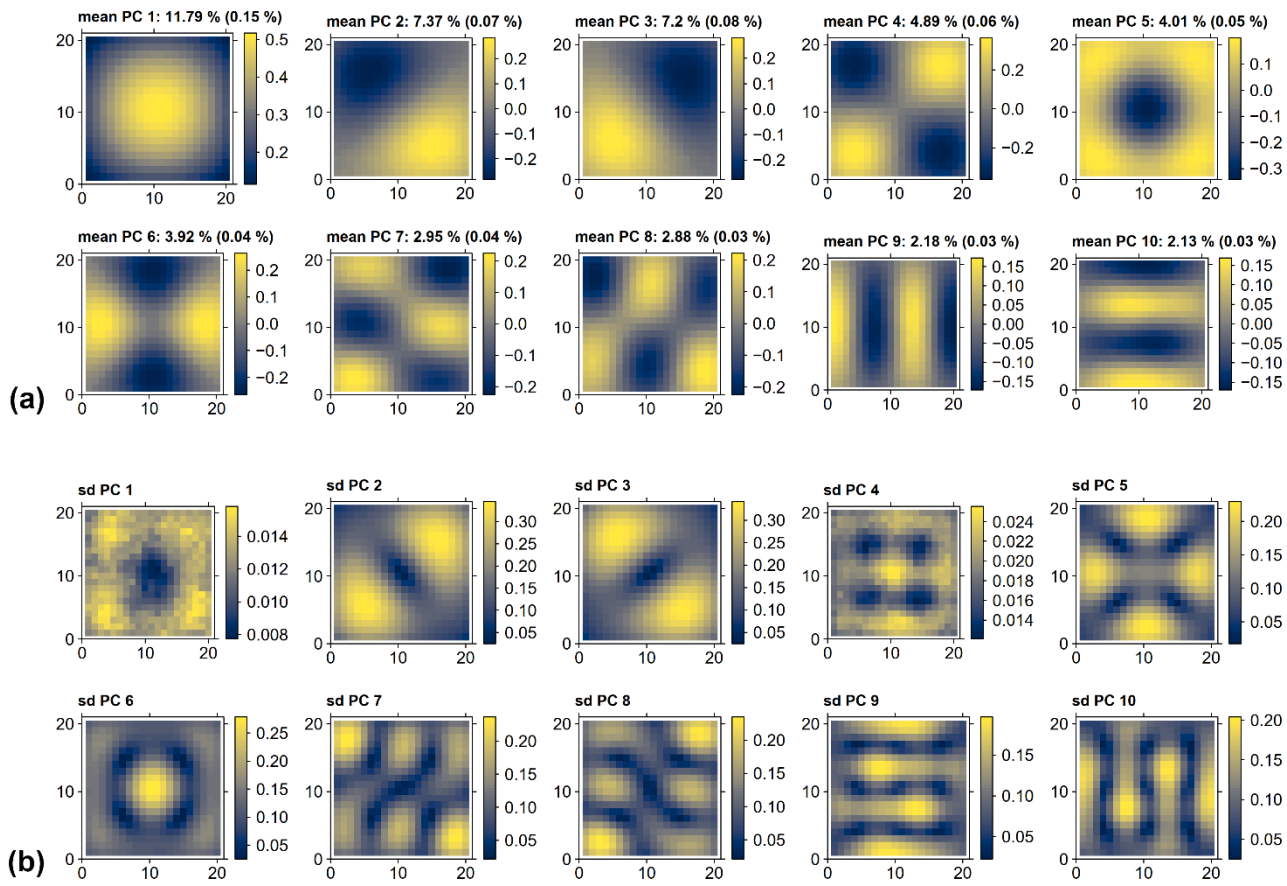
Figure S2 Detail plot of mean (a) and standard deviation (b) of the spatial patterns from the leading ten PCs of the data set ensemble with the square domain shown in Figure 8a and Figure 9a. The panel titles of (a) contain the mean (and standard deviation) of the fractions of variance assigned to the respective PCs from the 100 PCAs of the ensemble.
