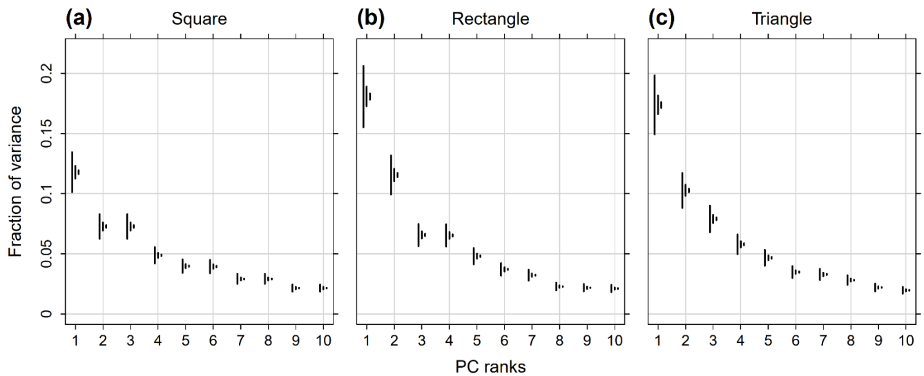
Figure S64 Variance representation of the ten leading PCs modelled with the analytic DD reference method using an isotropic exponential covariance model, a spatial correlation length of 10 cells and the domain boundaries (a) square, (b) rectangle and (c) triangle from Figure 6 Figure 3 . All cells within the boundaries were used. The upright bars show from left to right the 95 % confidence interval for an effective sample size of 100, 1 000 and 10 000 estimated with North's rule of thumb (North et al., 1982; Hannachi et al., 2007). For time series without temporal autocorrelation the effective sample size equals the time series length.
