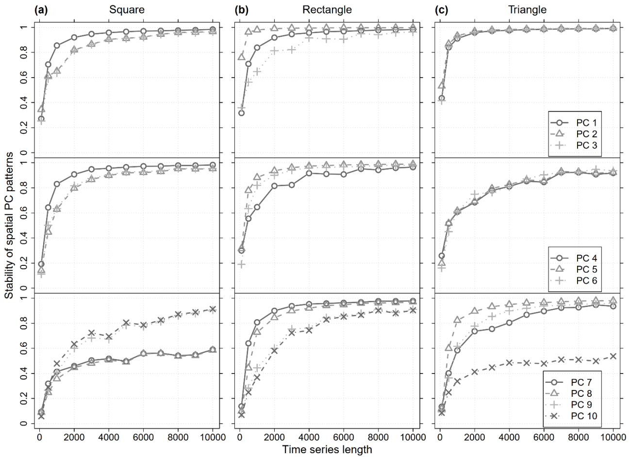
560 Figure 1240 Stability of the spatial PC patterns as in Figure 7Figure-4 but for the patterns of the homogeneous subsampling variant (Figure 10Figure-8).
