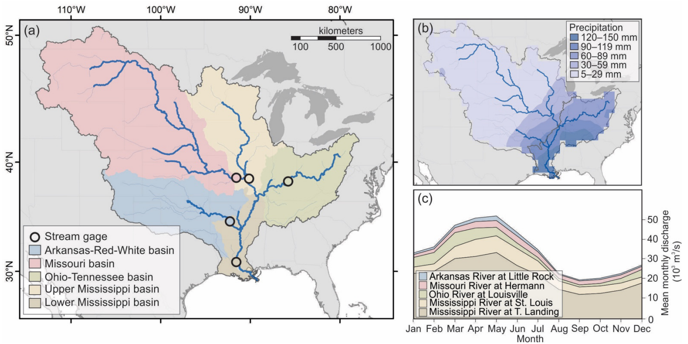
40 Figure 1. Mississippi River Basin and major tributaries: (a) Basins of major tributaries and corresponding stream gage locations. (b) Monthly mean (mm/month) precipitation from Global Precipitation Climatology Center (GPCC) 10 and grouping of subbasins into Eastern and Western Basins (gray line). (c) Monthly mean discharge from stream gages on the major tributaries (1950–2010).
