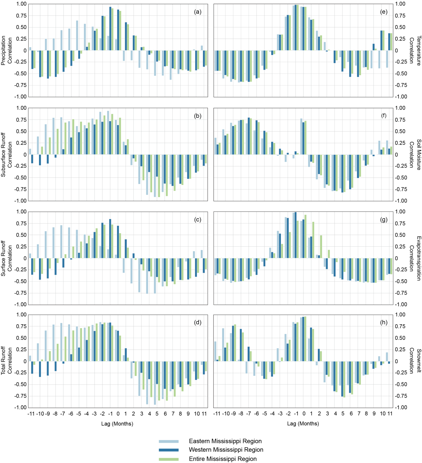
415 Figure 5. Monthly lag correlation values for each hydrologic variable [a) precipitation, b) subsurface runoff, c) surface runoff, d) runoff, e) temperature, f) soil moisture, g) ET, h) snowmelt], for each region: Eastern Mississippi basin (light blue), Western Mississippi Basin (dark blue), Entire Mississippi basin (green).
