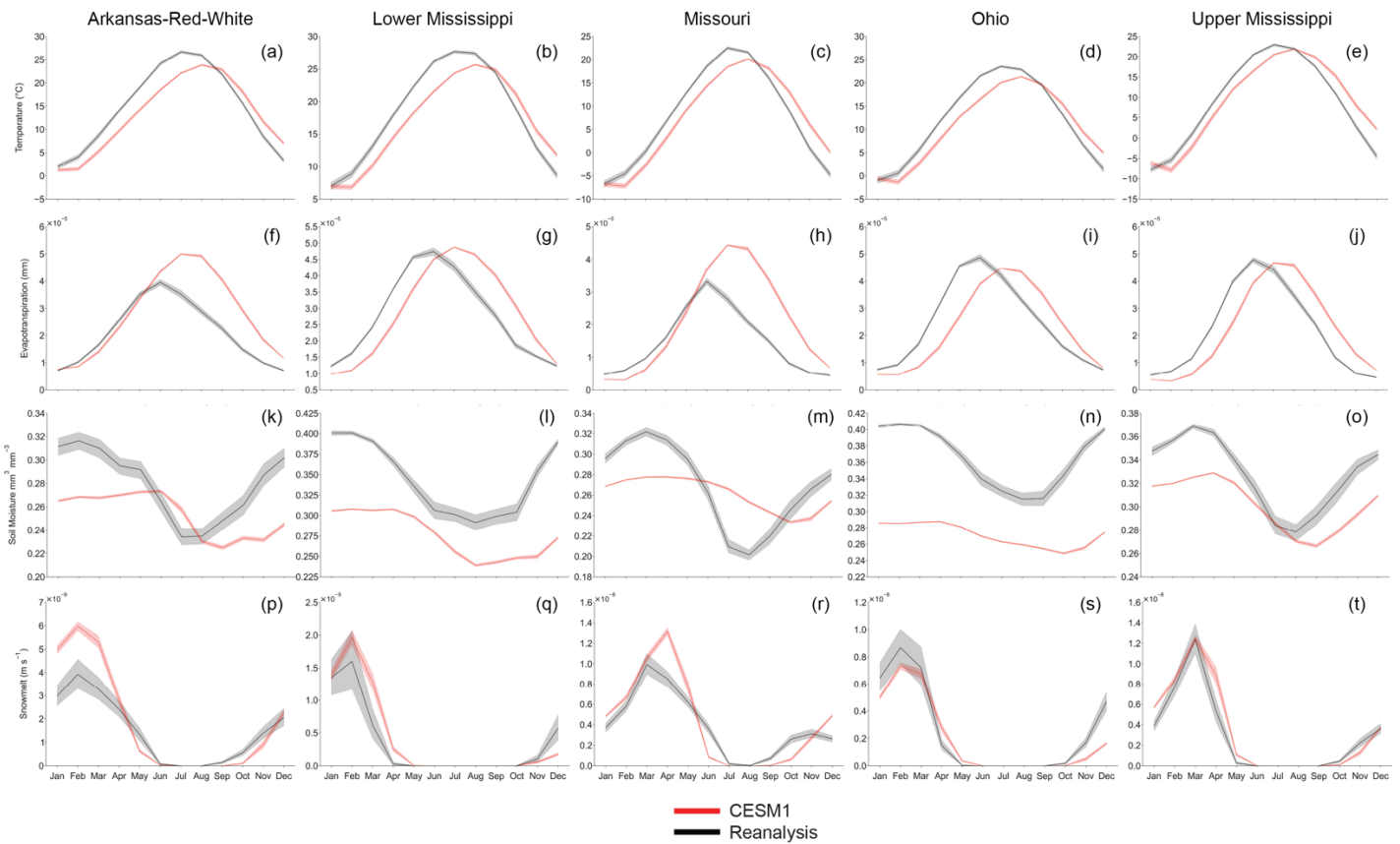
745 Figure A3: Monthly mean CESM1 simulated (red) values compared to reanalysis (black) values for temperature (a-e), evapotranspiration (f-j), soil moisture (k-o), and snowmelt (p-t) for the major subbasins: Arkansas-Red-White, Lower Mississippi, Missouri, Ohio, Upper Mississippi. Shading represents a 95% confidence interval from ensemble spread for CESM1 data (50 ensemble members) and interannual variability for both CESM1 and reanalysis data.
