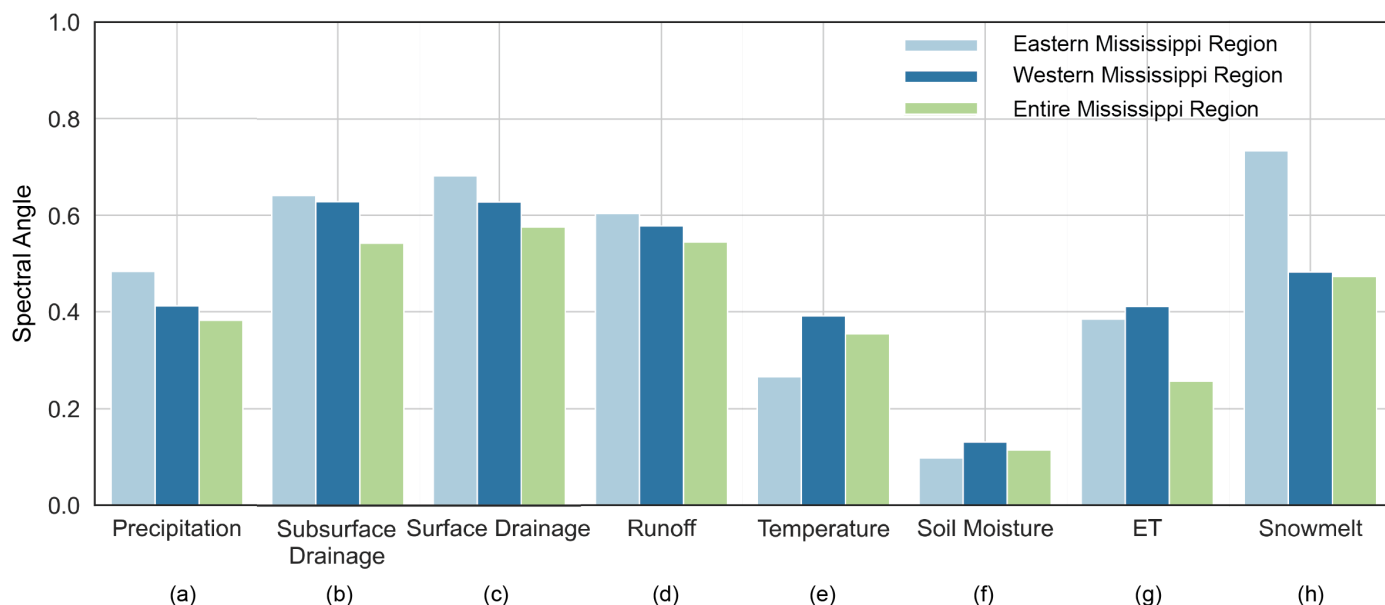
445 Figure 6. Spectral angle (SA) values for each hydrologic variable [a) precipitation, b) subsurface runoff, c) surface runoff, d) runoff, e) temperature, f) soil moisture, g) ET, h) snowmelt], for each region: Eastern Mississippi Basin (light blue), Western Mississippi Basin (dark blue), Entire Mississippi basin (green).
