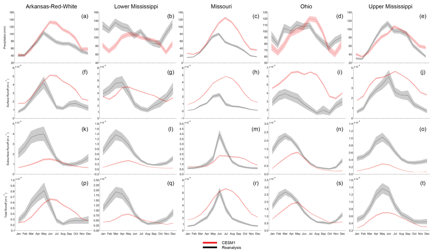
Figure 2A: Monthly mean CESM1 simulated (red) values compared to reanalysis (black) values for precipitation (a-e), surface runoff (f-j), subsurface runoff (k-o), and runoff (p-t) for the major subbasins: Arkansas-Red-White, Lower Mississippi, Missouri, Ohio, Upper Mississippi. Shading represents a 95% confidence interval from ensemble spread for CESM1 data (50 ensemble members) and interannual variability for both CESM1 and reanalysis data.
