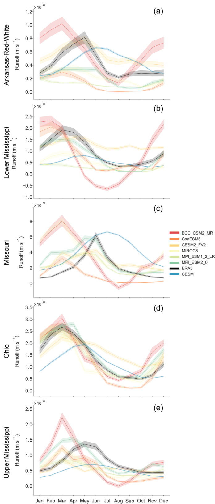
Figure 4A: Monthly mean simulated runoff (m/s) from selected CMIP6 models (BCC CSM2 MR [red], CanESM5 [dark orange], CEMS2 [light orange], MIROC6 [yellow], MPI ESM1 2 LR [light green], MRI ESM2 0 [dark green]), CESM1 [blue], and ERA5 reanalysis [black] for the Arkansas-Red-White (a), Lower Mississippi (b), Missouri (c), Ohio (d), and Upper Mississippi (e) basins. Shading represents a 95% confidence interval from interannual variability.
