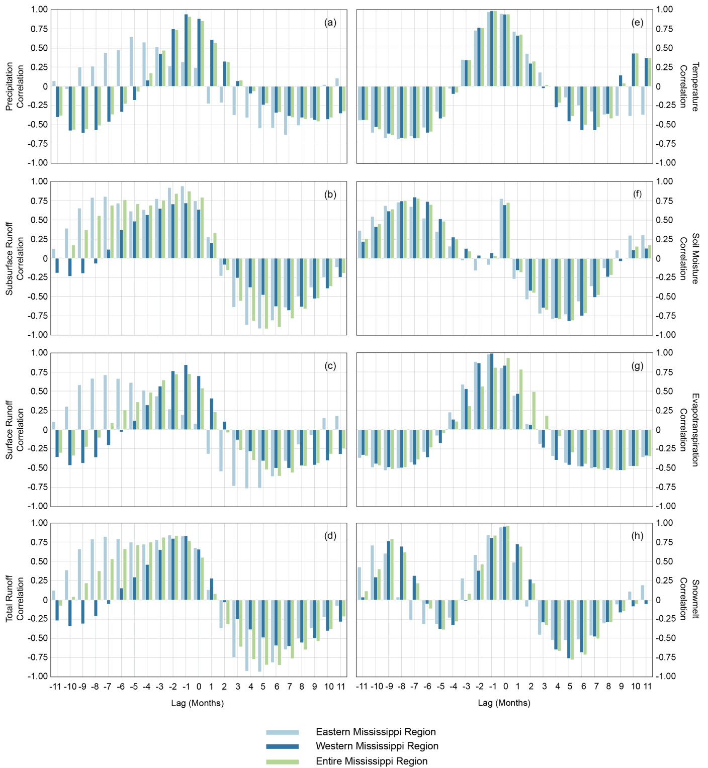
410 Figure 5. Monthly lag correlation values for each hydrologic variable [a) precipitation, b) subsurface runoff, c) surface runoff, d) runoff, e) temperature, f) soil moisture, g) ET, h) snowmelt], for each region: Eastern Mississippi basin (light blue), Western Mississippi Basin (dark blue), Entire Mississippi basin (green).
