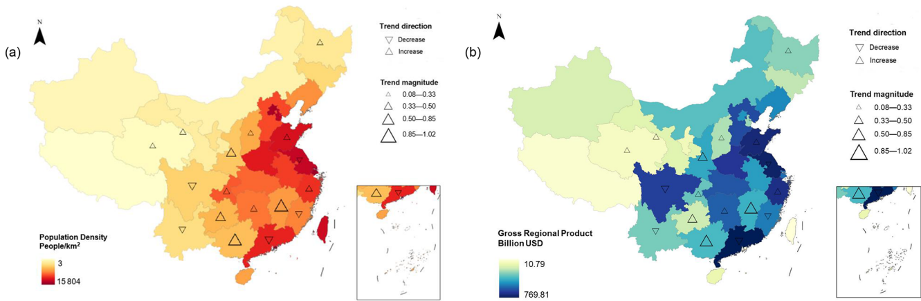
Figure 7. The analysis of flood event trends across the Chinese provinces from 2000 to 2022, shown in relation to (a) population density and (b) gross regional product (GRP). The triangles indicate trends: downward triangles represent decreases, and upward triangles represent increases, with the sizes corresponding to the trend values. Publisher’s remark: please note that the above figure contains disputed territories.
