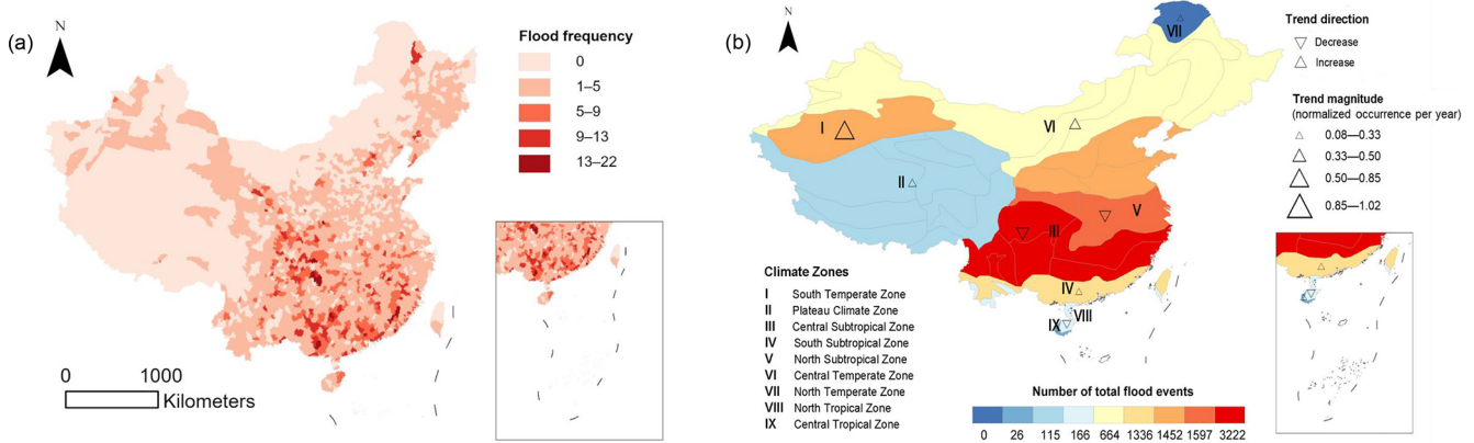
Figure 6. TS2 Spatial distribution of flood occurrences and trends in China (2000–2022). (a) The accumulated flood occurrences at the county level. (b) The accumulated flood occurrences and trends across different climate zones, where Roman numerals denote the climate zones. The triangles indicate trends; downward triangles represent decreases, and upward triangles represent increases, with the sizes corresponding to the trend values. Publisher’s remark: please note that the above figure contains disputed territories.
