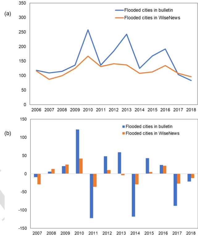
Figure 4. The comparison between the number of flooded cities extracted from the news and the China Flood and Drought Bulletin for each year. (a) The time series of both datasets. (b) Year-to-year changes in both datasets, with the y axis showing the difference in values from the previous year. The positive bars indicate an increase compared to the previous year, whereas the negative bars indicate a decrease.
