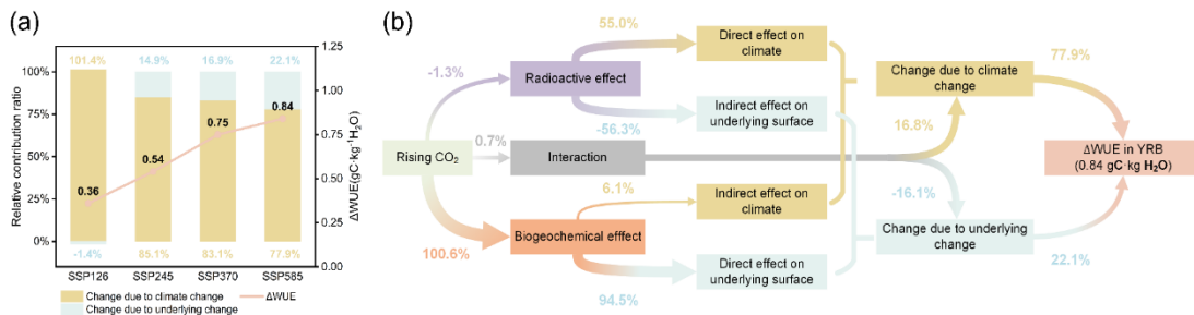
Figure 7. Attribution results for WUE changes. (a) Changes in WUE in the YRB under different SSPs, along with the relative contributions of climate factors and underlying surface factors. The stacked chart represents the relative contribution rates of climate change and underlying change to WUE variations under different scenarios. The line graph depicts the average WUE changes (between 1985-2014 and 2070-2099) across the basin under various scenarios. (b) Land-atmosphere decoupling attribution results based on SSP585 and CO 2 experiments. The percentage represents the relative contribution rates.
