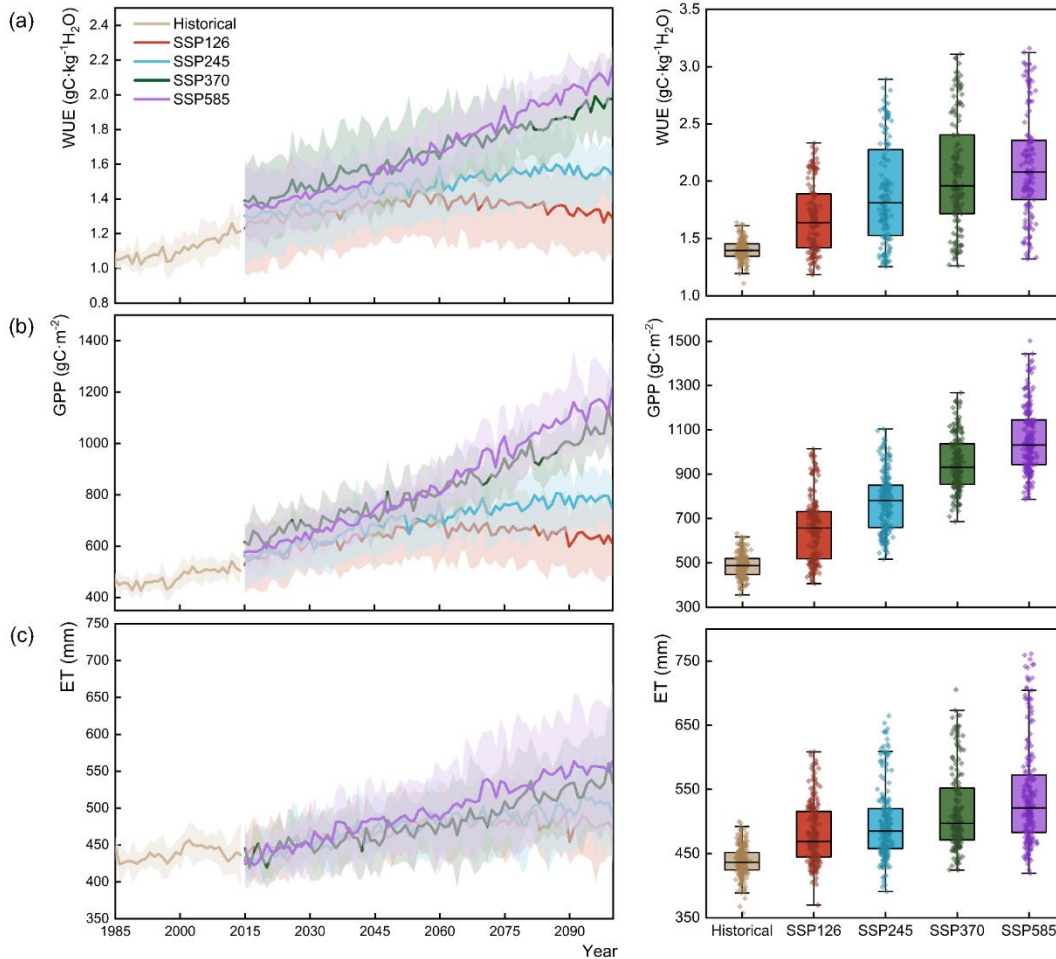
Figure 3. Annual averaged time series and box plots during historical (1985-2014) and future (2070-2099) period (a) WUE, (b) GPP, and (c) ET from the CMIP6 multi-model ensemble in the YRB.
