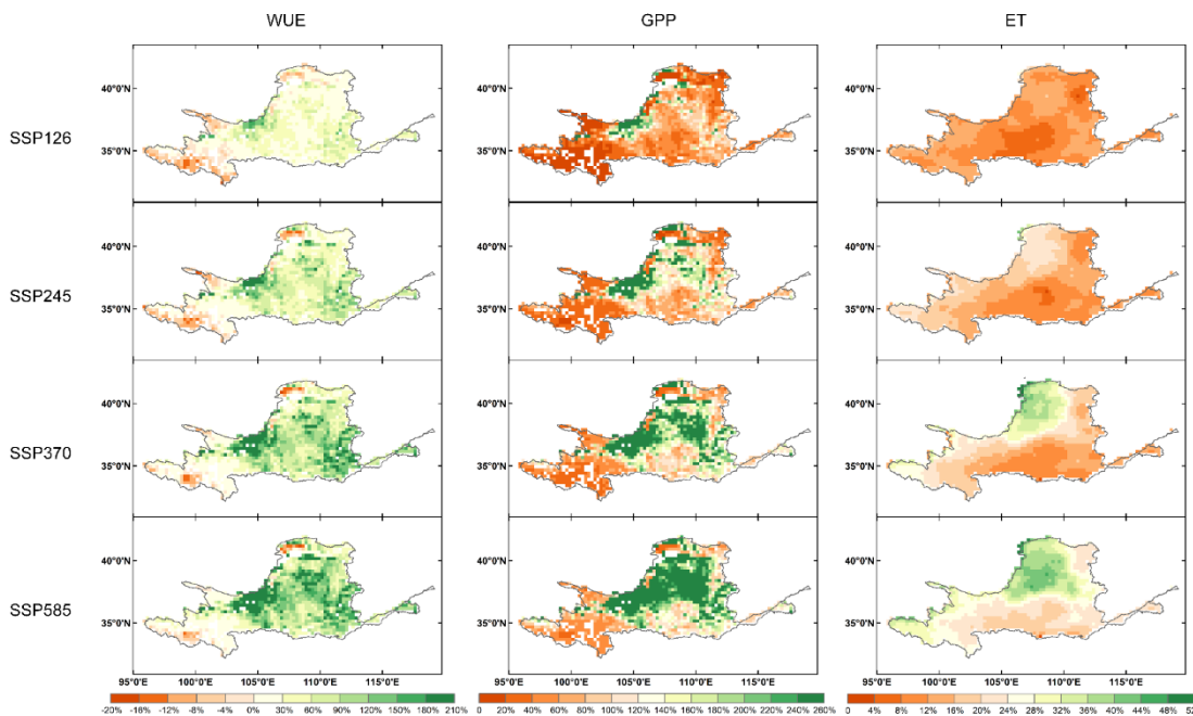
340 Figure 5. Spatial distribution of the relative changes in WUE (the first column), GPP (the second column) and ET (the third column) compared to the historical period under different scenarios.
