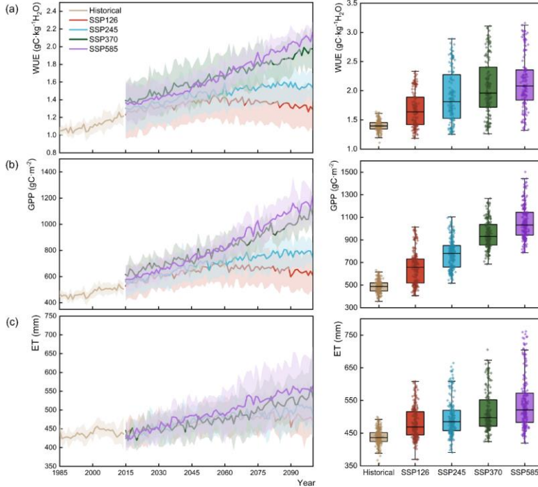
345 Figure 3. Annual averaged time series and box plots during historical (1985-2014) and future (2070-2099) period (a) WUE, (b) GPP, and (c) ET from the CMIP6 multi-model ensemble in the YRB.
