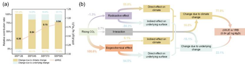
440 Figure 7. Attribution results for WUE changes. (a) Changes in WUE in the YRB under different SSPs, along with the relative contributions of climate factors and underlying surface factors. The stacked chart represents the relative contribution rates of climate change and underlying change to WUE variations under different scenarios. The line graph depicts the average WUE changes (between 1985-2014 and 2070-2099) across the basin under various scenarios. (b) Land-atmosphere decoupling attribution results based on SSP585 and CO 2 experiments. The percentage represents the relative contribution rates.
