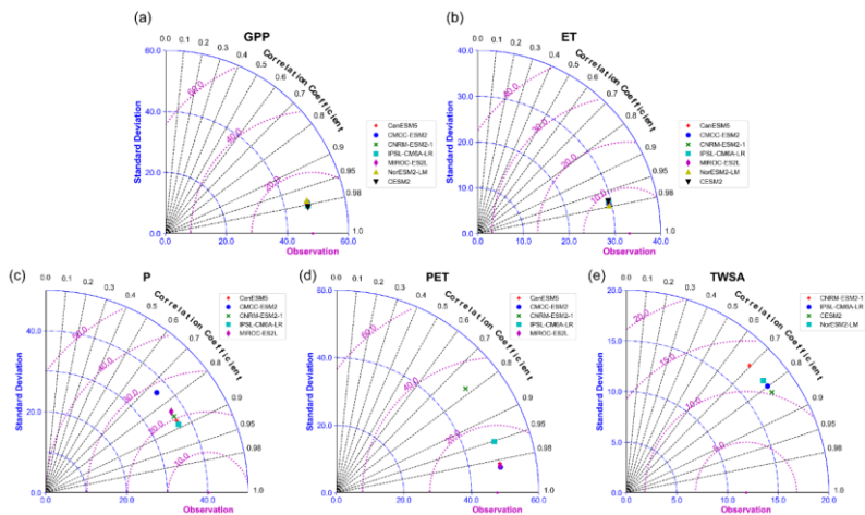
325 Figure 2. Taylor diagrams for corrected GCMs data of (a) GPP, (b) ET, (c) P, (d) PET, and (e) TWSA.
