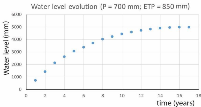
Figure 9: Results of the FdP water level assuming stable humid conditions during 17 years, when the water level stabilizes at ca. 5 m above the lakebed.
