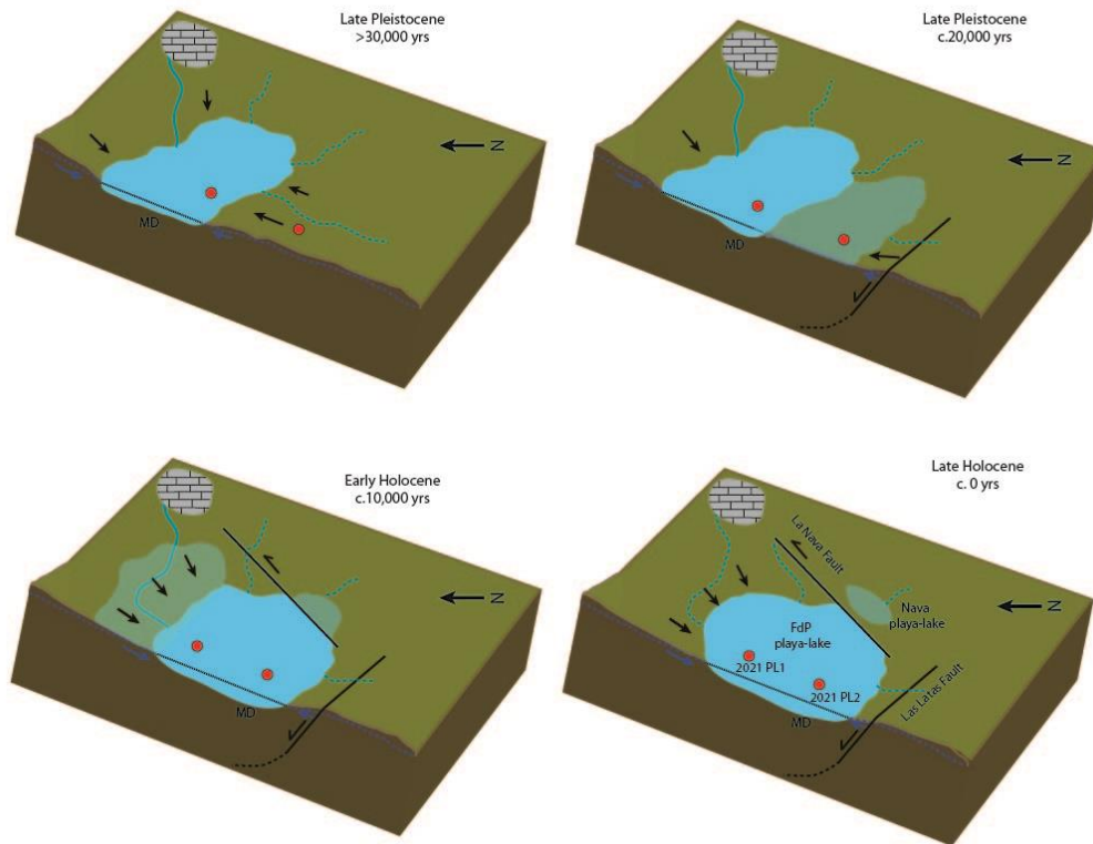
420 Fig. 12. Schematic evolution of the FdP playa-lake during the Late Pleistocene and Holocene showing the main active structures and the evolution of the flooded area according to neotectonics and variations on climate. Black arrows show main sediment supply. MD: Main deposcenter. Core locations are represented by red dots.
