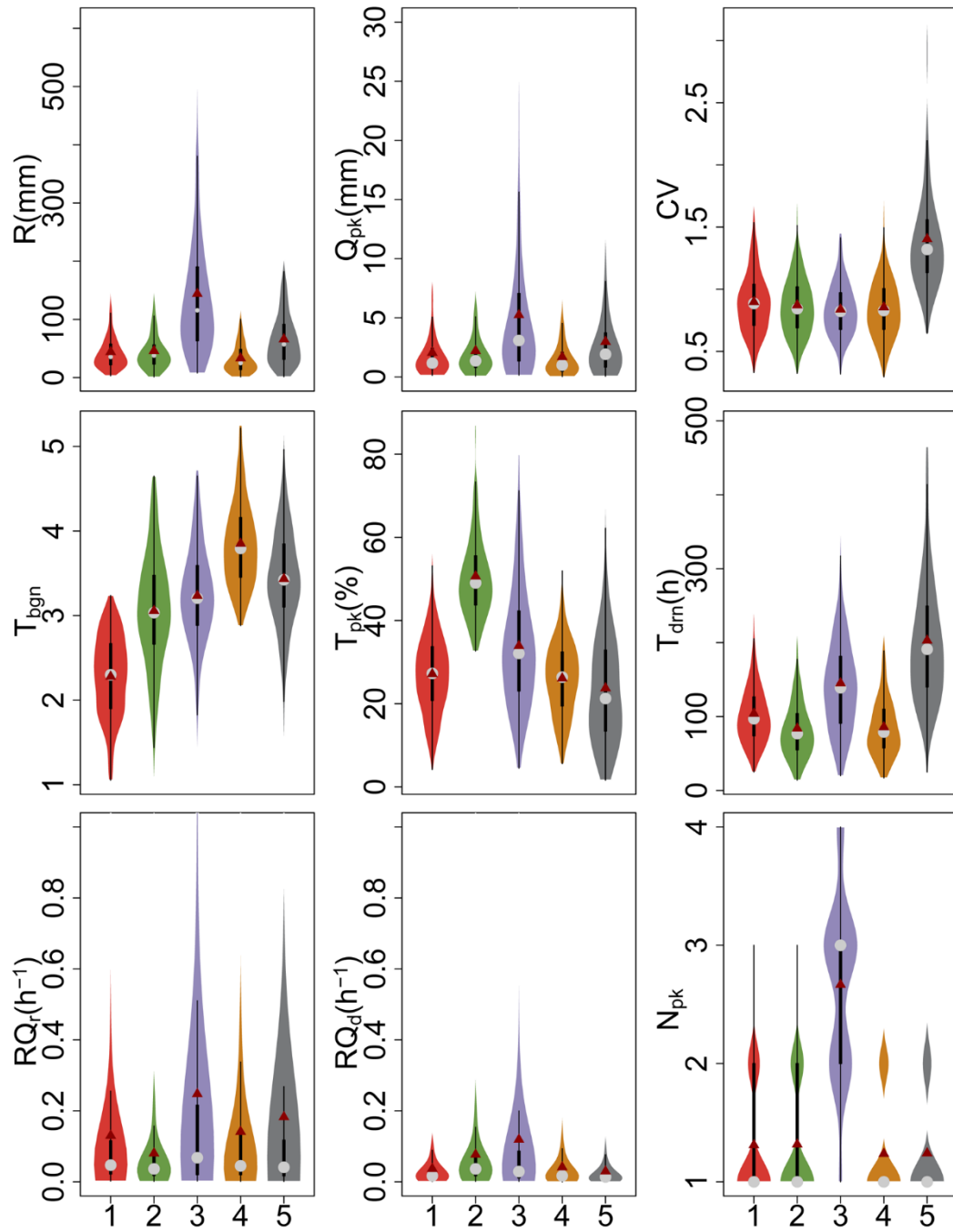
Figure 2. Variations of flood response metrics among Classes 1–5. The solid dark red dot and gray dot define the mean and 50th percentile values, respectively. Each black box means the 25th and 75th percentile values, and the vertical line defines the minimum and maximum values without outliers. The violin shape means the frequency distribution of flood response metric.
