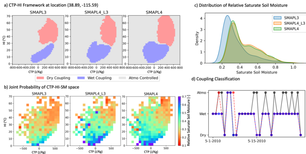
485 Figure 7: Multifaceted assessment of coupling classification influenced by soil moisture across SMAPL3, SMAPL4_L3, and SMAPL4 data at a specific grid location (38.89, -115.59) situated in Nevada, USA (a) CTP-HI framework (b) A joint probability space of CTP-HI-SM (c) Saturate soil moisture distribution (d) Coupling classification time series for May 2010.
