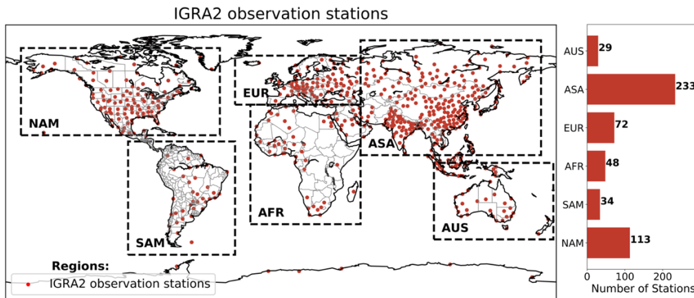
300 Figure 2: IGRA2 observation stations across the Globe, along with regions selected for further analysis and the number of observation stations in each region.
