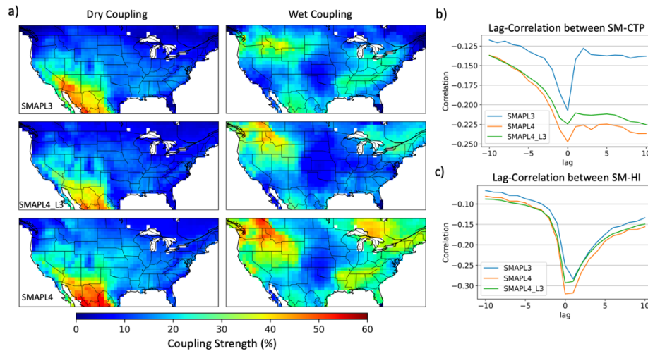
445 Figure 6: Comparative analysis of L-A coupling strength using SMAPL3, SMAPL4_L3, and SMAPL4 data (a) coupling strength for the dry and wet coupling regime and (b and c) lag- correlation between soil moisture and CTP and HI averaged over the contiguous United States.
