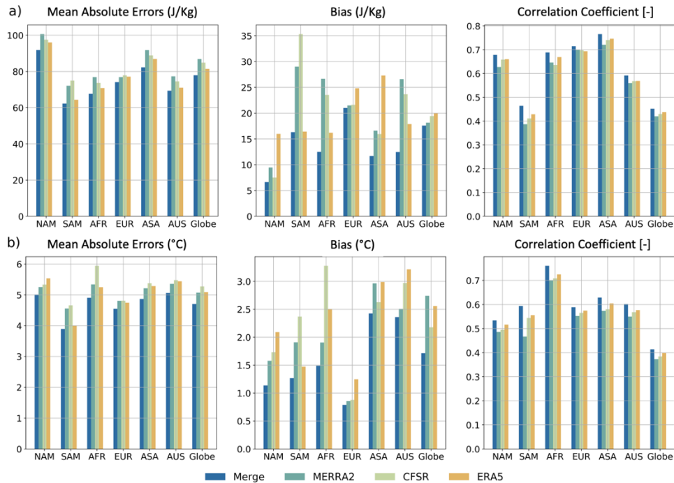
395 Figure 5: Bar plot of performance metric and intercomparison of merged data and reanalysis with satellite remote sensing from AIRSv7 in different region and globally for (a) CTP and (b) HI.
