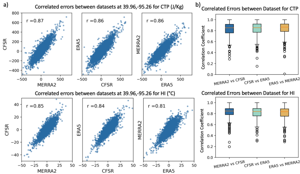
350 Figure 3: (a) Observed errors between IGRA2 and reanalysis datasets at a location in Kansas, United States (Latitude: 39.96, Longitude: -95.26) for CTP and HI from 2003 to 2022, along with the Pearson correlation displayed in the upper left corner. (b) Observed error correlation between reanalysis data sets at IGRA2 stations across the Globe (529 sites).
