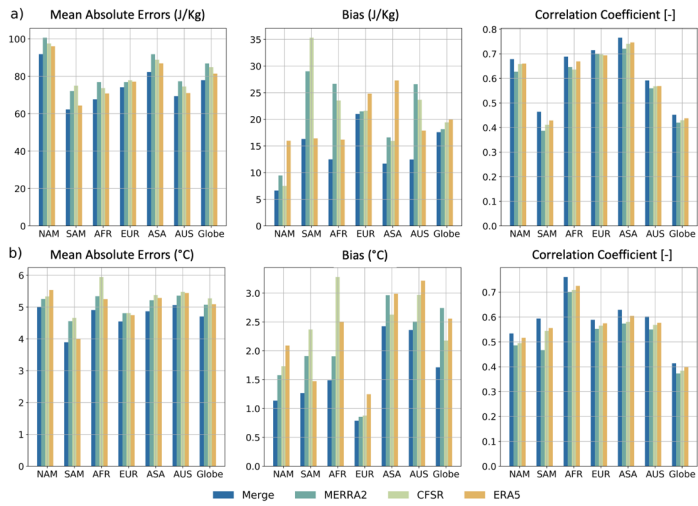
Figure 5: Bar plot of performance metric and intercomparison of merged data and reanalysis with satellite remote sensing from AIRSv7 in different region and globally for (a) CTP and (b) HI.
