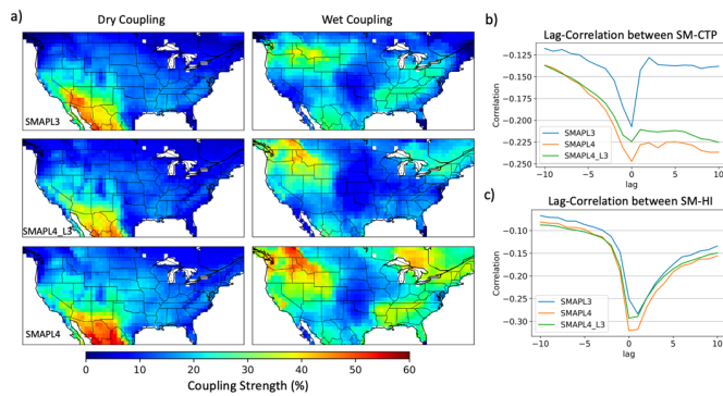
Figure 6: Comparative analysis of L-A coupling strength using SMAPL3, SMAPL4 L3, and SMAPL4 data (a) coupling strength for the dry and wet coupling regime and (b and c) lag- correlation between soil moisture and CTP and HI averaged over the contiguous United States.
