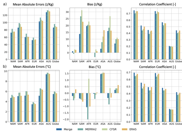
Figure 4: Bar plot of performance metric and intercomparison of merged data and reanalysis with radiosonde observation from IGRA2 in different region and globally for (a) CTP and (b) HI.
