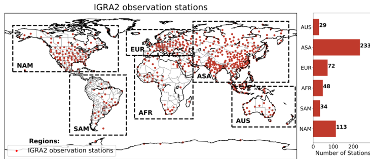
1155 Figure 2: IGRA2 observation stations across the Globe, along with regions selected for further analysis and the number of observation stations in each region.
