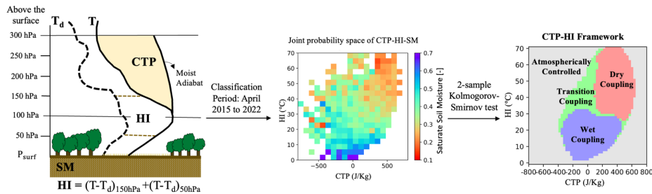
Figure 1: A visual representation of the Soil Moisture (SM), Convective Triggering Potential (CTP), and Humidity Index (HI) on a thermodynamic diagram, along with a joint probability space of CTP-HI-SM at a specific grid location (38.89, -115.59). The CTP-HI framework is depicted after applying a two-sample Kolmogorov-Smirnov test on the joint probability space of CTP-HI-SM for the classification period from April 2015 to 2022.
