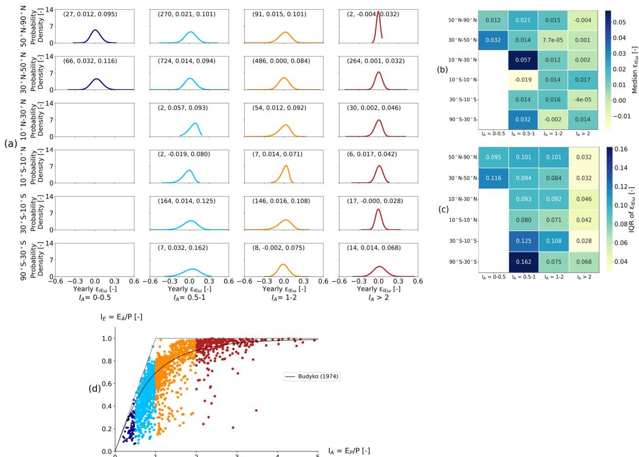
Figure 9: a) Regional marginal distributions of \varepsilon_{IE\omega} for defined latitude and I_A bins. The three numerical values in small brackets at the top of each panel presents number of catchments in that category, long-term median \varepsilon_{IE\omega} and IQR value of \varepsilon_{IE\omega} respectively, b) and (c) presents variation of median and IQR values of \varepsilon_{IE\omega} for the regional marginal distribution of \varepsilon_{IE\omega} , d) Long-term position (1901–2015) of catchments in Budyko space. The colour of the dots corresponds to the regional marginal distributions of \varepsilon_{IE\omega} for the corresponding I_A bin.
