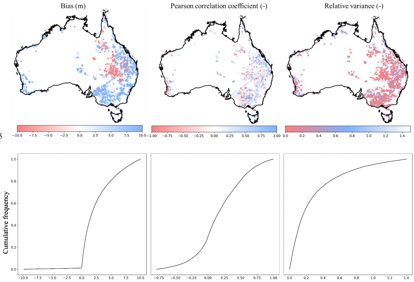
Figure 3: Evaluation statistics of observed groundwater depths against simulated groundwater depth head; top row: maps with values per observed location; bottom row: associated cumulative frequency distributions; left column: Bias (m); middle column: Pearson correlation coefficient; right column: relative variance. The white areas on the maps are locations without observation data.
