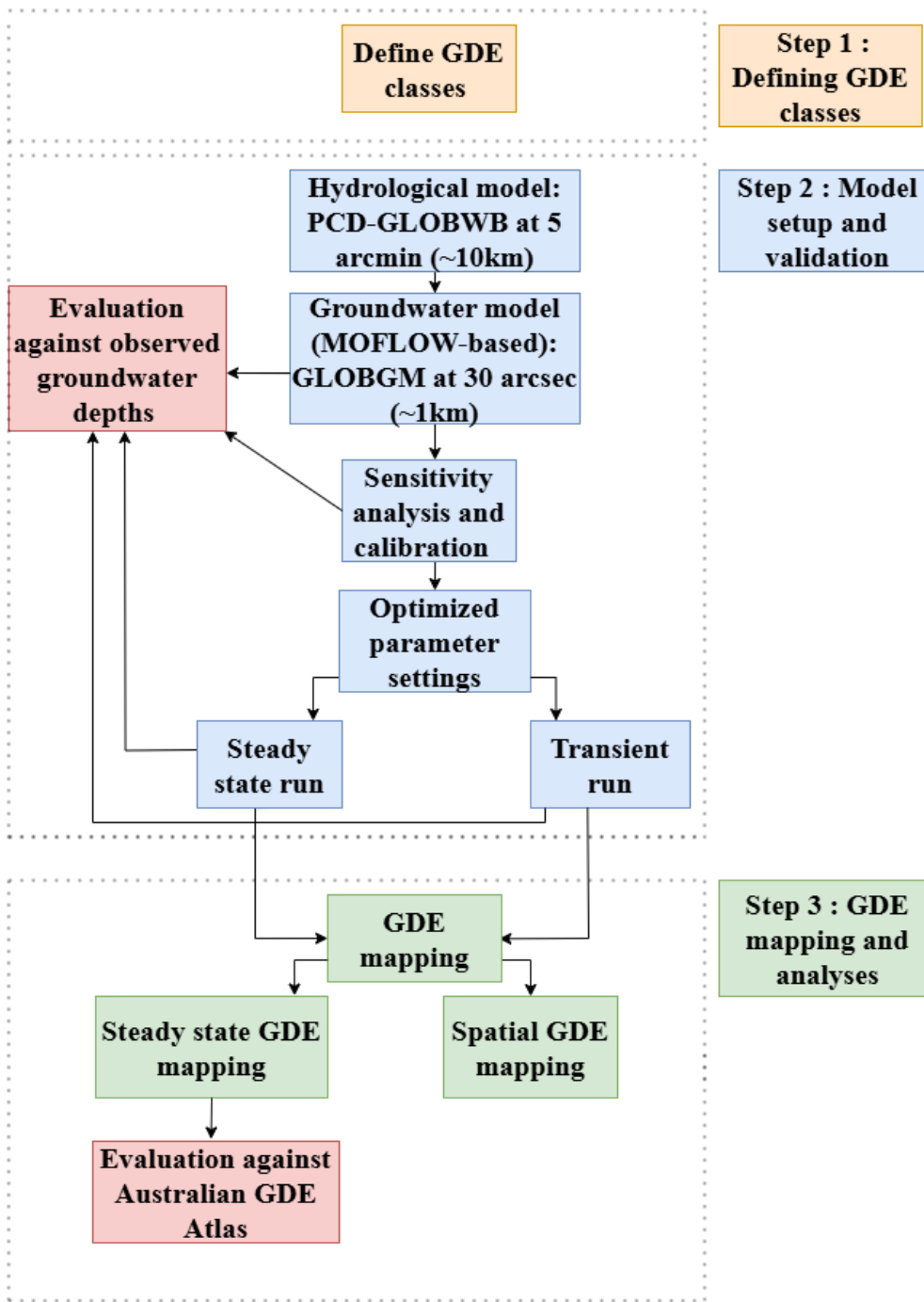
105 Figure 1: Groundwater dependent ecosystems (GDE) modelling mapping framework using a high-resolution groundwater model.
