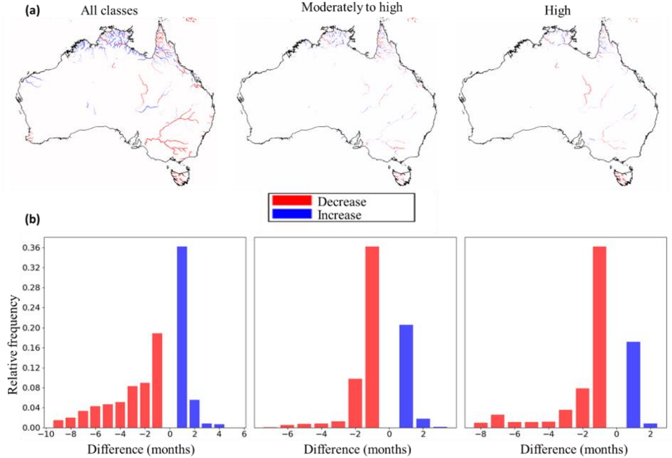
Figure 5: Change in groundwater dependency of aquatic GDEs between 1979-2000 and 2001-2019; (a) Maps of the direction of change in the average number of months that aquatic GDEs depend on groundwater; the left figure shows the change in the number of months \frac{Q_{gw}}{Q} > 0 (low to high dependency), the middle figure \frac{Q_{gw}}{Q} > 0.5 (moderate to high dependency) and the right figure \frac{Q_{gw}}{Q} > 0.75 (high dependency); Red areas indicate a decrease in the average number of months with groundwater dependency and blue indicates an increase; (b) associated frequency distributions of change in number of months.
