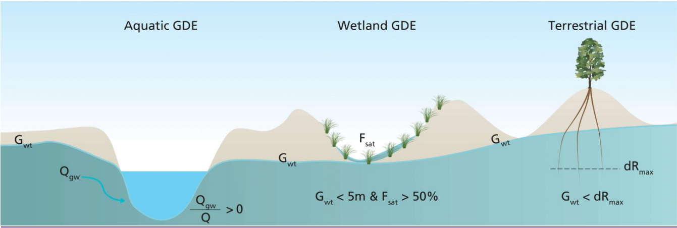
Figure 2: Criteria for defining ecosystem dependency on groundwater dependent ecosystems, with Q_{gw} \equiv local groundwater discharge, Q \equiv accumulated stream flow, G_{wt} = groundwater table depth, F_{sat} = saturated area fraction and dR_{max} = maximum rooting depth.
