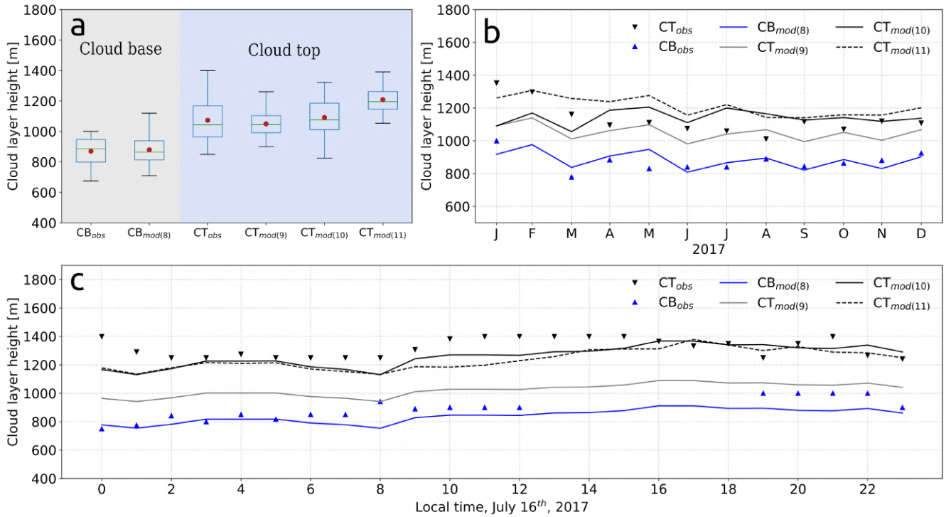
Figure 4. (a) Annual, (b) monthly-averaged, and (c) typical diurnal cycle of CB and CT comparisons between observations (obs) and modeling (mod). The number sub scripts refers to the equation number in sections 2.1.2 and 2.1.3.
