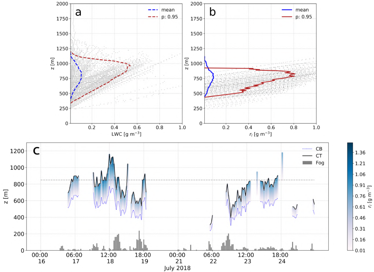
Figure 5. Vertical profiles r_l (in \text{g m}^{-3} ) (a) derived from a microwave radiometer and Doppler lidar observations (Schween et al., 2022; CLU, 2024) and (b) estimated by the AMARU model over Diego Aracena Airport. Grey dots represent hourly-averaged profiles filtered by percentile 0.99; red lines represent percentile 0.95, and the blue line represents the mean. (c) The evolution of the vertical profile simulated by the AMARU model for the Alto Patache Site. Grey bars at the bottom represent fog collection measurements at 850 m (dashed line).
