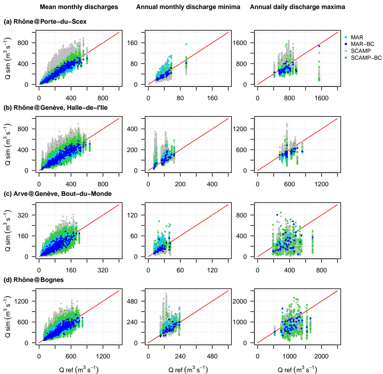
Figure 11. Scatter plots of mean monthly discharges, low-flows-annual monthly discharge minima and annual daily discharge maxima at (a) Rhône@Porte-du-Scex, (b) Rhône@Genève, Halle-de-l'Ile, (c) Arve@Genève, Bout-du-Monde, and (d) Rhône@Bognes for the 1961-2009 period. Q ref: simulated discharge from observed weather variables. MAR/MAR-BC: simulated discharge from the raw/bias-corrected weather scenario produced with the dynamical downscaling model MAR. SCAMP/SCAMP-BC: simulated discharge from the raw/bias-corrected weather scenarios produced with the statistical downscaling model SCAMP.
