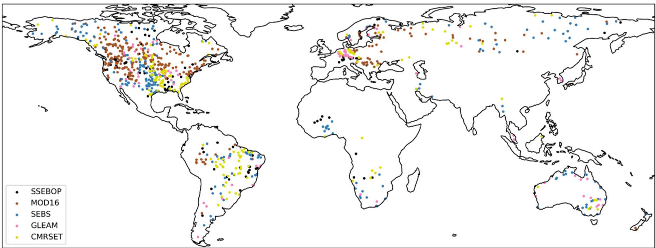
345 Figure 6: ET product used in combination with highest NSE at station
