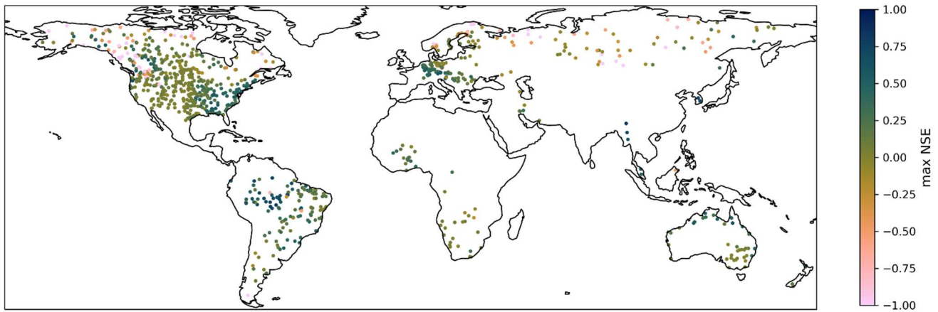
Figure 4: Max NSE achieved at each GRDC station
