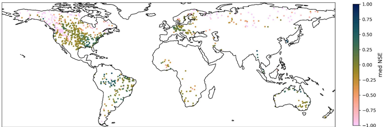
Figure 3: Median NSE for different product combinations at each GRDC station
