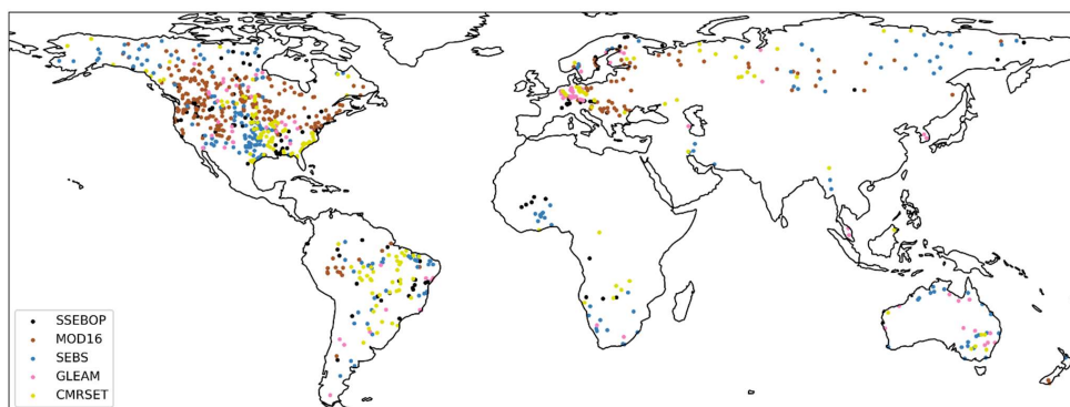
Figure 65: ET product used in combination with highest NSE at station
