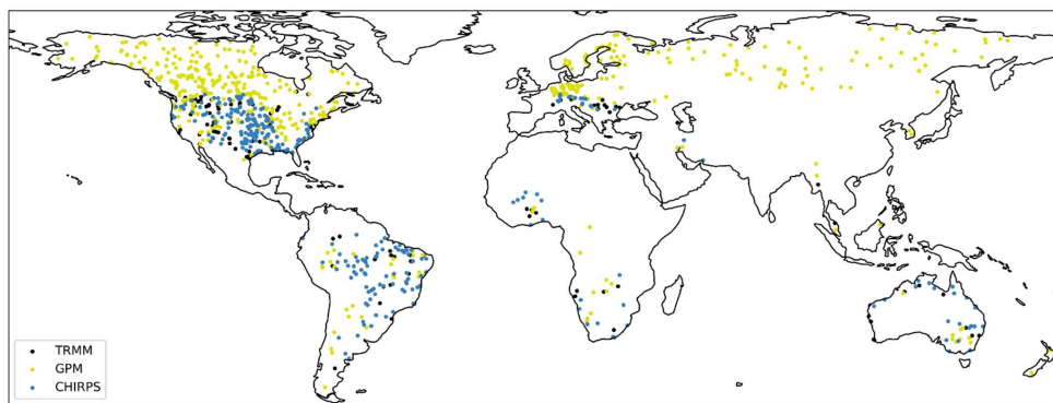
355 Figure 54: Precipitation product used in combination with highest NSE at station. Note that GPM is the only product available for latitudes >50°.
