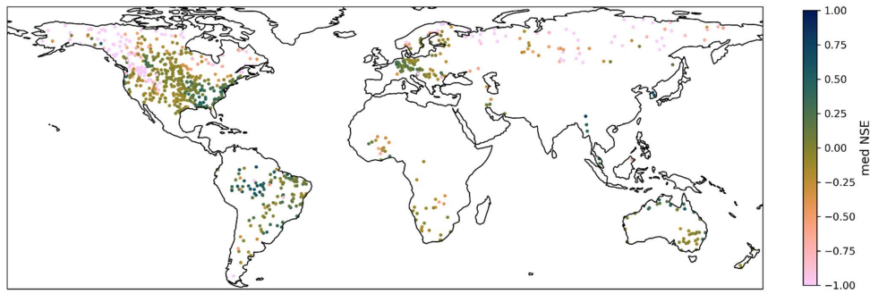
Figure 32: Median NSE for different product combinations at each GRDC station
