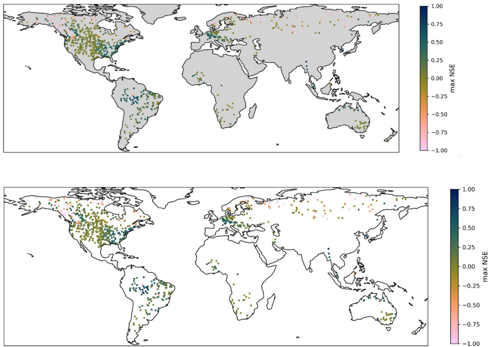
Figure 43: Max NSE achieved at each GRDC station
