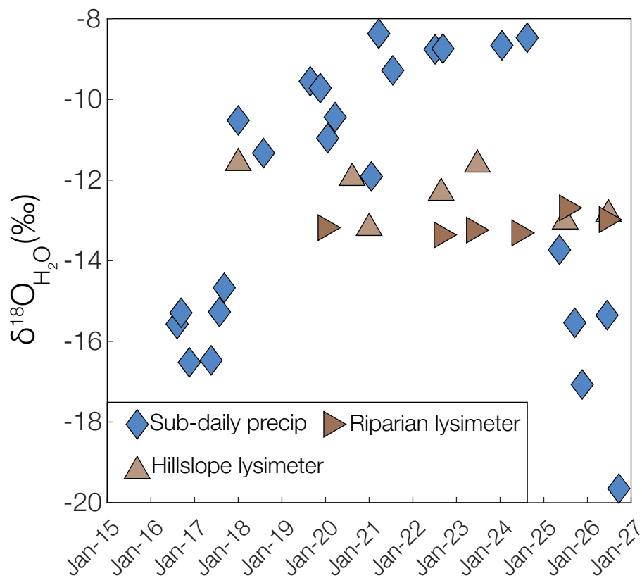
Figure S1. Precipitation and soil lysimeter water isotope ratios collected between 15 January 2017 and 27 January 2017 from a tropical montane cloud forested watershed in the southeastern Peruvian Andes mountains. Precipitation was collected in a bucket and sampled at least every 4 hours or more frequently.
