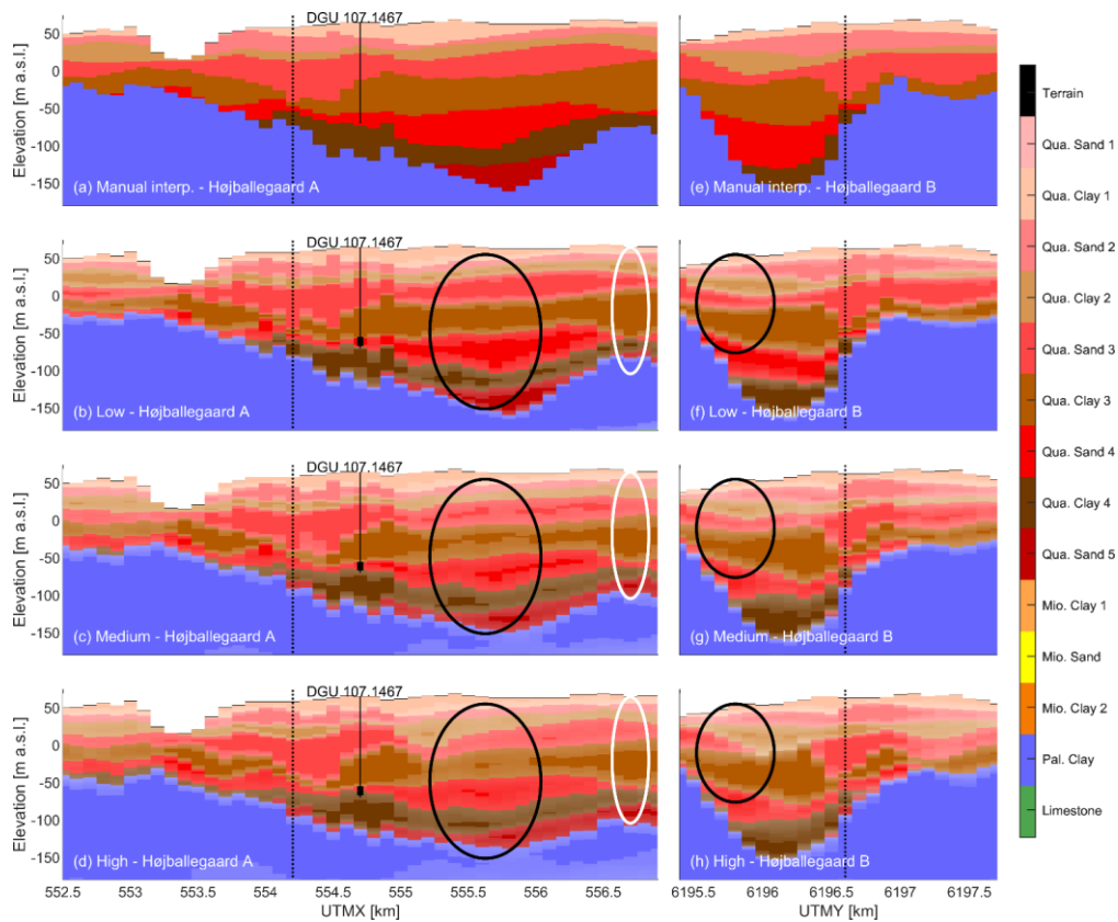
405 Figure 54: Two intersecting cross sections of summary statistics for the hydrostratigraphic model realizations; Højballegård A (a-d) and Højballegård B (e-h). Location of the cross sections can be seen in Figure 1. The intersection between the cross sections is marked with dotted lines. Abstraction boreholes from the well field are marked with a black line and the inlet filters marked with a black rectangle. The colors become increasingly transparent when the entropy is high. b,f) summary statistics from the Low uncertainty scenario, c,g) summary statistics from the Medium uncertainty scenario and d,h) summary statistics from the High uncertainty scenario. The black ellipses are examples for comparison of the boundary uncertainty in the three scenarios and the white ellipse shows an example of how borehole information lowers the uncertainty at the boundaries. 410
