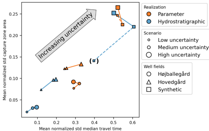
Figure 87: Mean normalized standard deviation of capture zone area and median travel time for all uncertainty scenarios (Low, Medium and High) and all well fields (Højballegård, Hovedgård and the Synthetic). The predictions have been marginalized on either parameter realizations (orange) or hydrostratigraphic realizations (blue). For the Synthetic well field in the low uncertainty scenario half of the hydrostratigraphic realizations had to be discarded and the predictions are therefore placed in a parenthesis.
