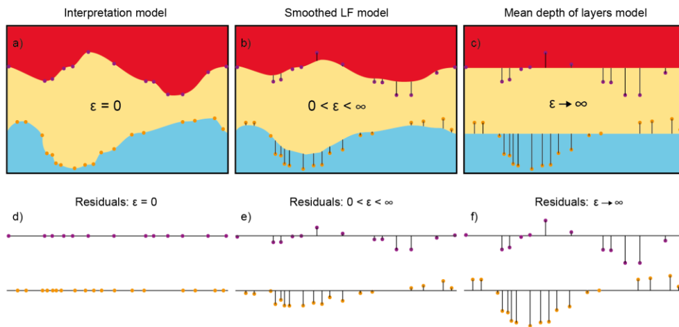
Figure 43: Schematic overview of effect of applying smoothing to a three-layer interpretation model based on interpretation points to obtain the overall structures in a LF model. a) The interpretation model has no smoothing ( \epsilon = 0 ), b) the interpretation model is smoothed ( 0 < \epsilon < \infty ) and c) the interpretation model is smoothed to a degree that only represents expected average depth of each layer ( \epsilon \rightarrow \infty ). The resulting residuals for each scenario are shown underneath in d)-f).
