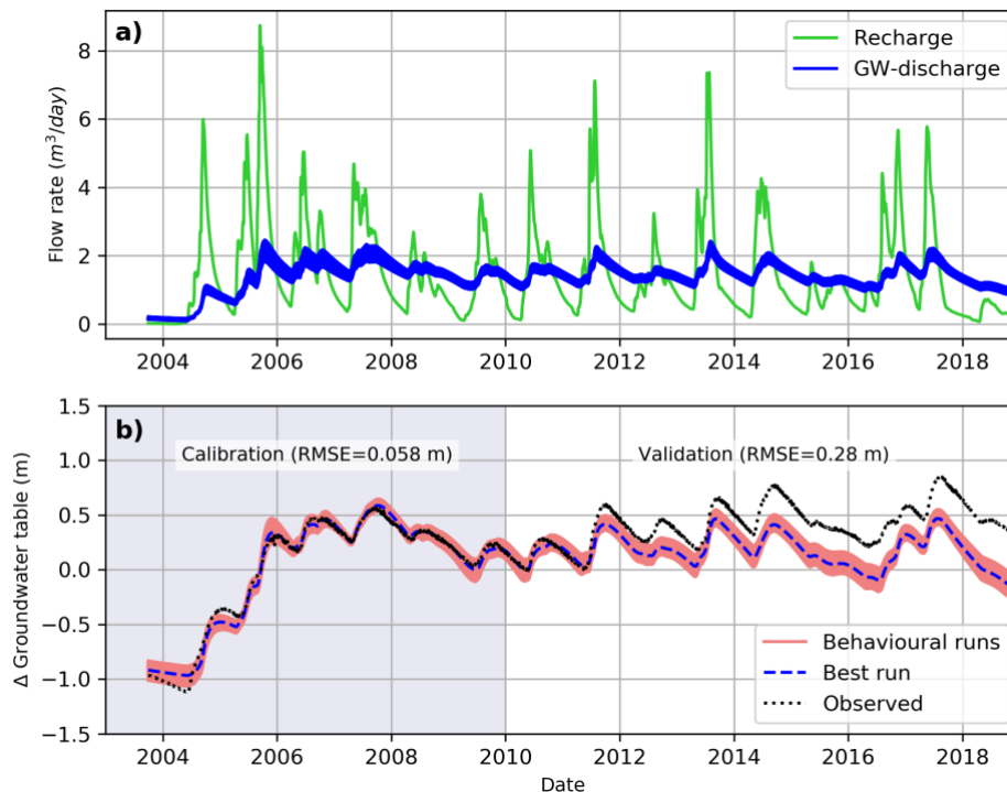
250 Figure 3: a) Upland recharge rates into the groundwater aquifer that are generated using MESH-OJP model and are used to drive the upland component, b) comparison between the simulated (V1) and observed changes in the GWT at OJP site. The uncertainty results (GW discharge and GWT) are obtained from the behavioural realizations using Monte-Carlo analysis.
