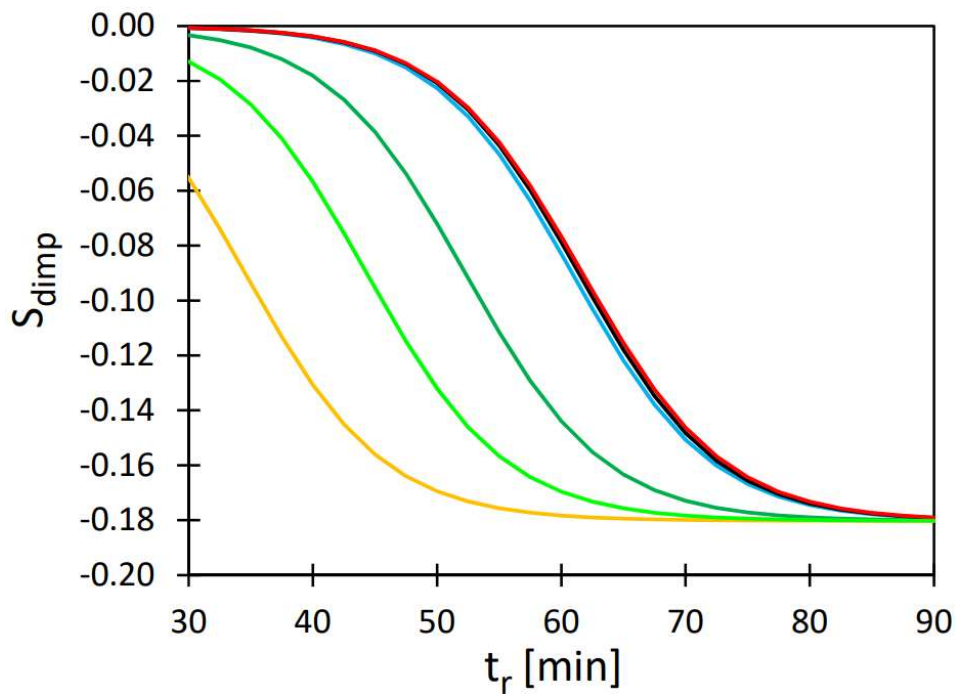
Figure S7. Influence of rainfall duration ( t_r ) depending on catchment and stormwater network characteristics (Imp, Impd, Vk, Jkp, Gk) on the sensitivity coefficient S_{dimp} . (L163)
