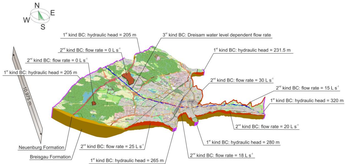
Figure S1.1. Numerical subsurface model of Freiburg consisting of the Neuenburg Formation (upper layer) and the Breisgau Formation (lower layer). The model illustration is ten times stretched in vertical direction. © OpenStreetMap contributors 2022. Distributed under the Open Data Commons Open Database License (ODbL) v1.0.
