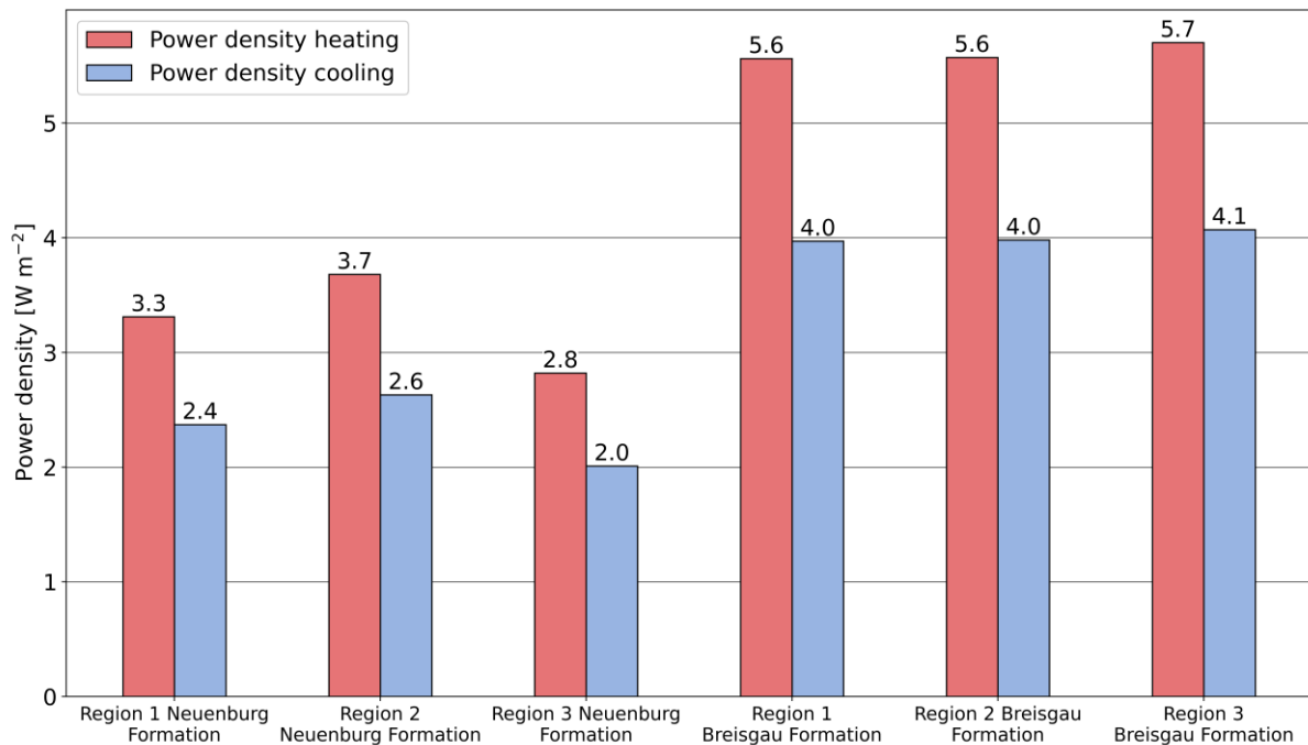
Figure S2. ATES Power densities for Neuenburg and Breisgau Formations when using the \pm 1 K-isotherms after 30 years for delineating the TAZ. ATES systems in the Neuenburg Formation are modeled as 2-doublet configurations. Systems in the Breisgau Formation use a 3-doublet configuration.
