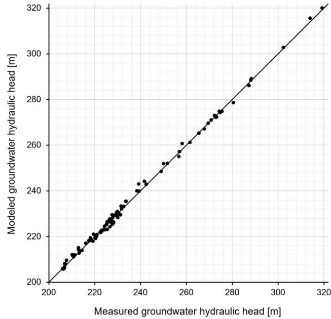
Figure S1.2. Modeled groundwater hydraulic heads plotted against measured groundwater hydraulic heads. The calibration results in a high coefficient of determination of 0.998. The root mean square deviation is 1.21 m.
