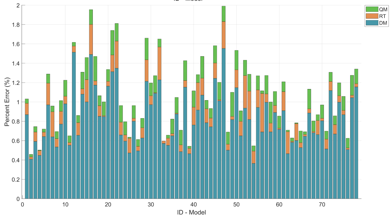
321 Figure 7 Median of Percentage Errors of total precipitation at the multiyear level to each model. Without the application of 322 downscaling techniques - WDS, and with the application of Delta Method - DM, Quantile Mapping - QM, and Regression 323 Trees - RT as downscaling techniques.
