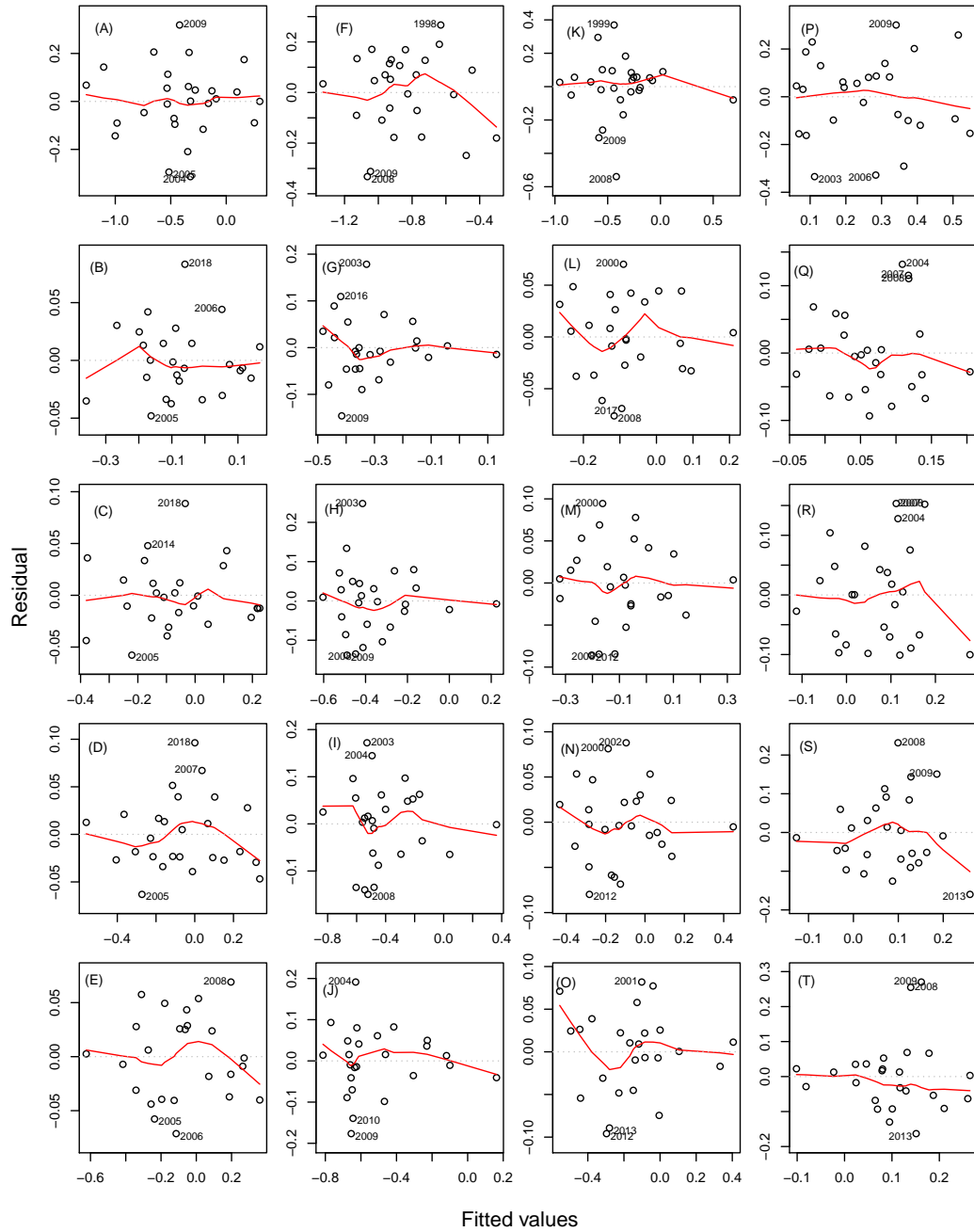
Figure B1. Residuals vs fitted for the linear models across different climate zones (columns from left to right: equatorial, arid, temperate, snow) and for the scPSDI and SPEI \tau with different integration times (rows from top to bottom: scPSDI and SPEI \tau with \tau \in \{03, 06, 12, 24\} ).
