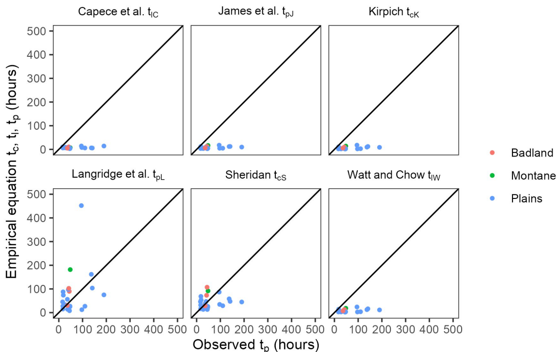
Figure 6: Empirical equation t_i , t_c and t_p vs. observed t_p for the study basins. The lines are 1:1.
