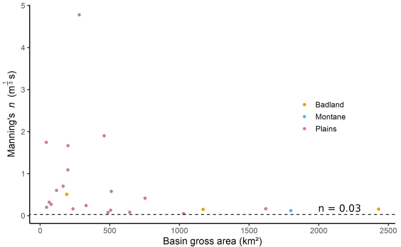
Figure 9: Manning's n vs. gross area of each basin. The dashed horizontal line represents the value of n for a clear straight channel (0.03).
