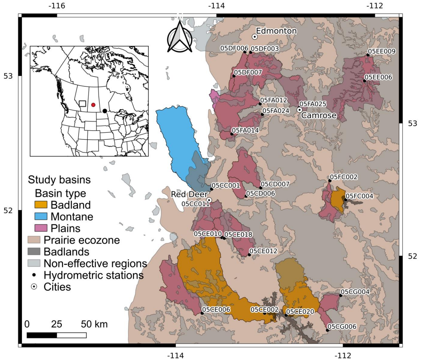
Figure 2: Map of the study basins in central Alberta, shaded by basin type. The Canadian Prairie ecozone (tan shading), non-effective regions (light gray shading) and badlands (dark grey shading) are also plotted. The locations of the gauging stations of
