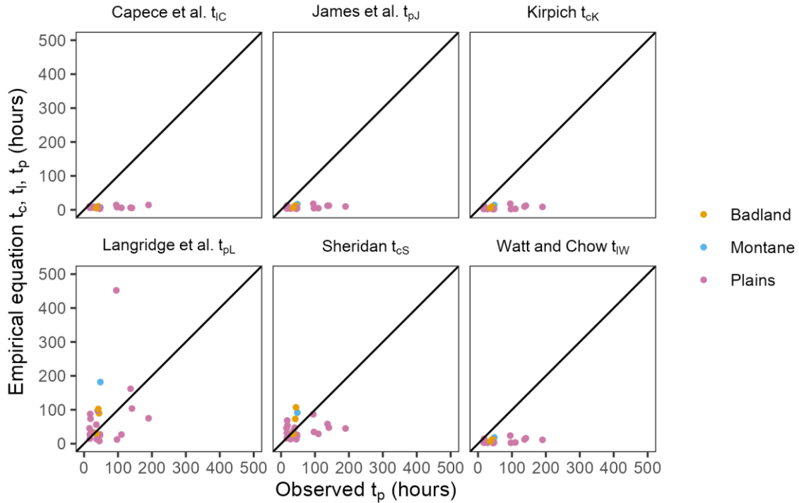
Figure 6: Empirical equation t_l , t_c and t_p vs. observed t_p for the study basins. The points are coloured according to the basin topographic type. The lines are 1:1.
