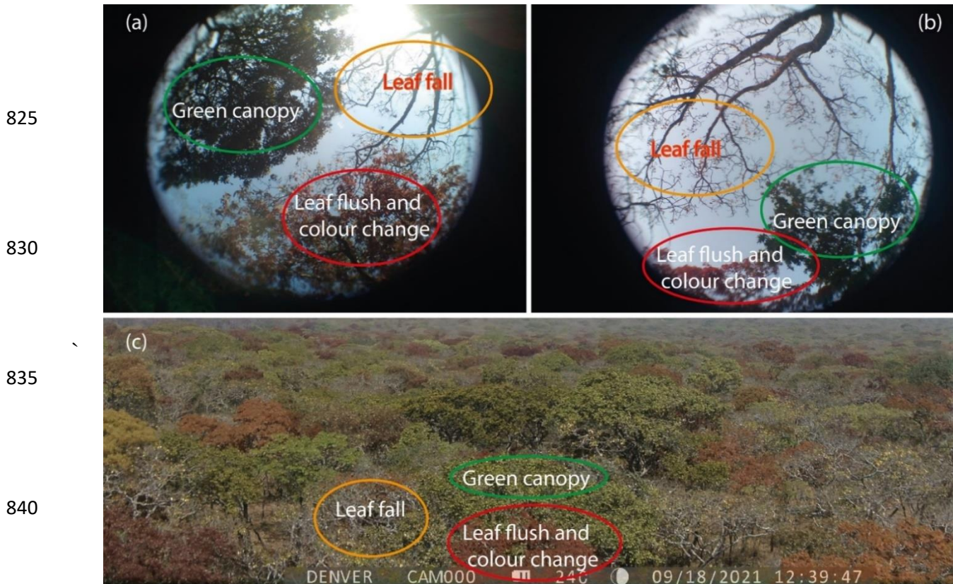
Figure 9: Heterogeneity in leaf fall and leaf flush activities among miombo woodland species: 845 observed from under the canopy (a, b) and as observed above the canopy (c). Images taken at the wet miombo woodland site in Mpika, Zambia. Images taken on 18 September, 2021.
