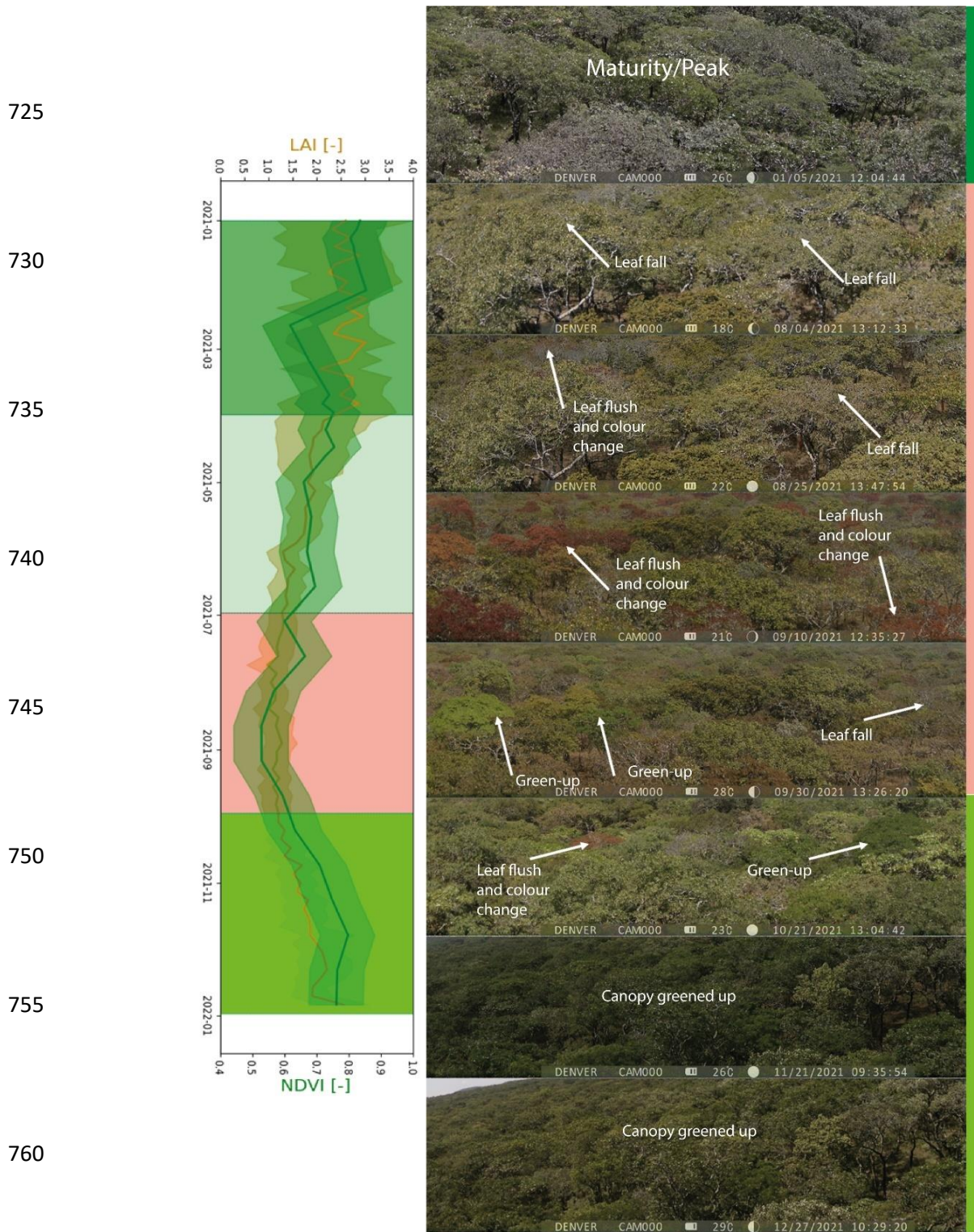
Figure 7: Temporal trend of MODIS LAI , NDVI , and the wet miombo woodland canopy display trend for the year 2021 at Mpika study site. Shaded area are phenophases: January – March is the Maturity/Peak; April-June is the Senescence/Green-down; July-September is the Dormant while October – December is the green-up. Shaded area for variables is the minimum and maximum.
