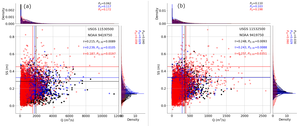
Figure S4. Epistemic uncertainty caused by the inappropriate NOAA gauge locations. The uncertainty is identified by model-data comparison at the river basins corresponding to USGS gauge 11530500 and 11532500.
