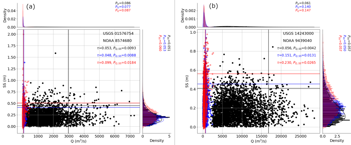
Figure S3. Epistemic uncertainty caused by the inappropriate USGS gauge locations. The uncertainty is identified by model-data comparison at the river basins corresponding to USGS gauge 01576754 and 14243000.
