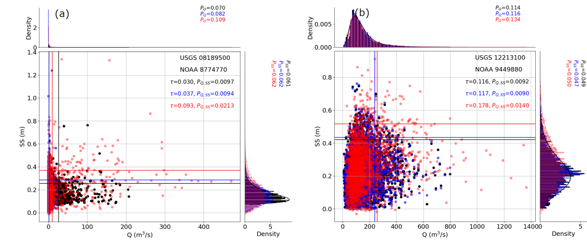
Figure S6. Epistemic uncertainty due to the underestimation of SS peaks in GTSM. The uncertainty is identified by model-data comparison at the river basins corresponding to USGS gauge 08189500 and 12213100.
