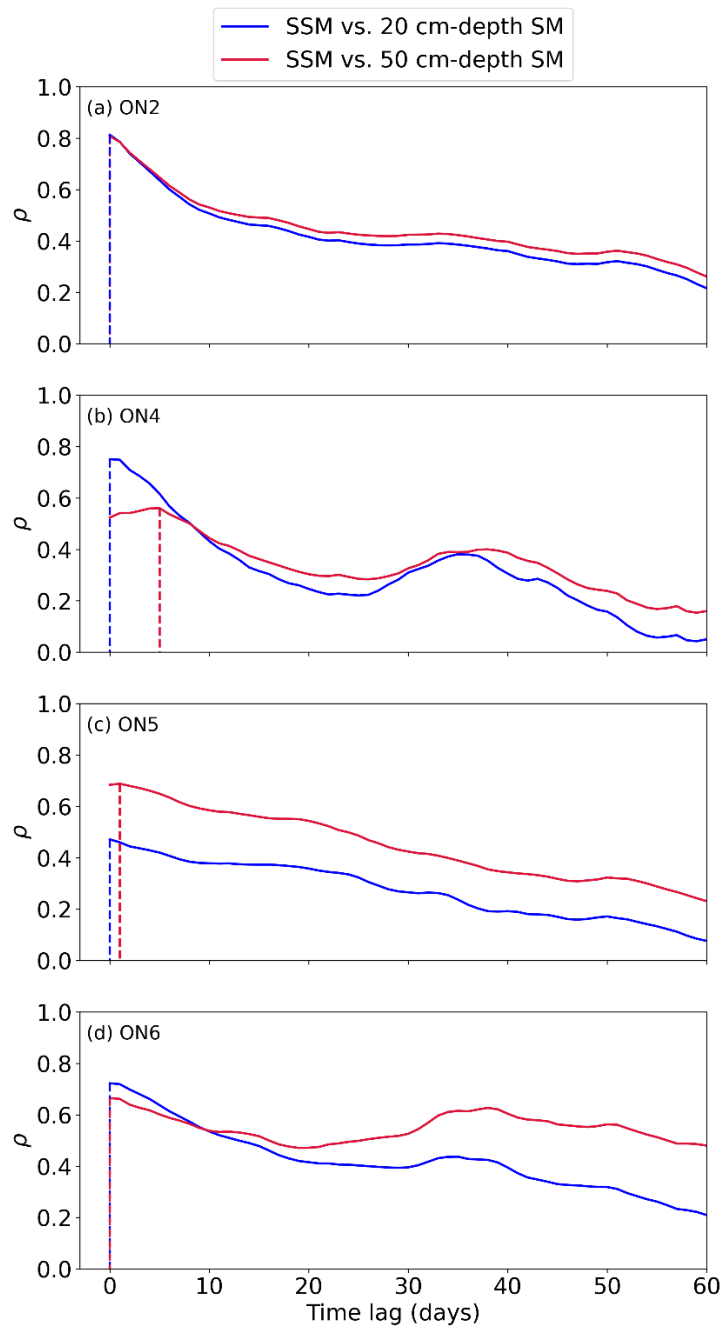
905 Figure A12: Spearman's rank correlation ( \rho ) between the near-surface (top 5 cm) soil moisture (SSM) and the subsurface (20 cm and 50 cm depths) soil moisture (SM) for the time lag ranging from 0 to 60 days based upon the in situ measurements at the four RISMA stations: (a) ON2, (b) ON4, (c) ON5, and (d) ON6, respectively. Positive lags indicate that the SSM leads the subsurface SM. The vertical dashed line indicates the optimal time lag corresponding to the maximum \rho between the SSM and subsurface SM.
