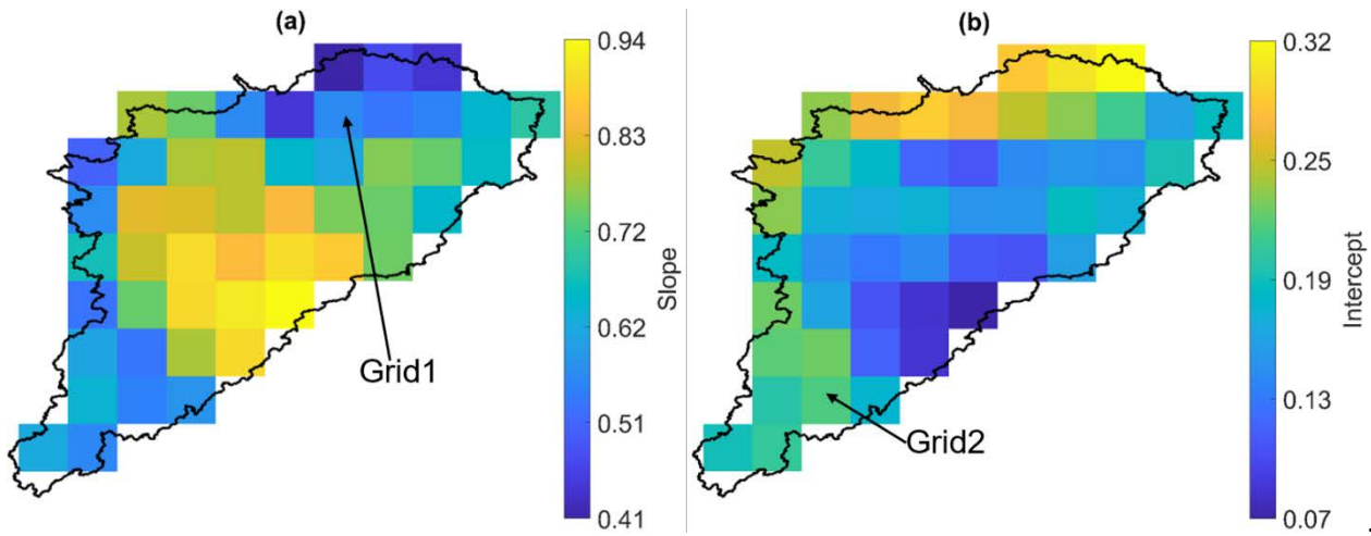
870 Figures A5: (a) Slope and (b) intercept for a linear regression between SMAP SSM (independent variable) versus HGS SSM (dependent variable) across all SMAP grids.
