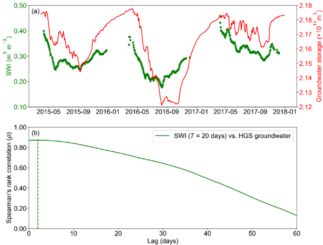
430 Figure 10: (a) Daily spaced time series of watershed-scale SWI (using T=20 days) and HGS simulated watershed integrated GW storage. (b) Spearman's rank correlations between the two time series in (a) for time lag ranging from 0 to 60 days. Positive lags indicate that the SWI leads the GW. In (b), the vertical dashed line indicates the location of the time lag leading to the maximum Spearman's rank correlation between the two series.
