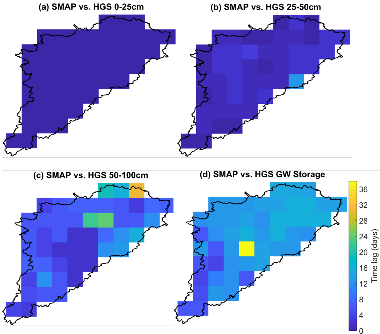
Figures A7: Optimal time lag (in days), relative to the SMAP SSM variability, for HGS simulated (a) 0–25 cm SM, (b) 25–50 cm SM, (c) 50–100 cm SM, and (d) GW storage across all SMAP grids.
