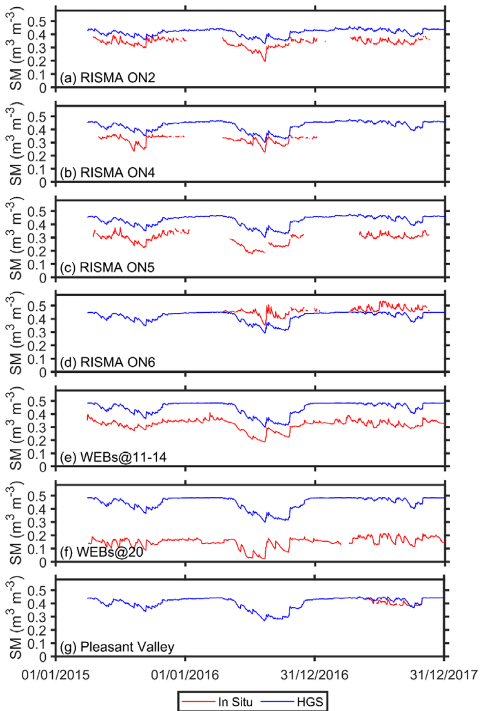
855 Figure A2. The 0-100 cm depth soil moisture time series of HGS versus In Situ at (a) ON2, (b) ON4, (c) ON5, (d) ON6, (e) WEBs@11-14, (f) WEBs@20, and (g) Pleasant Valley, respectively.
