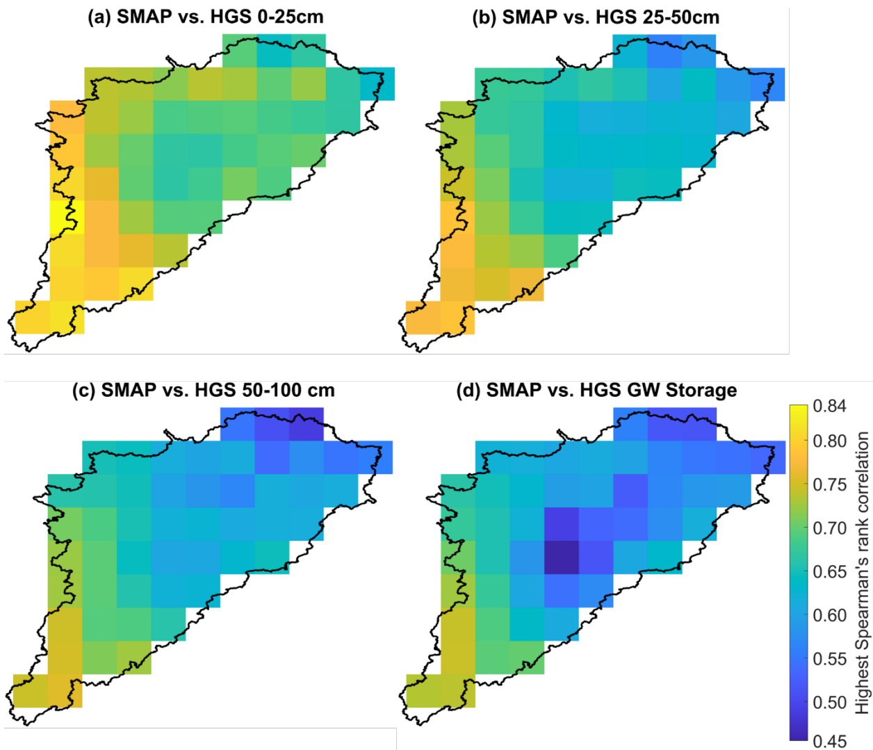
Figures A8: Maximum Spearman's rank correlation between SMAP SSM versus HGS simulated (a) 0–25 cm SM, (b) 25–50 cm SM, (c) 50–100 cm SM, and (d) GW storage, respectively, across all SMAP grids.
