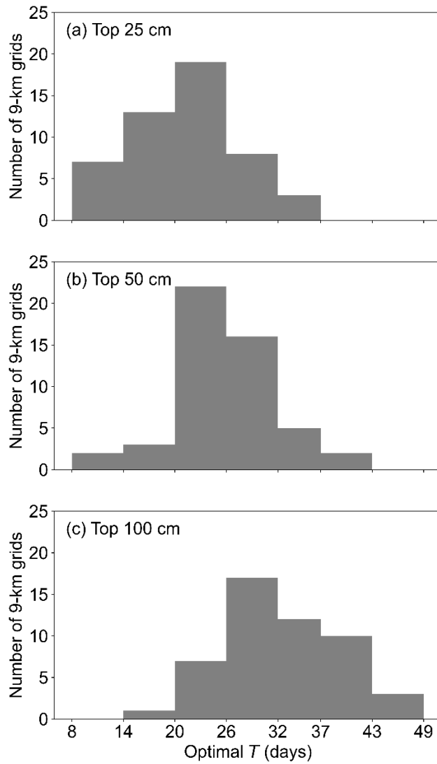
925 Figure A11: Distribution of the optimal T_{opt} at the 9-km grid scale for (a) 0–25 cm, (b) 0–50 cm, and (c) 0–100 cm soil depths, respectively.
