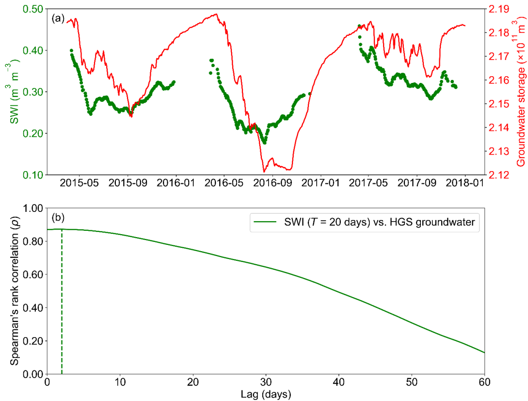
Figure 10: (a) Daily spaced time series of watershed-scale SWI (using T=20 days) and HGS simulated watershed integrated GW storage. (b) Spearman's rank correlations between the two time series in (a) for time lag ranging from 0 to 60 days. Positive lags indicate that the SWI leads the GW. In (b), the vertical dashed line indicates the location of the time lag leading to the maximum Spearman's rank correlation between the two series.
