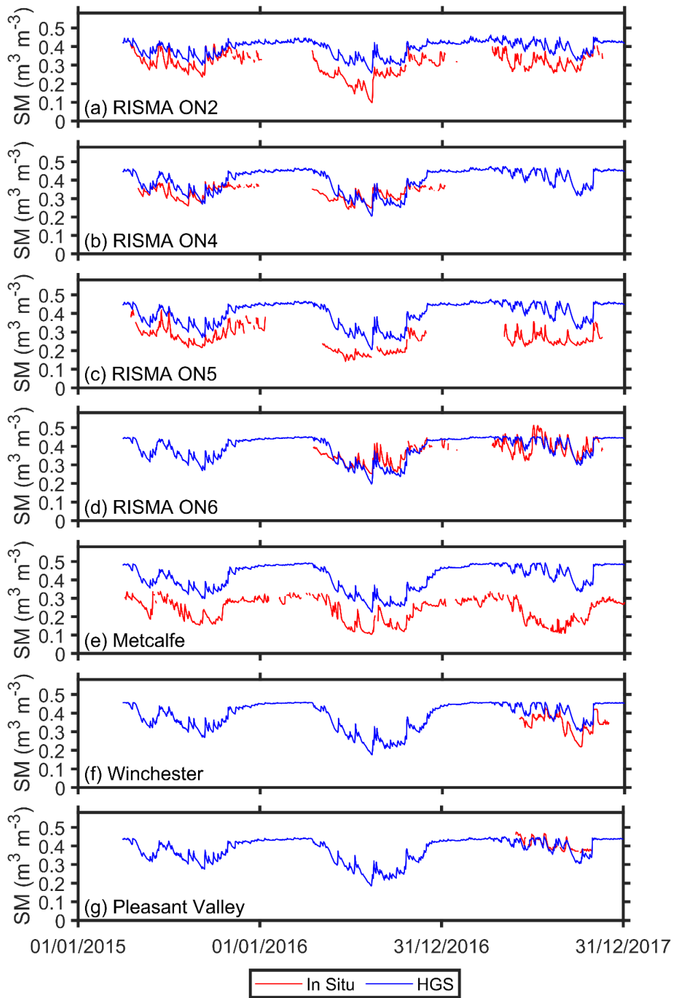
880 Figure A1: The 0-25 cm depth soil moisture time series of HGS versus In Situ at (a) ON2, (b) ON4, (c) ON5, (d) ON6, (e) Metcalfe, (f) Winchester, and (g) Pleasant Valley, respectively.
