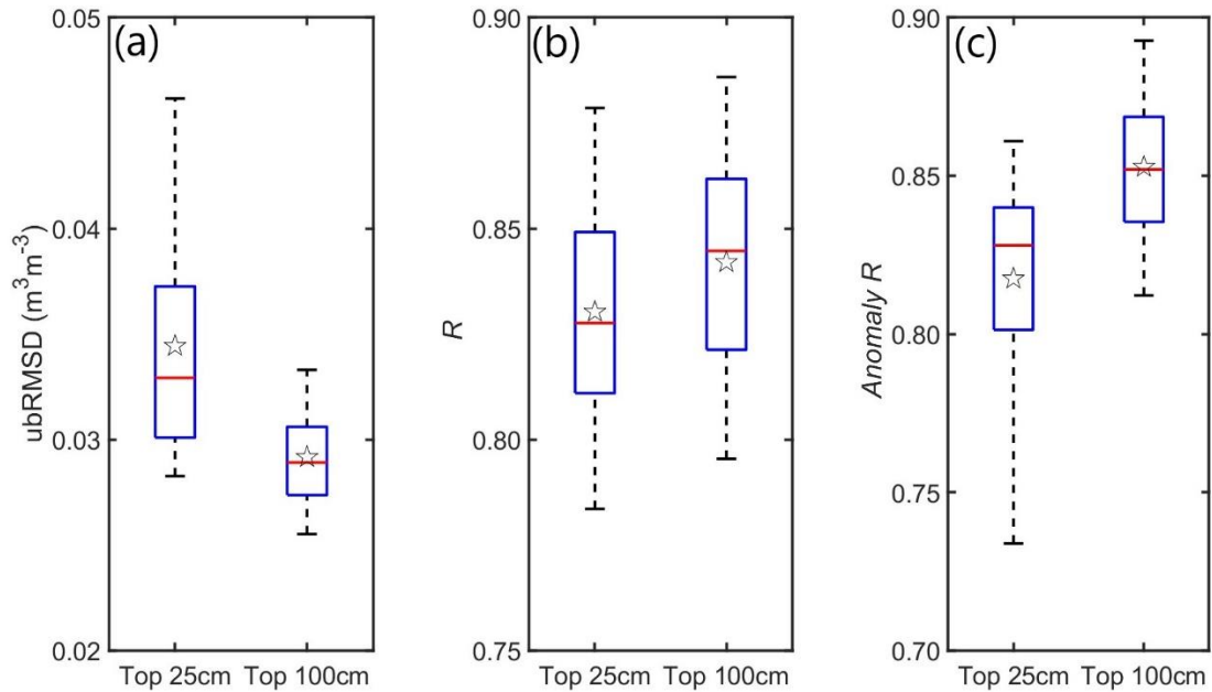
410 Figure 8: (a) Boxplots for the ubRMSD between the SMAP SSM-derived SWI (using T = 15 days) and HGS simulated top 25 cm SM and the ubRMSD between the SMAP SSM-derived SWI (using T = 20 days) and HGS simulated top 100 cm SM, respectively, summarized from all SMAP 9-km grids over the study watershed. Within each box, the horizontal segment and the star denote the median and mean of the sample data, respectively; the lower and upper edges of the box indicate the 25th and 75th percentiles, respectively; and the bottom and top ends of the whiskers denote the 5th and 95th percentiles, respectively. (b) and (c): Similar to (a), but for the correlation coefficient R and anomaly R , respectively.
