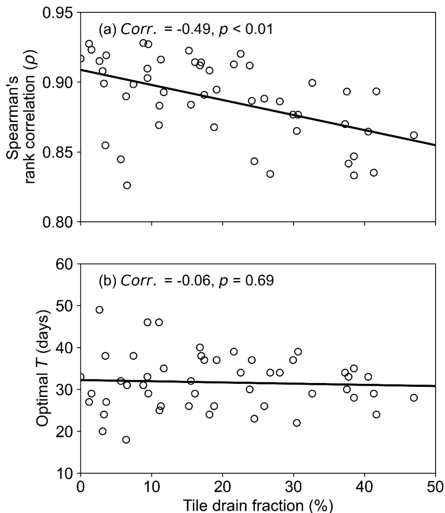
615 Figure 13: Scatterplot of the percent area of tile drains versus (a) the highest Spearman's rank correlation between the SWI series and HGS 0–100 cm SM (as shown in Fig. A10f) and (b) the identified optimal T_{opt} value for the root zone layer (as shown in Fig. A10e) across all SMAP grids. In each plot, the Pearson correlation between the two variables with p -value are provided.
