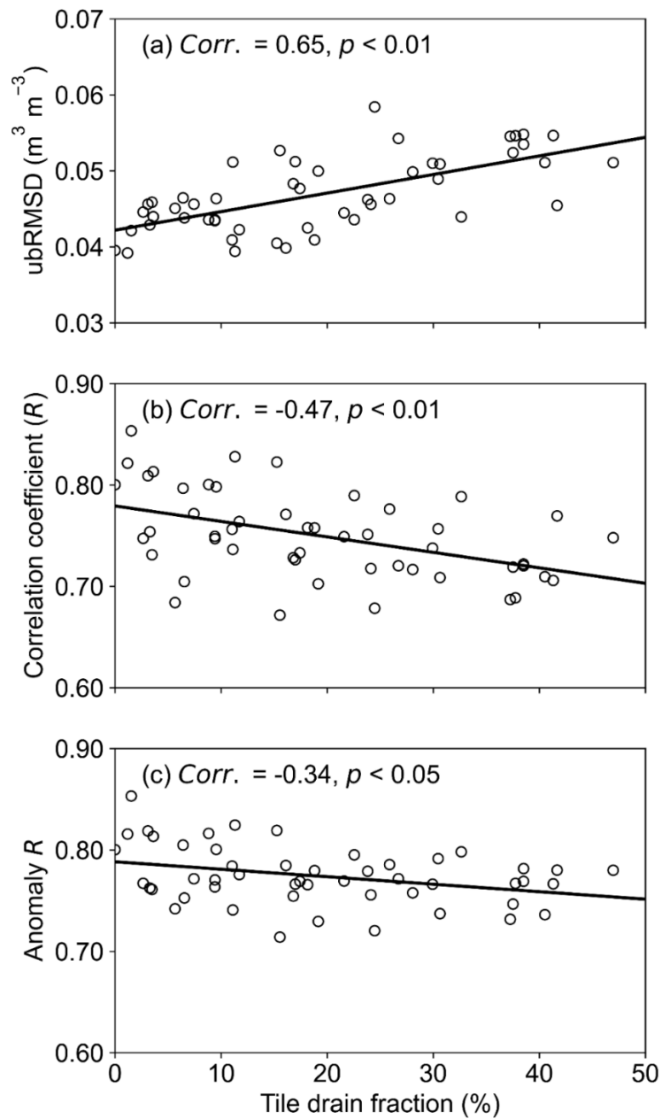
610 Figure 12: Scatterplot of the percent area of tile drains versus (a) ubRMSD, (b) R , and (c) anomaly R , respectively, across all SMAP grids within the SNW. The calculated performance metrics (shown in Fig. 3) were for HGS simulated SSM vs SMAP SSM. The Pearson correlation between tile drain fraction and each performance metric with p -value are provided in each plot.
