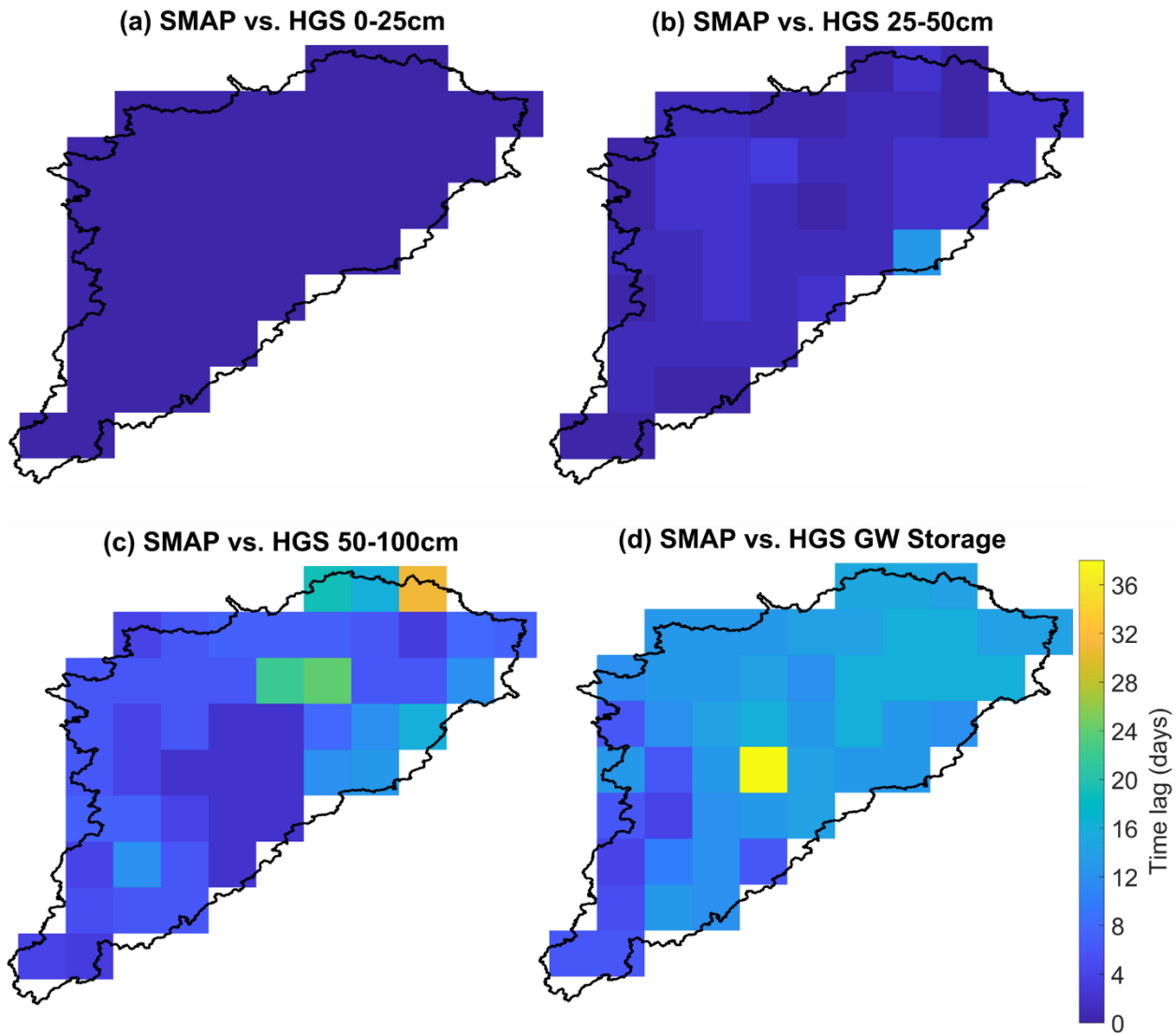
905 Figures A7: Optimal time lag (in days), relative to the SMAP SSM variability, for HGS simulated (a) 0–25 cm SM, (b) 25–50 cm SM, (c) 50–100 cm SM, and (d) GW storage across all SMAP grids.
