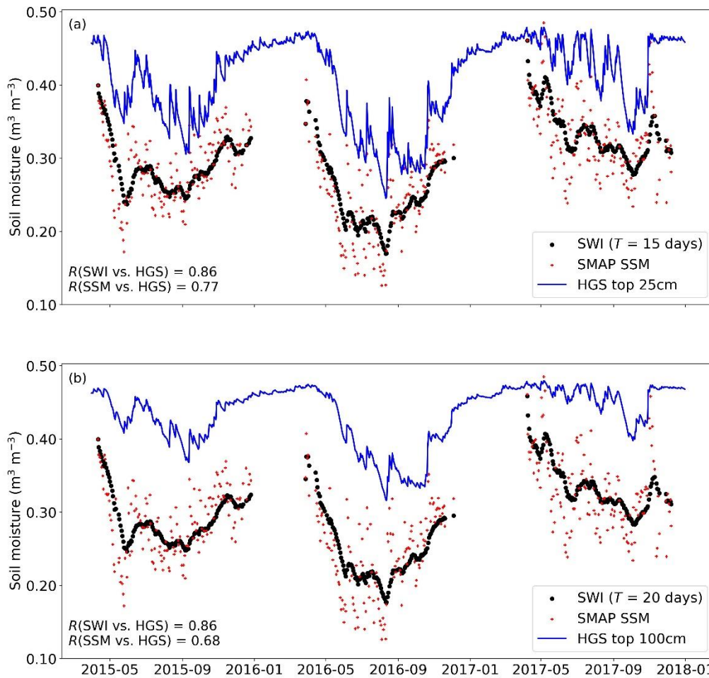
Figure 9: (a) Watershed-scale time series of SMAP SSM, SMAP SSM-derived SWI (using T=15 days), and HGS simulated top 25 cm SM. (b) Watershed-scale time series of SMAP SSM, SMAP SSM-derived SWI (using T=20 days), and HGS simulated top 100 cm SM. In each plot, the correlation R between SWI (or SMAP SSM) and simulated SM is provided.
