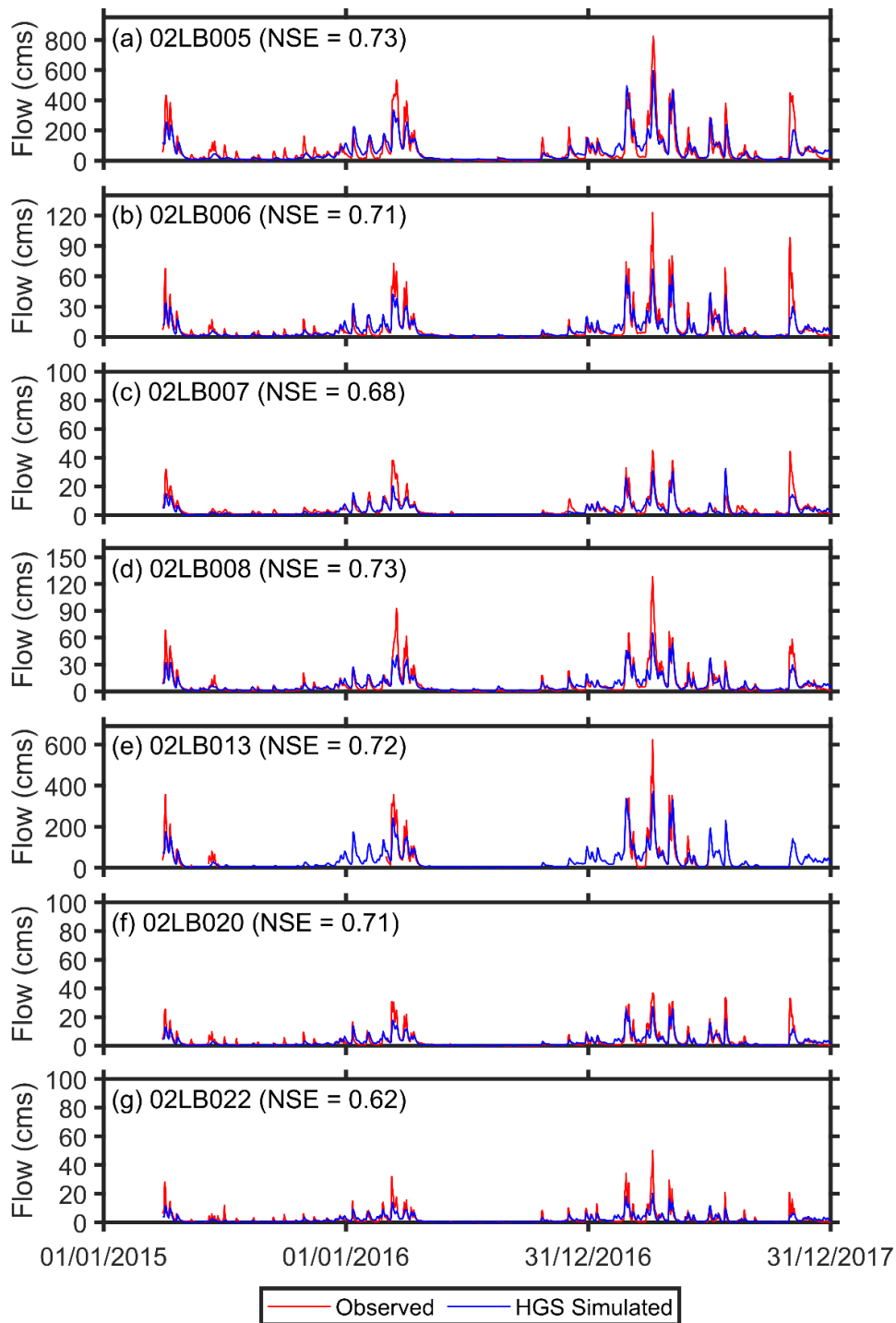
885 Figure A3: Comparison between the observed and HGS simulated hydrographs at the seven gauges: (a) 02LB005, (b) 02LB006, (c) 02LB007, (d) 02LB008, (e) 02LB013, (f) 02LB020, and (g) 02LB022, respectively. The corresponding Nash-Sutcliffe efficiency (NSE) value is provided in each panel.
