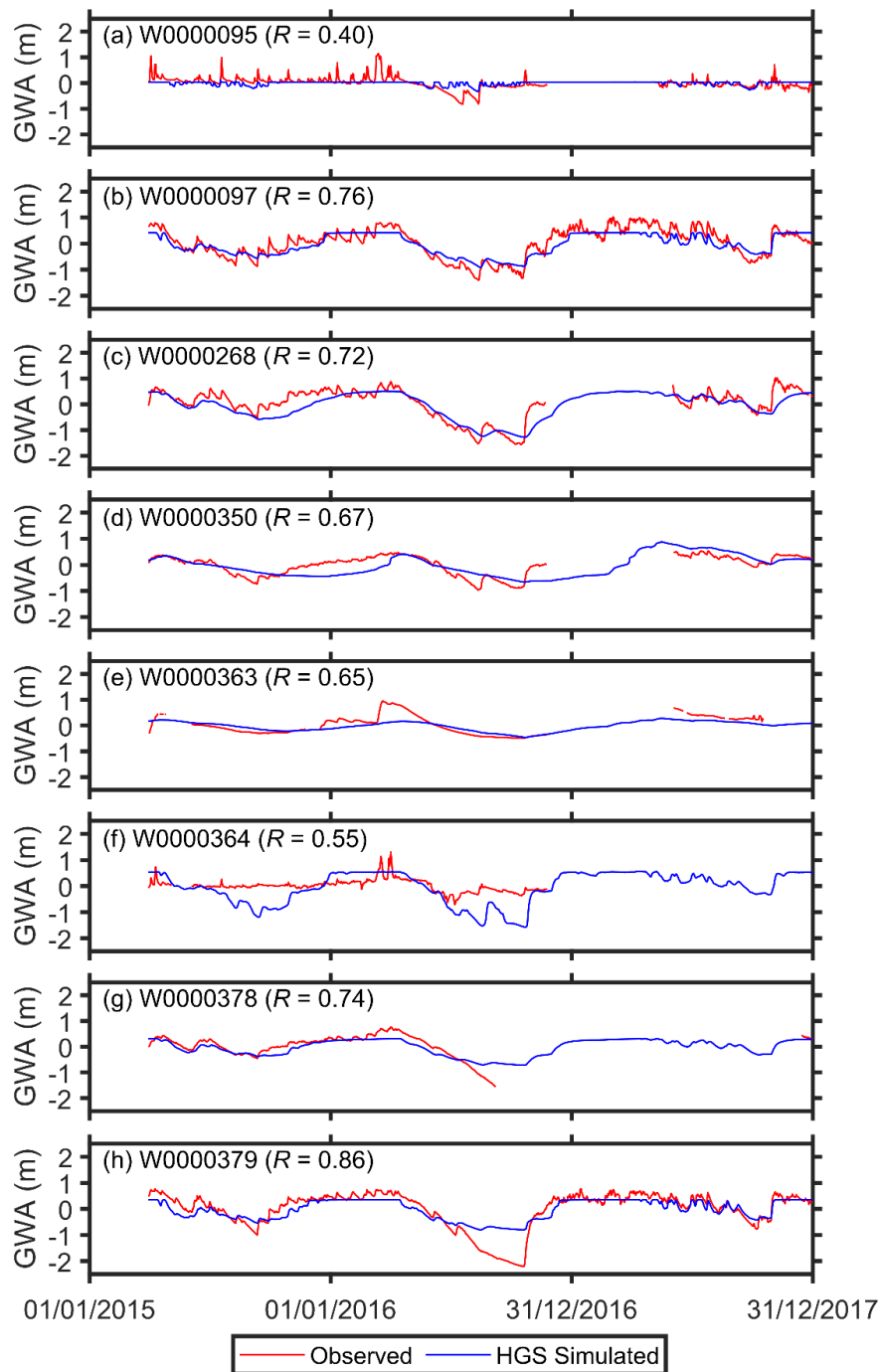
870 Figure A4: Comparison between the observed and HGS simulated groundwater level anomalies (GWA) at the eight GW monitoring wells. The anomalies represent the deviations relative to their respective means over the study period. The corresponding R value is provided in each panel.
