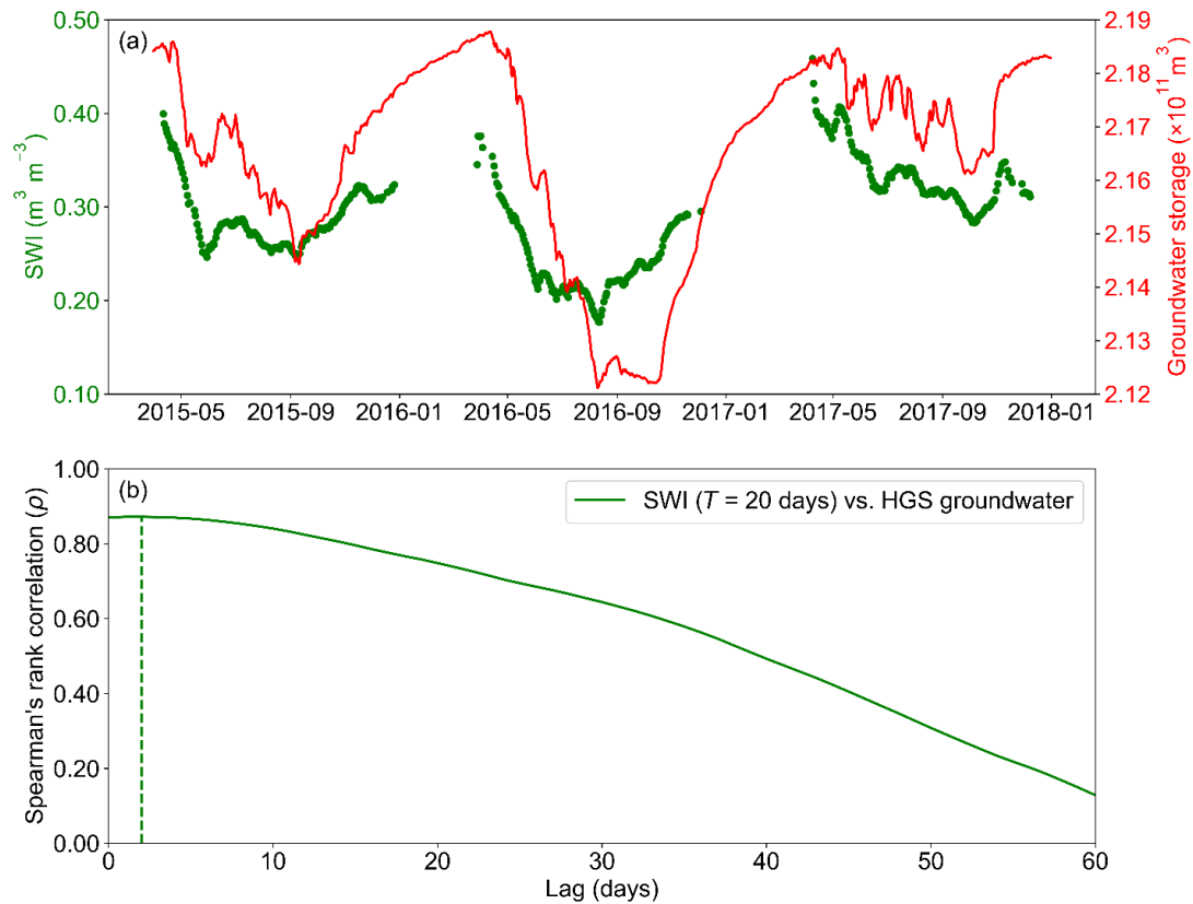
435 Figure 10: (a) Daily spaced time series of watershed-scale SWI (using T=20 days) and HGS simulated watershed integrated GW storage. (b) Spearman's rank correlations between the two time series in (a) for time lag ranging from 0 to 60 days. Positive lags indicate that the SWI leads the GW. In (b), the vertical dashed line indicates the location of the time lag leading to the maximum Spearman's rank correlation between the two series.
