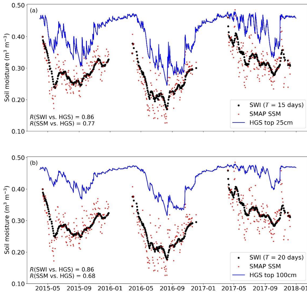
425 Figure 9: (a) Watershed-scale time series of SMAP SSM, SMAP SSM-derived SWI (using T=15 days), and HGS simulated top 25 cm SM. (b) Watershed-scale time series of SMAP SSM, SMAP SSM-derived SWI (using T=20 days), and HGS simulated top 100 cm SM. In each plot, the correlation R between SWI (or SMAP SSM) and simulated SM is provided.
