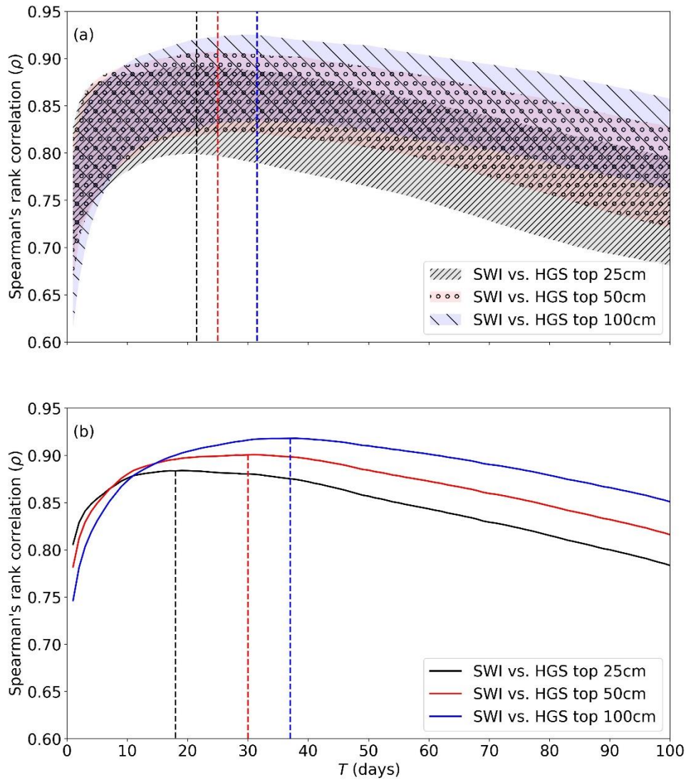
Figure 11: (a) Spearman's rank correlations coefficients between the time series (9-km grid scale) of HGS simulated SM (from the 0–25 cm, 0–50 cm, and 0–100 cm layers, respectively) and SMAP SSM-derived SWI for the characteristic time length T ranging from 1 to 100 days. For each layer, the shaded band represents the 5th to 95th percentiles of the results from all SMAP grids within the study watershed with a vertical dashed line indicating the location of the optimal T_{opt} median from all SMAP grids. (b) Spearman's rank correlation coefficients between the time series (watershed scale) of HGS simulated SM (from the 0–25 cm, 0–50 cm, and 0–100 cm layers, respectively) and SMAP SSM-derived SWI for T ranging from 1 to 100 days. For each layer, the vertical dashed line indicates the location of T_{opt} at the watershed scale.
