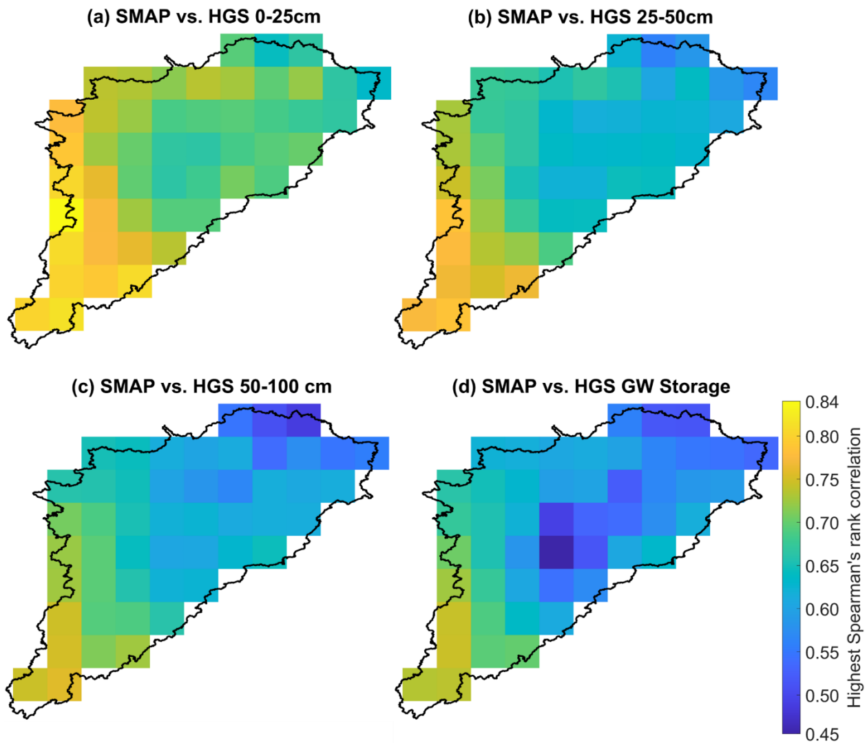
890 Figures A8: Maximum Spearman's rank correlation between SMAP SSM versus HGS simulated (a) 0–25 cm SM, (b) 25–50 cm SM, (c) 50–100 cm SM, and (d) GW storage, respectively, across all SMAP grids.
