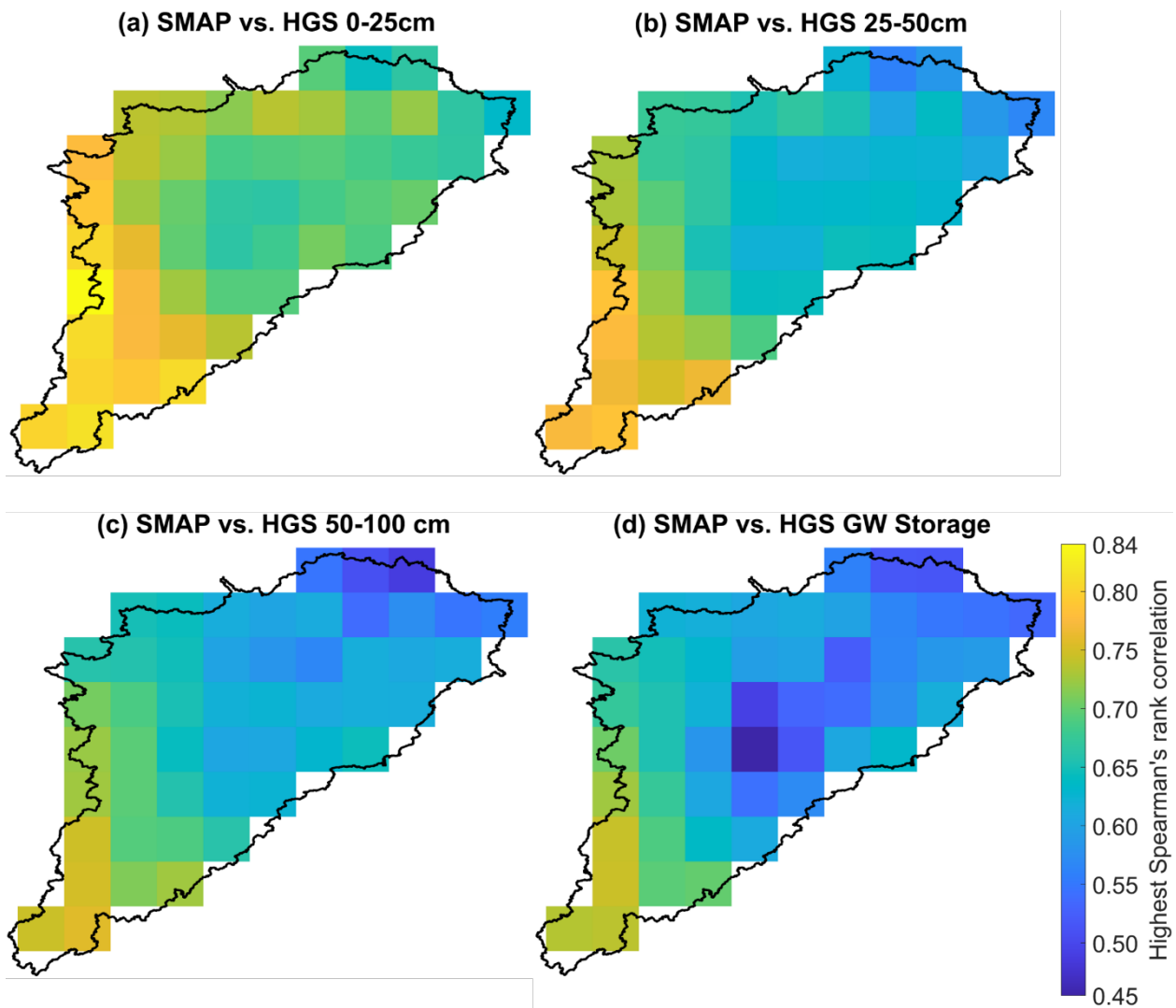
885 Figures A8: Maximum Spearman's rank correlation between SMAP SSM versus HGS simulated (a) 0–25 cm SM, (b) 25–50 cm SM, (c) 50–100 cm SM, and (d) GW storage, respectively, across all SMAP grids.
