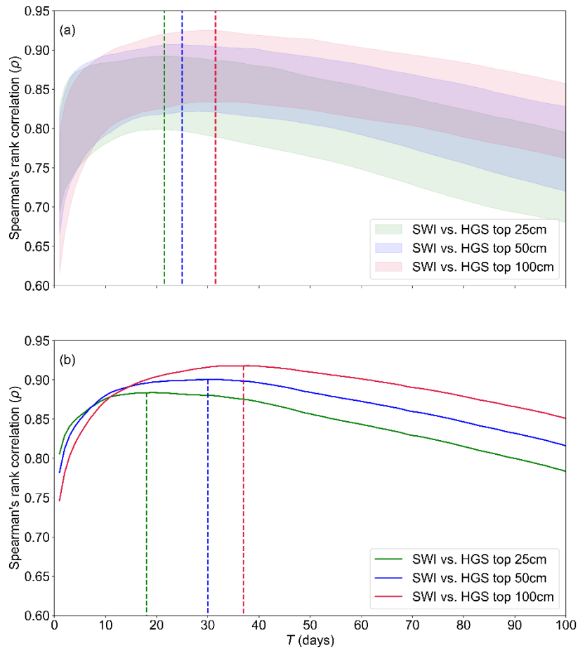
465 Figure 11: (a) Spearman's rank correlations coefficients between the time series (9-km grid scale) of HGS simulated SM (from the 0–25 cm, 0–50 cm, and 0–100 cm layers, respectively) and SMAP SSM-derived SWI for the characteristic time length T ranging from 1 to 100 days. For each layer, the shaded band represents the 5th to 95th percentiles of the results from all SMAP grids within the study watershed with a vertical dashed line indicating the location of the optimal T_{opt} median from all SMAP grids. (b) Spearman's rank correlation coefficients between the time series (watershed scale) of HGS simulated SM (from the 0–25 cm, 0–50 cm, and 0–100 cm layers, respectively) and SMAP SSM-derived SWI for T ranging from 1 to 100 days. For each layer, the vertical dashed line indicates the location of T_{opt} at the watershed scale.
