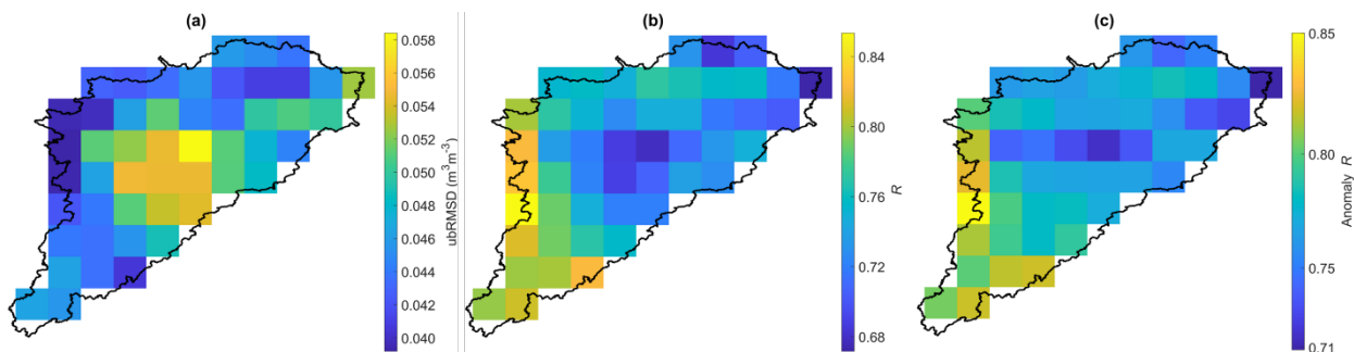
280 Figure 3: (a) ubRMSD, (b) R , and (c) anomaly R between the SMAP SSM and HGS SSM across all SMAP grids.
