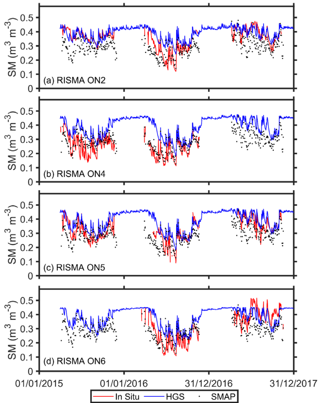
245 Figure 2: The SSM time series from SMAP, HGS model simulation, and in situ measurements, respectively, at the four RISMA stations: (a) ON2, (b) ON4, (c) ON5, and (d) ON6.
