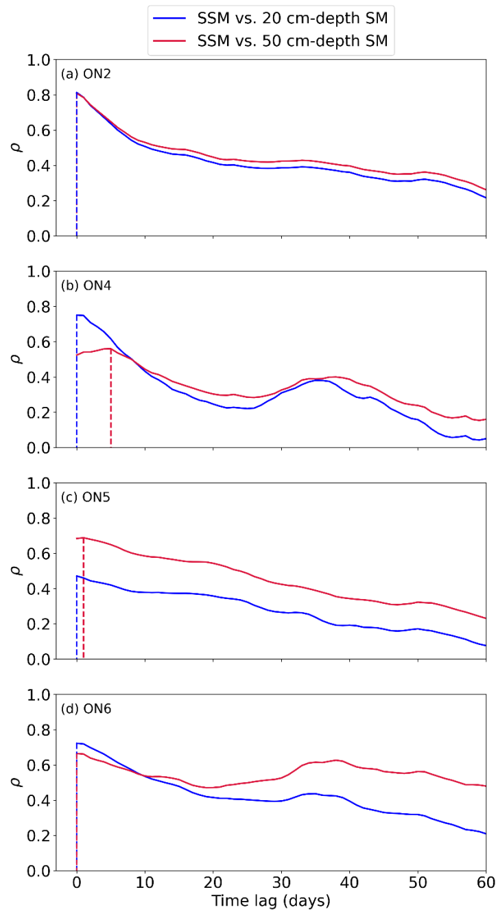
Figure A12: Spearman's rank correlation ( \rho ) between the near-surface (top 5 cm) soil moisture (SSM) and the subsurface (20 cm and 50 cm depths) soil moisture (SM) for the time lag ranging from 0 to 60 days based upon the in situ measurements at the four RISMA stations: (a) ON2, (b) ON4, (c) ON5, and (d) ON6, respectively. Positive lags indicate that the SSM leads the subsurface SM. The vertical dashed line indicates the optimal time lag corresponding to the maximum \rho between the SSM and subsurface SM.
