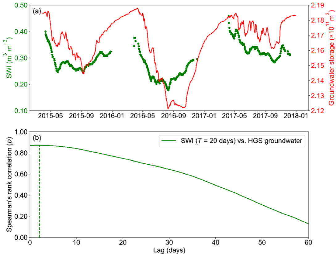
430 Figure 10: (a) Daily spaced time series of watershed-scale SWI (using T=20 days) and HGS simulated watershed integrated GW storage. (b) Spearman's rank correlations between the two time series in (a) for time lag ranging from 0 to 60 days. Positive lags indicate that the SWI leads the GW. In (b), the vertical dashed line indicates the location of the time lag leading to the maximum Spearman's rank correlation between the two series.
