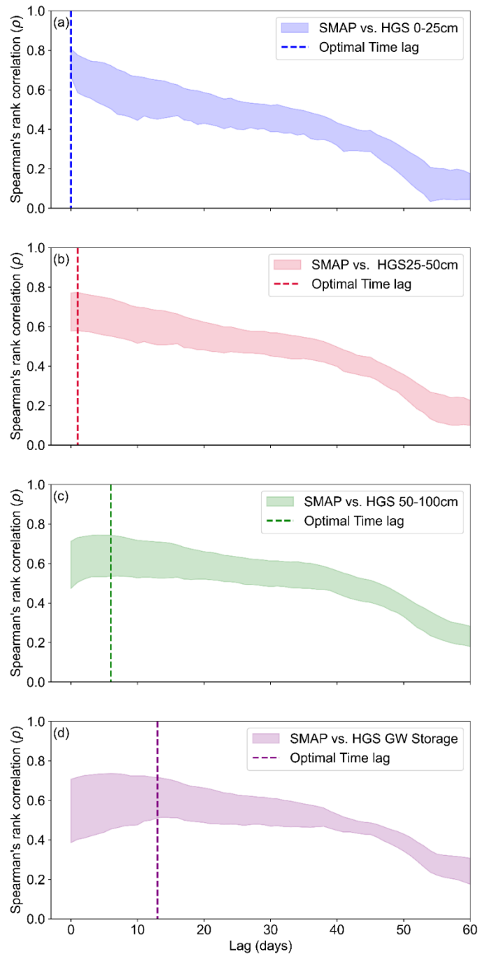
310 Figure 5: Spearman's rank correlation coefficients between the time series of SMAP SSM and HGS simulated SM from (a) 0–25 cm 315 depth, (b) 25–50 cm depth, and (c) 50–100 cm depth, respectively, as well as (d) GW storage for time lags ranging from 0 to 60 days. Positive lags indicate that the SMAP data are leading the HGS simulations. In each plot, the shaded band represents the 5th to 95th percentiles of the results from all SMAP grids within the study watershed. For each SMAP grid, the optimal time lag is defined as the one with the maximum Spearman's rank correlation between SMAP SSM and HGS simulated variable. The vertical dashed line indicates the median of the optimal time lags from all SMAP grids.
