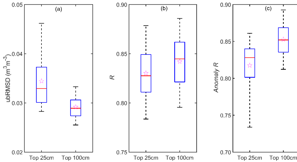
410 Figure 8: (a) Boxplots for the ubRMSD between the SMAP SSM-derived SWI (using T = 15 days) and HGS simulated top 25 cm SM and the ubRMSD between the SMAP SSM-derived SWI (using T = 20 days) and HGS simulated top 100 cm SM, respectively, summarized from all SMAP 9-km grids over the study watershed. In each box, the red line and the star denote the median and mean of the sample data, respectively; the lower and upper edges of the box indicate the 25th and 75th percentiles, respectively; and the bottom and top ends of the whiskers denote the 5th and 95th percentiles, respectively. (b) and (c): Similar to (a), but for the correlation coefficient R and anomaly R , respectively.
