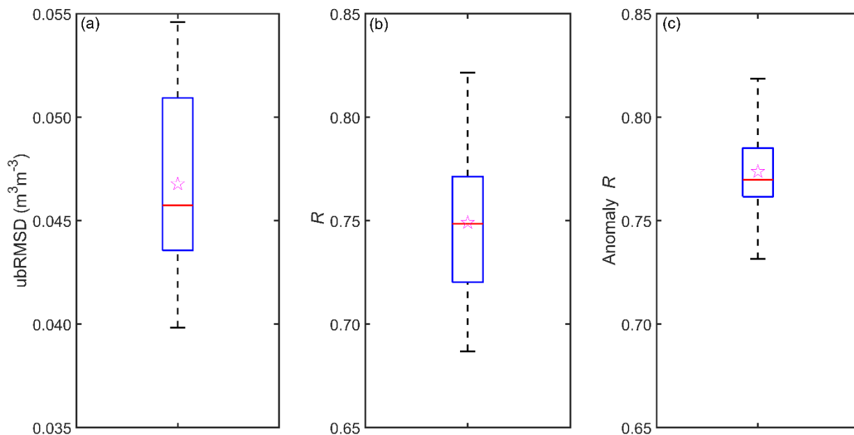
285 Figure 4: Boxplots of (a) ubRMSD, (b) R , and (c) anomaly R between the SMAP SSM and HGS SSM, summarized from all 9-km grids within the study watershed. In each box, the red line and the star denote the median and mean of the sample data, respectively; the lower and upper edges of the box indicate the 25th and 75th percentiles, respectively; and the bottom and top ends of the whiskers denote the 5th and 95th percentiles, respectively.
