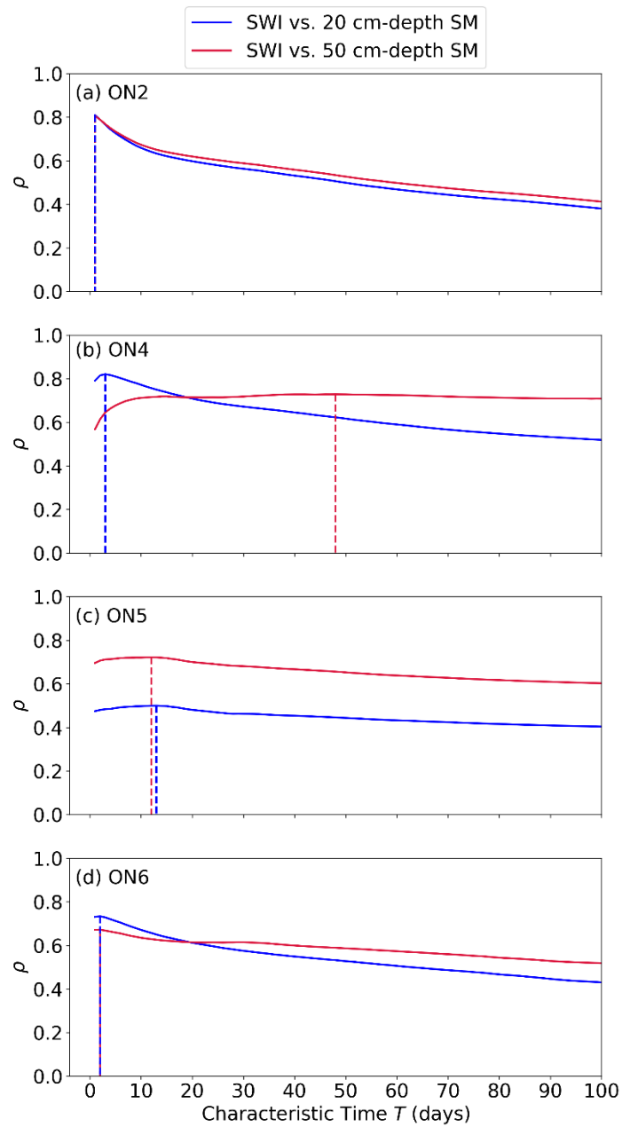
910 Figure A13: Spearman's rank correlation ( \rho ) between the subsurface SM (20 cm and 50 cm depths) and the SSM-derived SWI for the characteristic time T ranging from 1 to 100 days, based upon the in situ measurements at the four RISMA stations: (a) ON2, (b) ON4, (c) ON5, and (d) ON6, respectively. The vertical dashed line indicates the location of the optimal characteristic time T_{opt} for SWI estimation.
