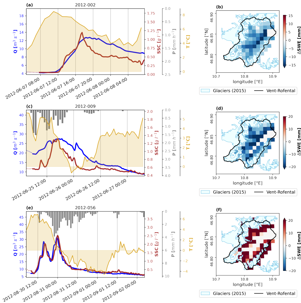
Figure 12. Examples of freeze-thaw modulated events (type 2 events). See explanation Fig. 10. Event 2012-002 (a) is an example of an early season, smaller magnitude snow-melt event where the lower elevations contributed most (b). Event 2012-009 is a rain-on-snow event where both snow-melt (d) and rainfall (c) contributed to streamflow. Event 2012-056 is a precipitation-driven event (e), with two initial rainfall-driven pulses, and subsequent snowfall as the catchment froze (f).
