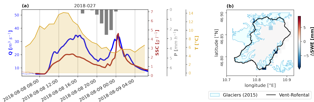
Figure 10. Example of a compound rainfall-melt extreme event (type 0event). Left-hand panels show event hydrographs of 15-min streamflow ( Q ), sedigraphs of 15 min suspended sediment concentrations (SSC), hyetographs of hourly precipitation ( P ), and hourly catchment average air temperature ( T ). Right-hand panels show changes in SNOWGRID SWE from first to last day of event. Event 2018-027 was not influenced by snow-melt (b). An initial pulse of glacier melt during the day, was followed by a rainfall-driven pulse at night (a).
