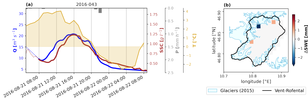
Figure 13. Example of late season glacier melt events (type 3 event). See explanation Fig. 10. Event 2016-043 is a small magnitude glacier melt event due to low and below freezing temperatures (a) and no snow-melt (b).
