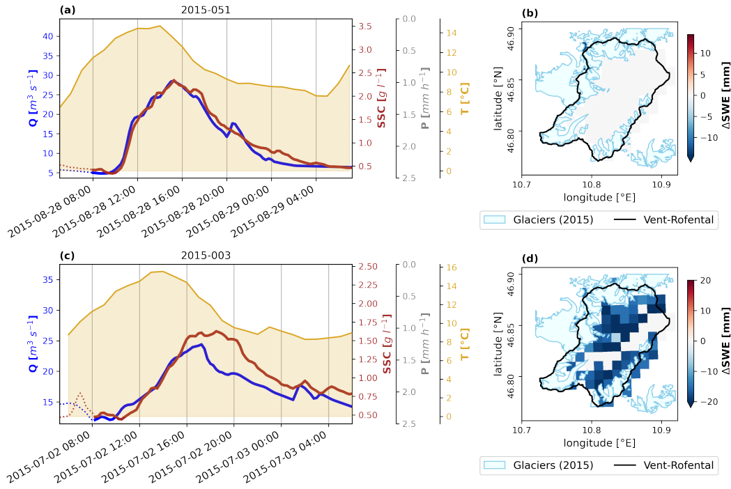
Figure 11. Examples of high melt events (type 1 events). See explanation Fig. 10. Event 2015-051 represents a glacier-melt-induced event (a), with no apparent influence of snow-melt (b). Event 2015-003 (c) is mainly snow-melt-driven (d). Note the high catchment temperatures for both events.
