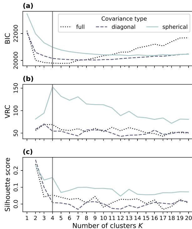
Figure 6. Selection of optimal number of clusters K and GMM covariance type based on the Bayesian Information Criterion (BIC) and the Variance Ratio Criterion (VRC), and the silhouette score (SC). Low (high) BIC (VRC, SC) indicates better defined clusters. The selected number of clusters ( K = 4 ) is indicated with a grey vertical line.
