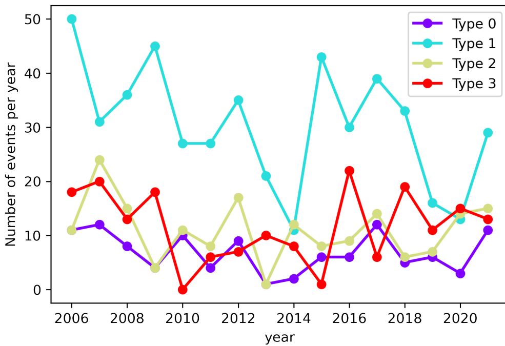
Figure 2: Event type frequency over the study period
