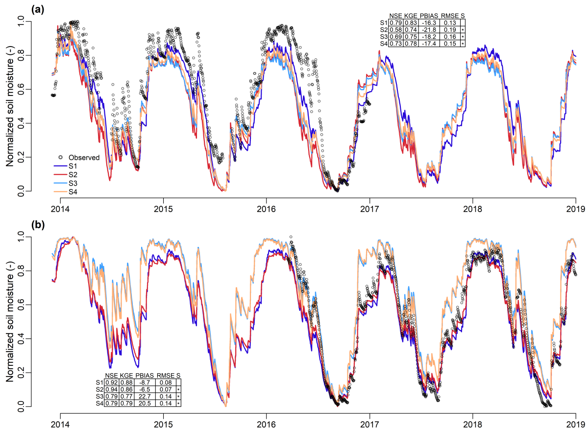
620 Figure 10. a) Normalized observed (point PG2) and simulated soil moisture in the S_{UR} reservoir and b) Normalized observed (Toullou point) and simulated soil moisture in the S_U reservoir for four calibration scenarios: S1 (Hydro Only), S2 (Hydro + DOC), S3 (Hydro + \text{NO}_3^- ) and S4 (Hydro + DOC + \text{NO}_3^- ). NSE: Nash–Sutcliffe model efficiency coefficient, KGE: Kling–Gupta efficiency, PBIAS = Percent bias, RMSE: Root-mean-square error, S: Significance level. An asterisk in the significance level column indicates values that differed significantly ( p < 625 0.05) from those for scenario S1 (two-sided Mann-Whitney test). See Table 3 for definitions of the performance metrics.
