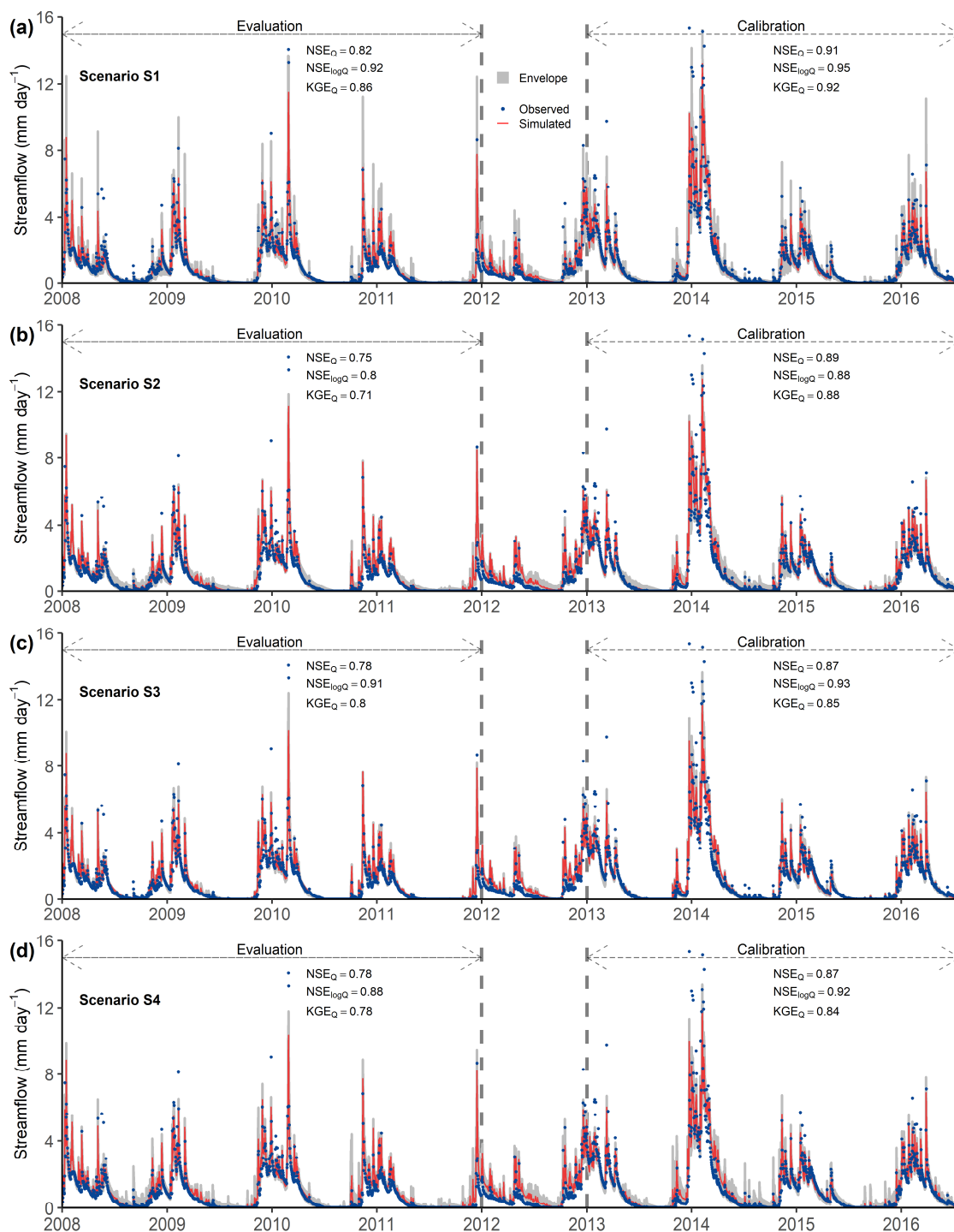
520 Figure 4. Observed and simulated flows for the calibration and evaluation periods according to the four scenarios: a) S1 (Hydro only), b) S2 (Hydro + dissolved organic carbon (DOC)), c) S3 (Hydro + nitrate ( NO_3^- )) and d) S4 (Hydro + DOC + NO_3^- ). The simulated data for each scenario correspond to the best-compromise simulated discharge of the set of optimal solutions. “Envelope” refers to the simulated discharge envelope using all parameter sets on the Pareto front. See Table 3 for definitions of model-performance metrics.
