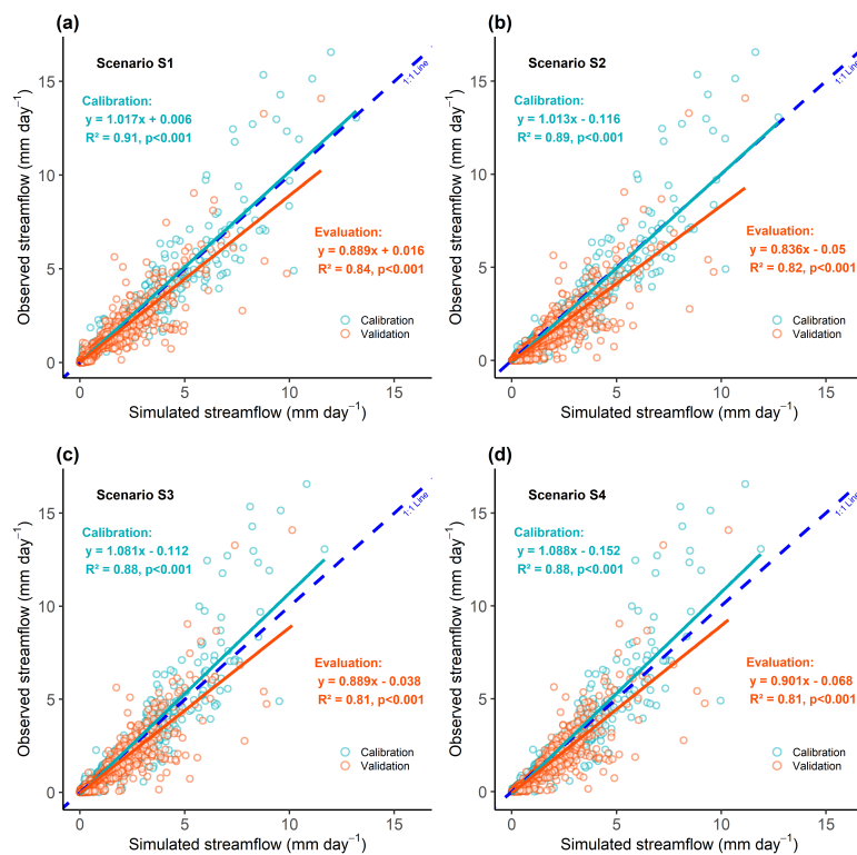
Figure A1. Relationship between observed and simulated streamflow for calibration and evaluation periods for four calibration scenarios: a) S1 (Hydro Only), b) S2 (Hydro + DOC), c) S3 (Hydro + NO 3 - ) and d) S4 (Hydro + DOC + NO 3 - ). The dashed blue line is the 1:1 line. The light green or orange lines are linear regressions for the calibration or evaluation period, respectively. All relationships were statistically significant ( p < 0.001 ).
