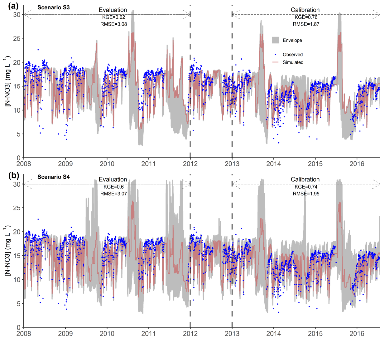
540 Figure 6. Observed and simulated nitrate ( \text{NO}_3^- ) concentrations for the calibration and evaluation periods according to two scenarios: a) S3 (Hydro + \text{NO}_3^- ) and b) S4 (Hydro + DOC + \text{NO}_3^- ). The mean ( \pm standard deviation) observed \text{NO}_3^- concentration was 13.4 \pm 2.7 and 16.6 \pm 2.8 mg N- \text{NO}_3^- \text{L}^{-1} for the calibration and evaluation period, respectively. The simulated data for each scenario correspond to the best-compromise simulated \text{NO}_3^- concentration of the set of optimal solutions. “Envelope” refers to the simulated \text{NO}_3^- concentration envelope using all parameter sets on the Pareto front. KGE: Kling–Gupta efficiency, RMSE: Root-mean-square error. See Table 3 for definitions of model-performance metrics. 545
