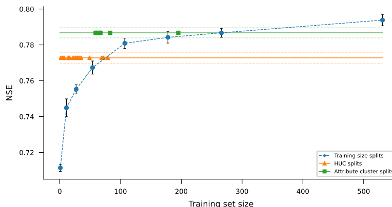
Figure 6. Median NSE scores of simulated volumetric discharge over 531 CAMELS basins for LSTM models trained and tested on splitting the 531 CAMELS basins into different sized-groupings for training and testing. All models were tested on the same basins where they were trained (during different time periods). Grouping-The blue line represents basin groupings of different sizes were-chosen randomly without replacement so that all 531 basins are-were modeled exactly once for each grouping size-split. The dots represent Orange and green lines show results from grouping the median-NSE-score-across-all-531 basins into sets based on USGS hydrological unit codes (orange), average over-the-ten-separately-trained-LSTM-models. The error bars represent standard deviation and k-means clustering of basin attributes (green). Dots on the medians-over orange and green lines indicate the ten repetitions. The ten separately-trained-LSTMs all use-sizes of the same-(18 and 6) basin groups used in those splits, so-that-variability-is-due-to-randomness-since there are a different number of CAMELS basins in each HUC and a different number of basins in each attribute cluster. Blue dots and solid orange and green lines represent the initial-weights median model performance over 531 basins, while blue error bars and biases-before-training-dashed orange and green lines represent the standard deviation of this median over a ten-member ensemble.
