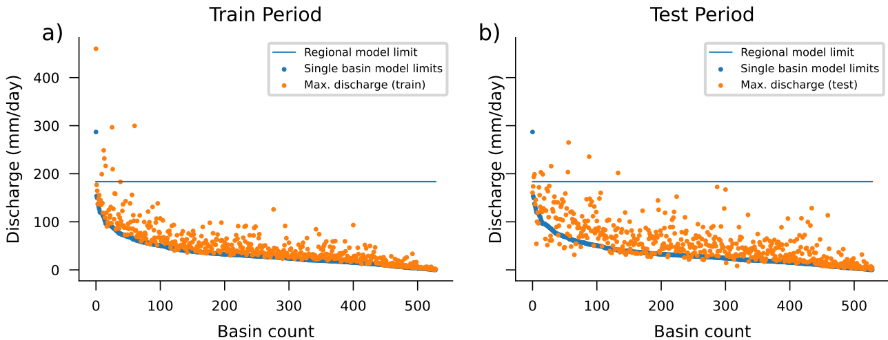
Figure 4. The theoretical maximum streamflow prediction of an LSTM model with a linear head layer when trained per basin (blue dots) and for all 531 CAMELS basins together (blue line). Orange dots represent the maximum streamflow values per basin in the train period (left subpanel a) and test period (right subpanel b). In the test period, there are 10 flow values above the maximum prediction of the regional model, while there are more than 6,346 flow values above the theoretical maximums of their respective single-basin models across all basins and all timesteps.
