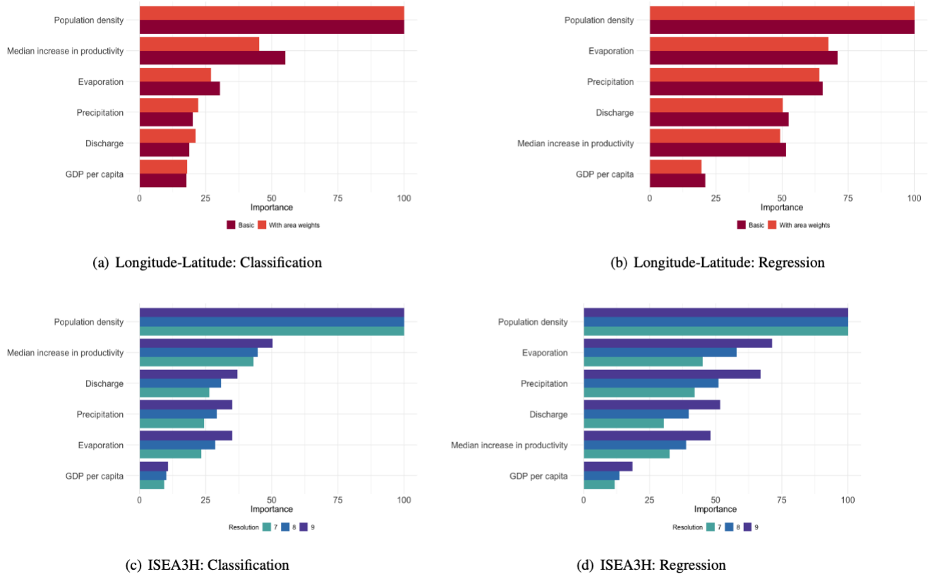
Figure 4. Relative importance, measured as decrease of node impurity. The results for the longitude-latitude grids can be seen in red and the results for the ISEA3H grids are displayed in blue. The order of variables in the importance plots are robust to 500 bootstrap steps.
